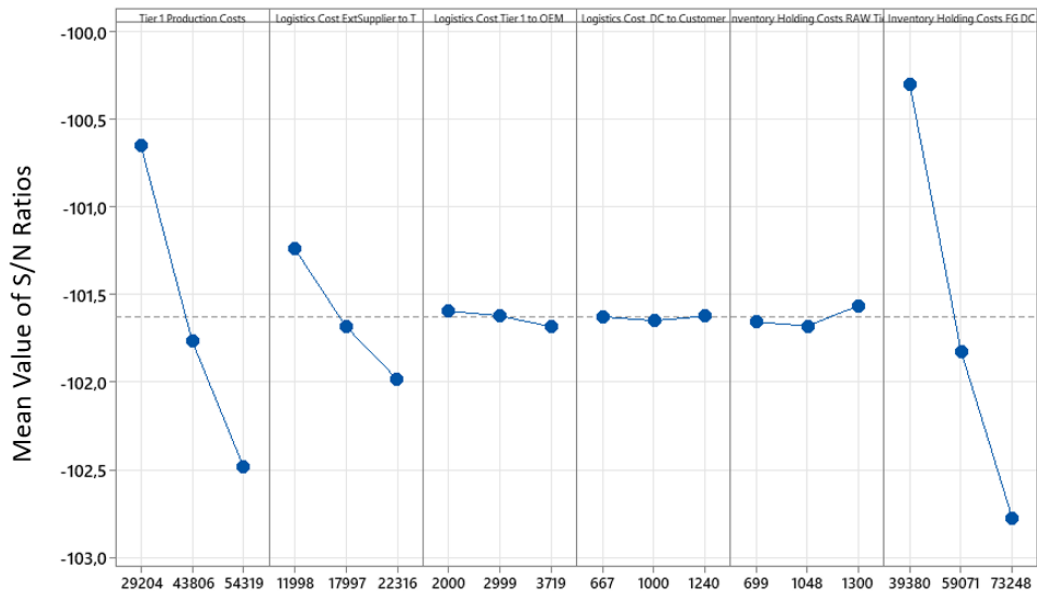
Figure 2.6: Main Plot for Signal and Noise Ratio Reduced Case
