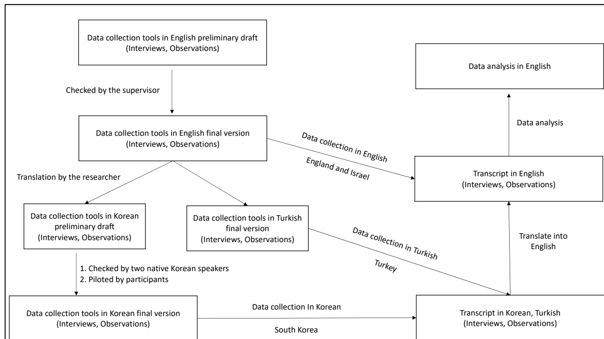
Figure 4. 3: Translation procedures
