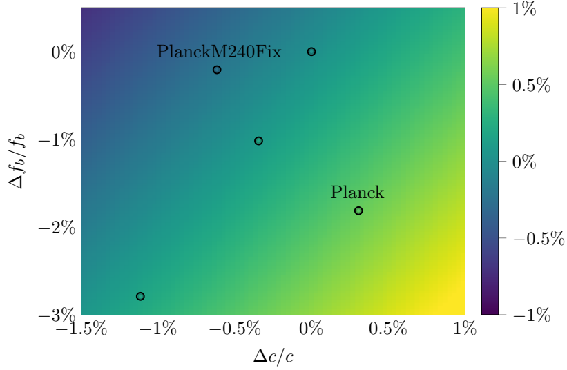
Figure 8.3: We can predict the non-factorizable correction to the power spectrum from the changes in baryon fraction and halo concentration. The points are based on the different L = 1 Gpc simulations listed in Table 8.1, shown relative to the fiducial DES3.L1000 model. We evaluate the matter power spectra at k = 10h \text{ Mpc}^{-1} , where the corrections first become important.
