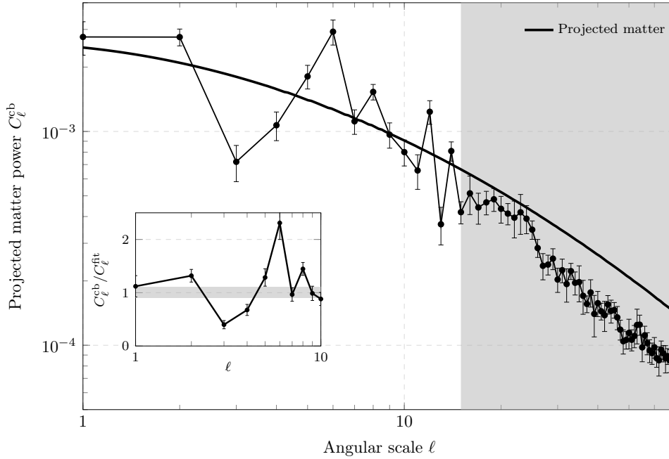
Figure 7.6: Dimensionless angular power spectrum of the projected CDM and baryon density contrast, C_\ell^{\text{cb}} , out to 200 Mpc for 0.01 eV. By construction, the results are similar for different neutrino masses. We fit a smooth spectrum, C_\ell^{\text{fit}} = \exp(c_1 + c_2 \log \ell + c_3 \log^2 \ell) , up to \ell_{\text{max}} = 15 to the simulation spectrum (thick solid curve). The inset graph zooms in on the lowest-order multipoles, showing the data relative to the fit. The grey error bar represents \pm 10\% .
