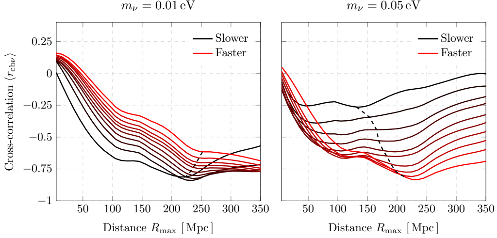
Figure 7.7: Cross-correlation coefficient, r_{cb\nu}(\ell) = C_\ell^{cb\nu}/(C_\ell^\nu C_\ell^{cb})^{1/2} , between the local neutrino density and the projected CDM and baryon density, as a function of the maximum projected distance R_{\max} , for m_\nu \in \{0.01, 0.05\} eV, split into ten equal-sized neutrino momentum bins. The coefficients are averaged over the multipoles 1 \leq \ell \leq 10 and the curves are smoothed with a Savitzky-Golay filter. The dashed line indicates the locus of the barycentre of each curve, indicating that the sensitivity shifts to larger distances for faster neutrinos. Note that the overall momentum range is much wider for the 0.01 eV case.
