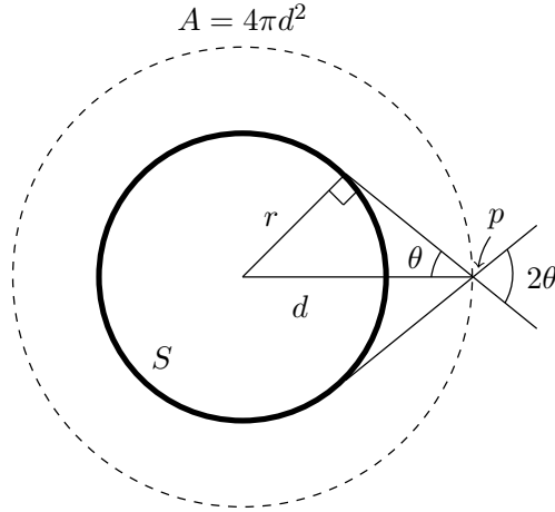
Figure 1.3: Geometric illustration of conservation of étendue, based on a similar figure in [37].
