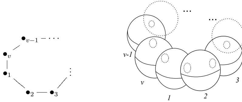
Figure 4.2: Schematic topology of B_3^L [170]
