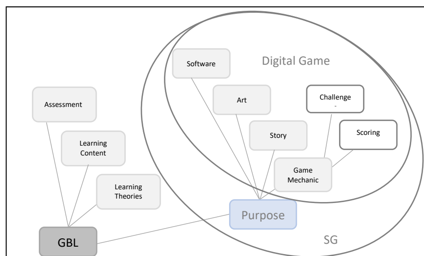
Figure 1.1: GBL Components.
