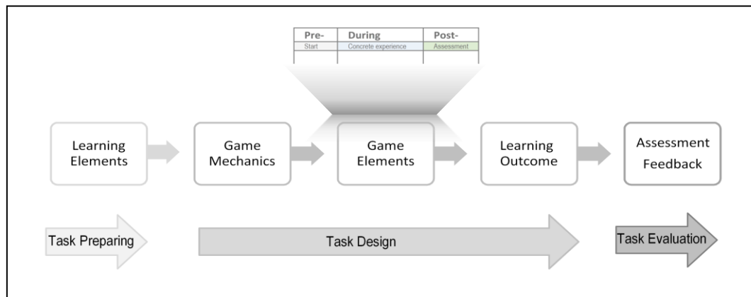
Figure 4.11: Task model.
