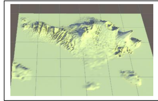
Figure 6.5: Terrain of Bali.
