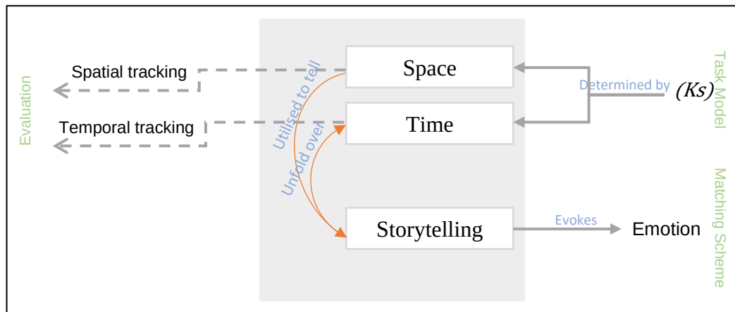
Figure 4.28: World modelling.
