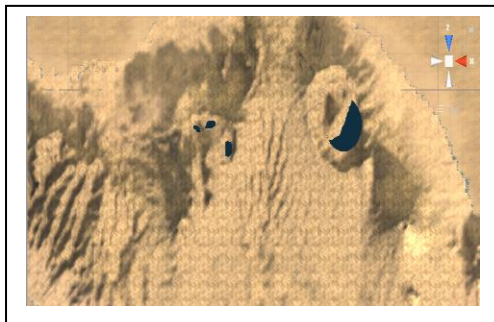
Figure 6.6: Volcanoes' lakes.
