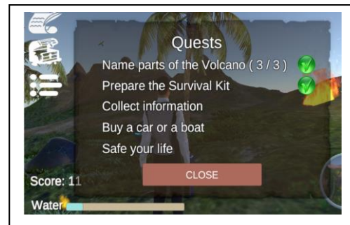
Figure 6.7: Quests list.
