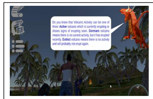
Figure 6.17: Learning materials.
