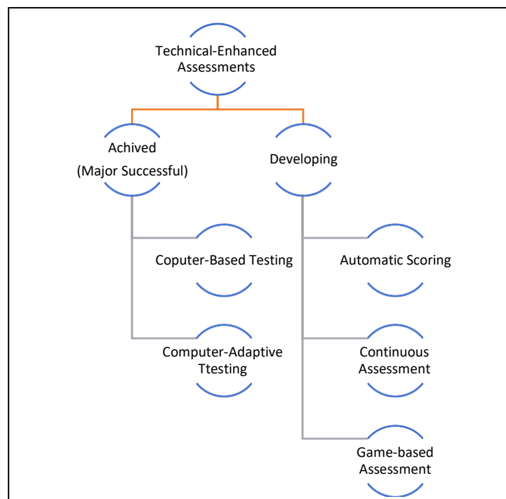
Figure 2.2: E-assessment categories
