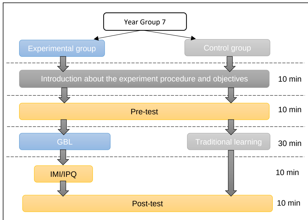
Figure 7.1: Experiment design.
