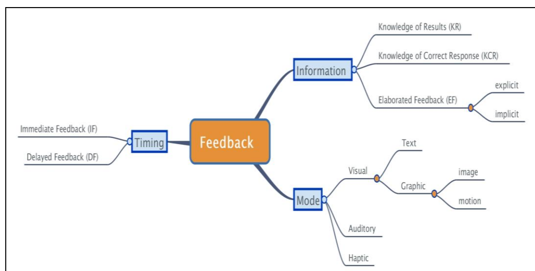
Figure 2.3: Feedback categories.
