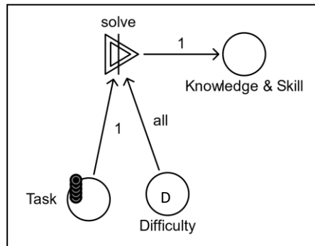
Figure 4.14: Constructing block.
