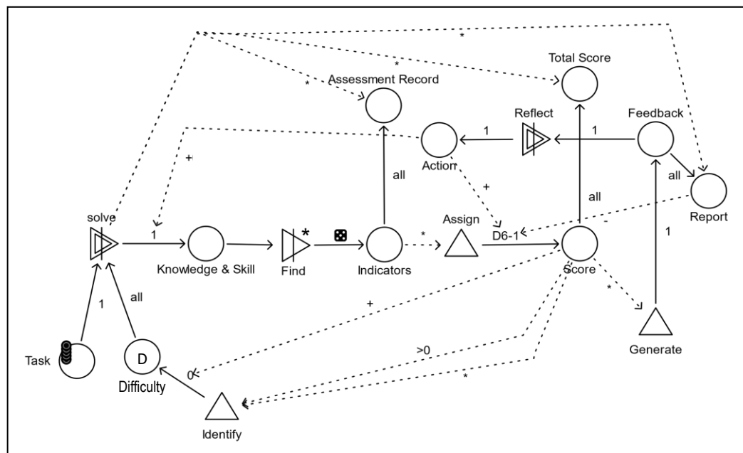
Figure 4.18: Evaluation model.
