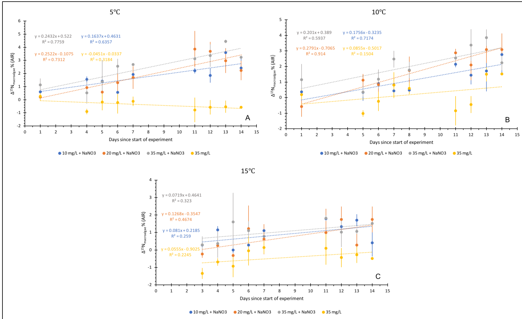
Figure 2.1: \Delta^{15}\text{N} values of Fucus vesiculosus tips cultured in solutions of varying salinity containing NaNO 3 at a concentration of 11.3 mg NO 3 - -N/L. One solution did not contain NaNO 3 to act as the control (35 mg/L). Three experiments were conducted at 5°C, 10°C, and 15°C, representing graphs A, B, and C respectively. Means and standard deviations are representative of three sampled tips. Note the y-axis does not begin at zero.
