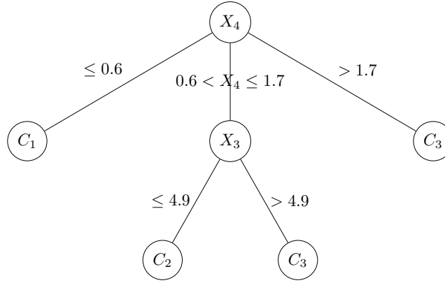
Figure 4.3: Classification tree of Iris data set created by the NPI 3 -Tree algorithm, where a = 0.77 , b = 0.75 and c = 0.80 .
