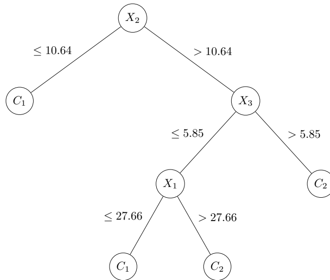
Figure 3.3: Classification tree created by NPI 2 -Tree algorithm, with a = 0.56 and b = 0.50 .
