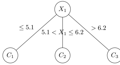
(b) Tree with a multiple split
