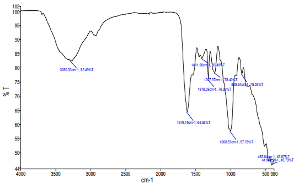
Figure 6. Fourier-Transformed Infrared analysis of the ulvan extracted from the Ulva sp. The corresponding peaks to the sulfate esters (1227 cm -1 ) and peaks related to the uronic acid (1620 cm -1 ) are observed.
