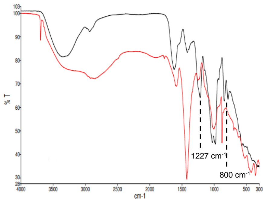
Figure 11. FTIR spectra of as obtained ulvan fraction (black) and ulvan fraction after hydrolysis (red). Drastically reduction of the sulfate ester peak at 1227cm -1 .
