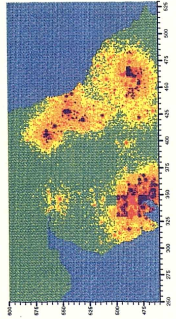
Generation 8
