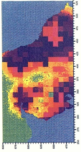
Generation 20
