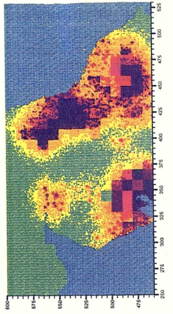
Generation 12
