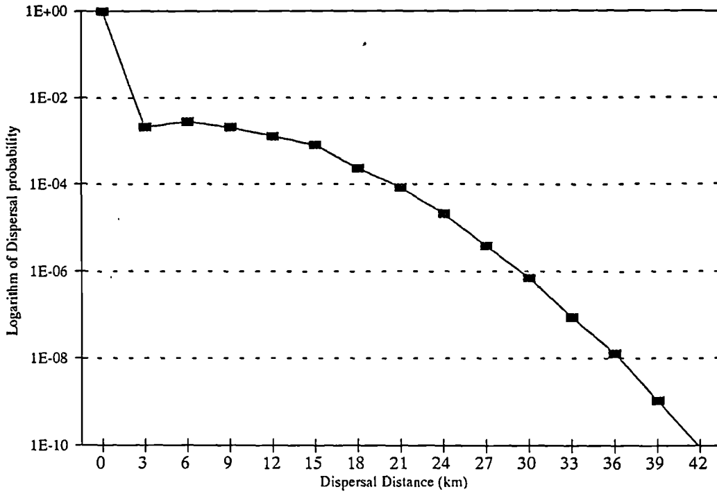
Fig. 4.10 Dispersal distances achieved during a simulation with case I parameter values and a homogeneous environment.
