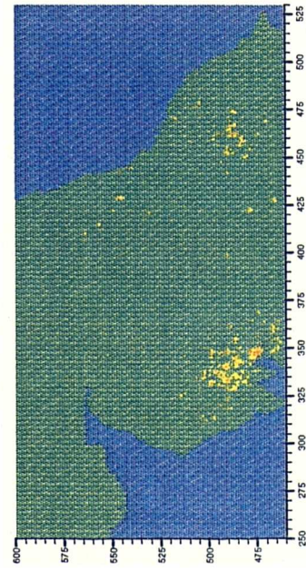
Generation 4
