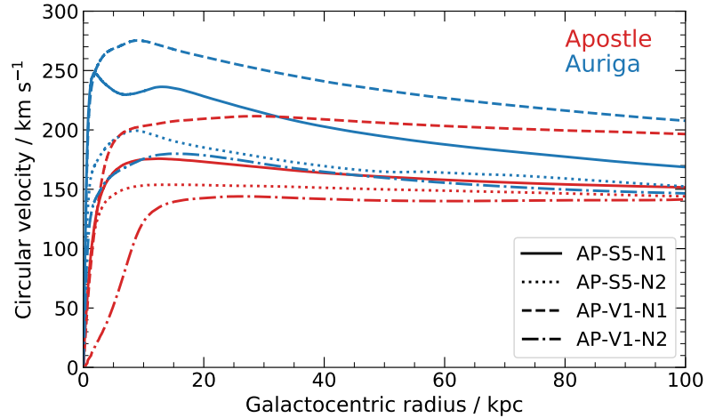
Figure 4.18: The approximate circular velocity of the four primary haloes in both APOSTLE and AURIGA at z = 0 . The circular velocity, V_{\text{circ}} , at radius r is calculated from the total enclosed mass, M(< r) , assuming spherical symmetry V_{\text{circ}}^2 = GM(< r)/r where G is the gravitational constant. The APOSTLE and AURIGA simulations are shown in red and blue, respectively.
