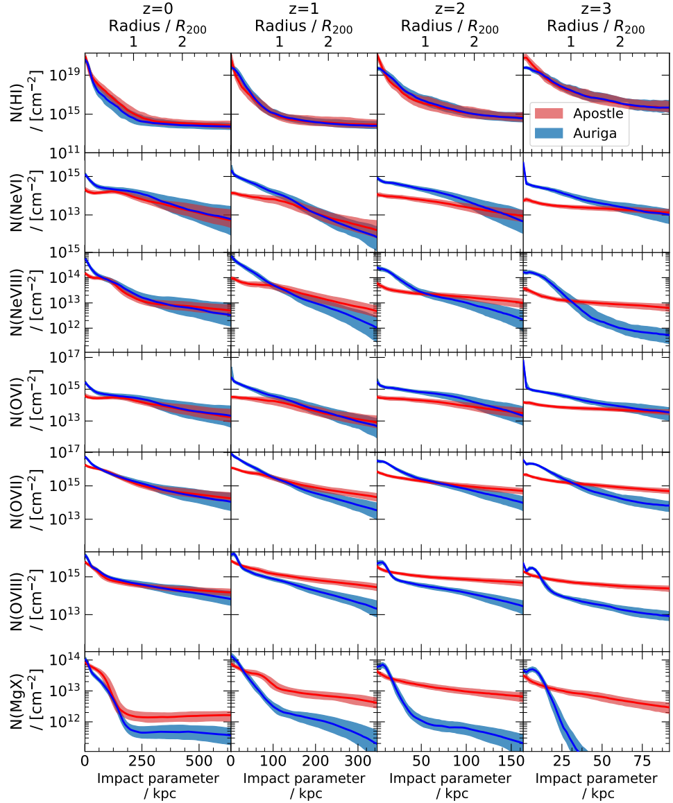
Figure 4.20: Atomic column number densities of several species as a function of impact parameter from the centre of the primary halo in both the APOSTLE (red) and AURIGA (blue) simulations, out to 3R_{200} at four redshifts z \sim 0, 1, 2, 3 from left to right, respectively. From top to bottom, the rows show results for H I, Ne VI, Ne VIII, O VI, O VII, O VIII and Mg X, respectively. The column density at a fixed radius, r , for each halo is calculated by taking the median column density of many sightlines through a small annulus. We also compute the lower and upper quartiles of the column density in each annulus. The solid lines are the mean of the median column density, at each radius, for all four haloes. The shaded regions illustrate the range between the mean of the lower and upper quartiles for all of the haloes. We choose to use the median and quartiles as these are more comparable to a single random line-of-sight through a halo in the real universe. The results are binned by impact parameter, and the mean virial radius is used to show the approximate impact parameter as a function of R_{200} for all four haloes on the same plot.
