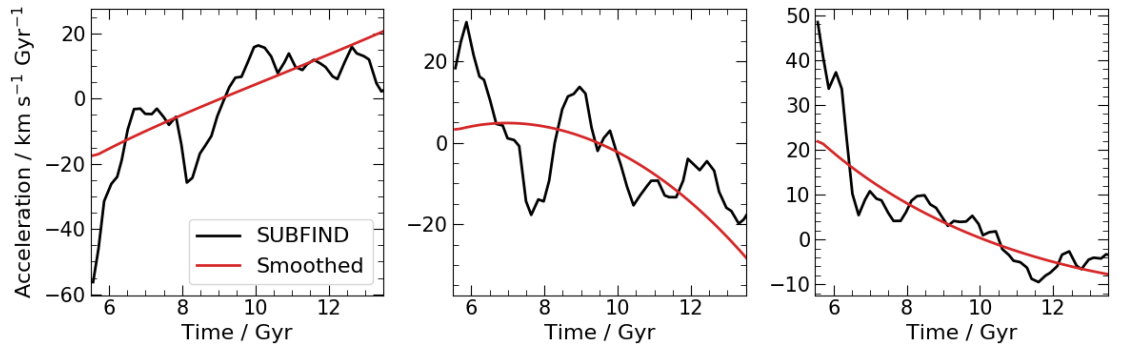
Figure 5.6: Similar to Fig. 5.4 but for the peculiar acceleration of the primary halo in the AURIGA Au16 (DMO). The SUBFIND value is calculated by taking the first derivative of the peculiar velocities reported by the halo finder. We also show a smooth approximation (red line) to the peculiar acceleration calculated from the second derivative of the smoothed halo trajectory shown in Fig 5.4.
