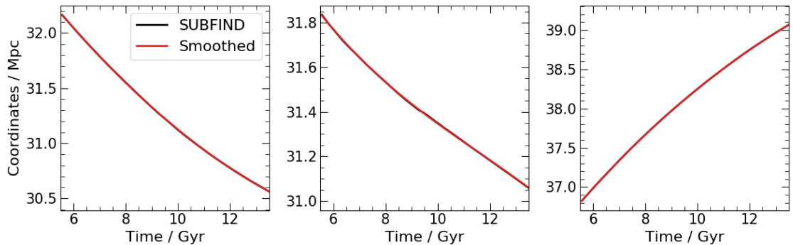
Figure 5.4: The centre of the primary halo of the AURIGA Au16 (DMO) simulation, in the simulation box frame, as a function of time. The coordinates in the x -, y -, and z -axes are shown in the three panels from left to the right, respectively. The centre of the halo is taken to be the centre of the potential as reported by SUBFIND. We also include a smoothed spline approximation to the halo centre.
