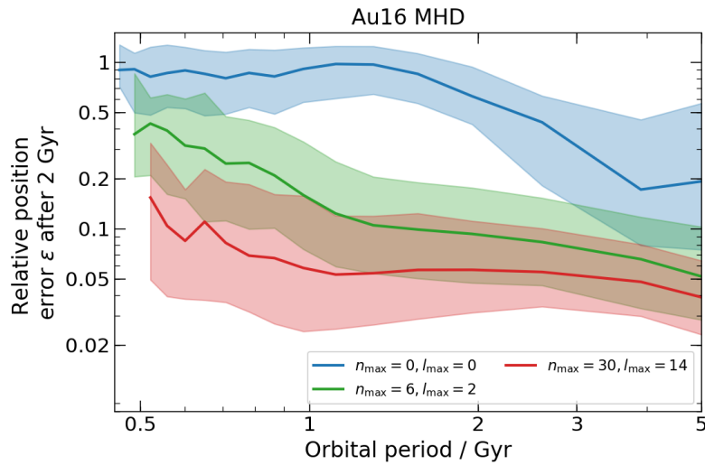
Figure 5.20: The same as Fig. 5.18 but for 25000 random dark matter particle orbits taken from the MHD Au16 halo and evolved with the coefficients generated from the baryonic halo.
