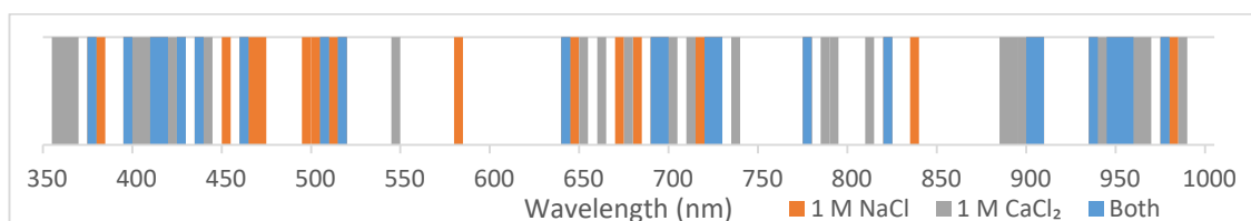
Figure 5-5: Wavelengths at which the 1 M NaCl, 1 M CaCl 2 or both the 1 M NaCl and the 1 M CaCl 2 measurements were outwith the 2σ range obtained by repeat measurements of DI water.
