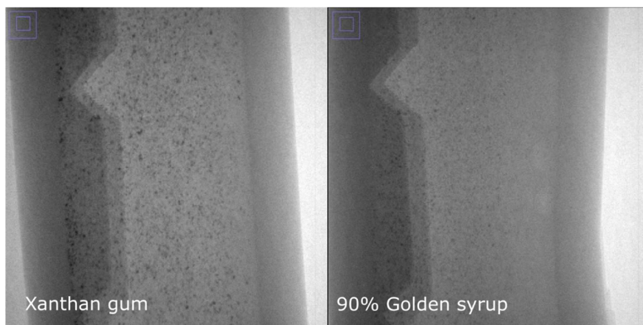
Figure 6-40: API barite in 6.25 g/l xanthan gum and 90% w/w golden syrup/water. 100 KV, 10 W, 1 s/image with binning set to 2 and angle varying from 0° to 1° over the duration of the scan. 13.18 \mu\text{m}/\text{pixel} .
