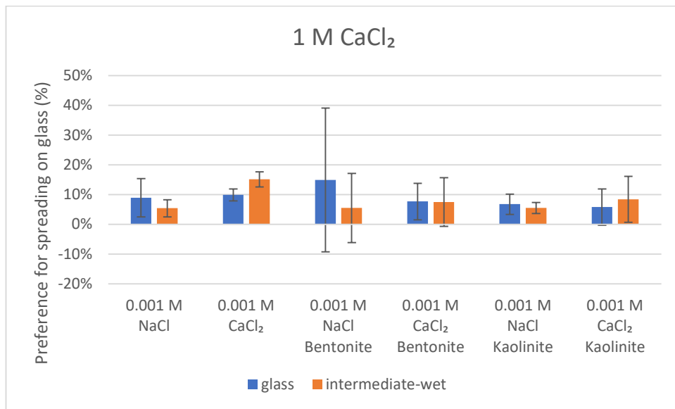
Figure 6-28: Salinity contrast drop spread on intermediate wet patterned slide – 1 M CaCl 2 bulk solution. Series names denote whether drop spread initiated from glass or intermediate-wet surface.
