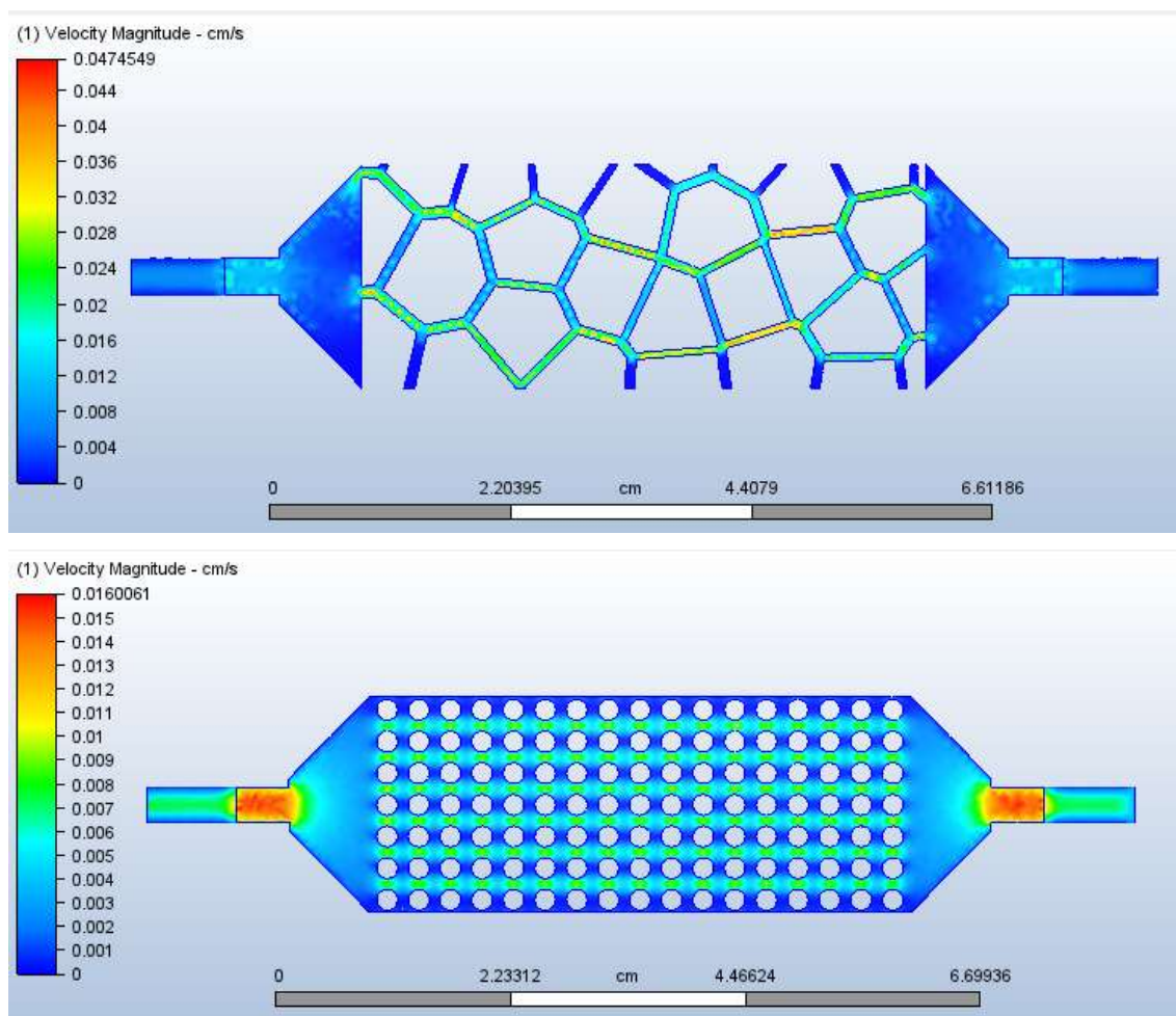
Figure 6-50: Simulation of flow of 6.25 g/l xanthan gum in different flow cells after 50 s flow at 0.02 cm 3 /minute. Flow from right to left.
