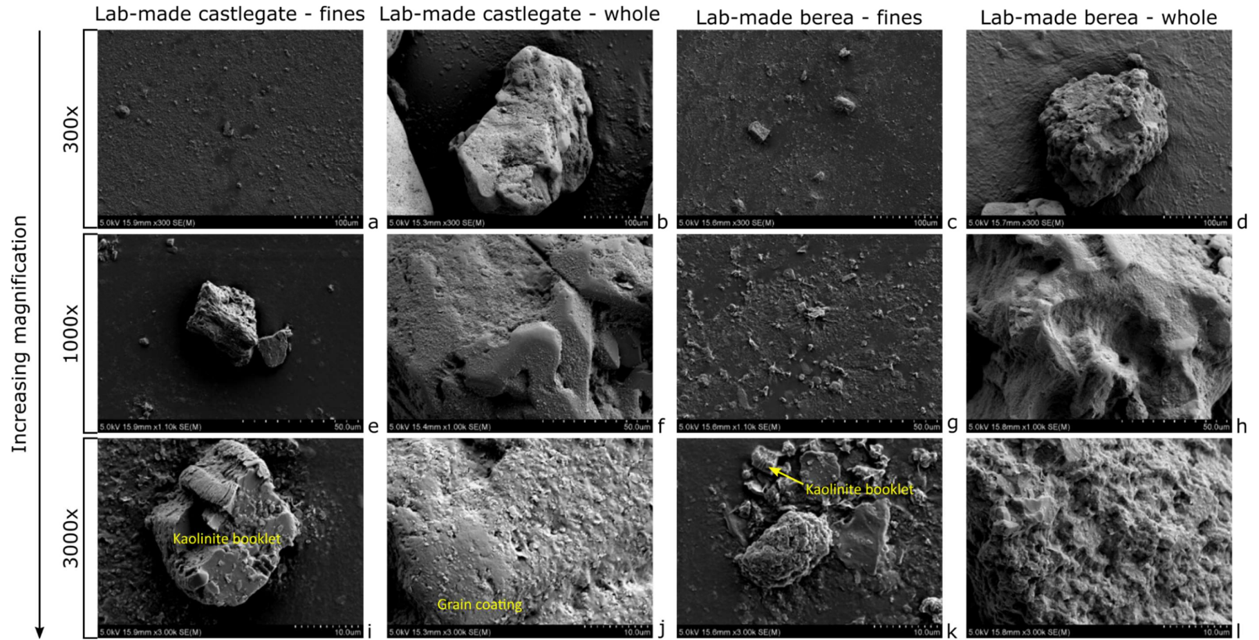
Figure 5-20: Lab-made synthetic Castlegate and Berea treated with ultrasound to break apart the sandstone and remove the fines from the sand grains. a-d: 300x magnification, e-h: 1000x magnification, i-l: 3000x magnification
