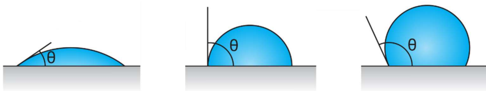
Figure 6-1: Illustration of contact angles vs surface wettability. Left to right: water-wet, neutral-wet, oil-wet.
