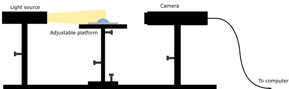
Figure 3-12: Schematic of a typical contact angle goniometer. The light source and camera are fixed, but the sample platform can be adjusted to give a variety of measurement options and the ability to accommodate a number of substrate sizes.
