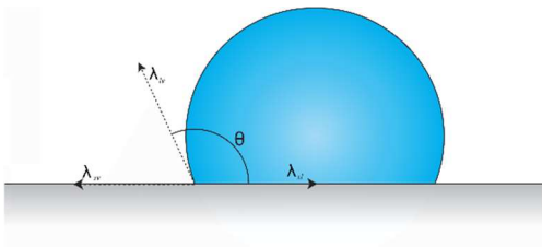
Figure 3-9: Surface tension balance contributing to wettability. Grey: surface, blue: water, white: air, \vartheta : contact angle, \lambda : surface tensions at liquid-solid, liquid-air and solid-air boundaries.
