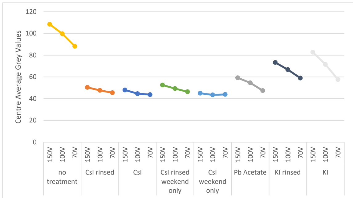
Figure 6-35: Grey values averaged over the centre of the top 1/4 of clay pellet images.
