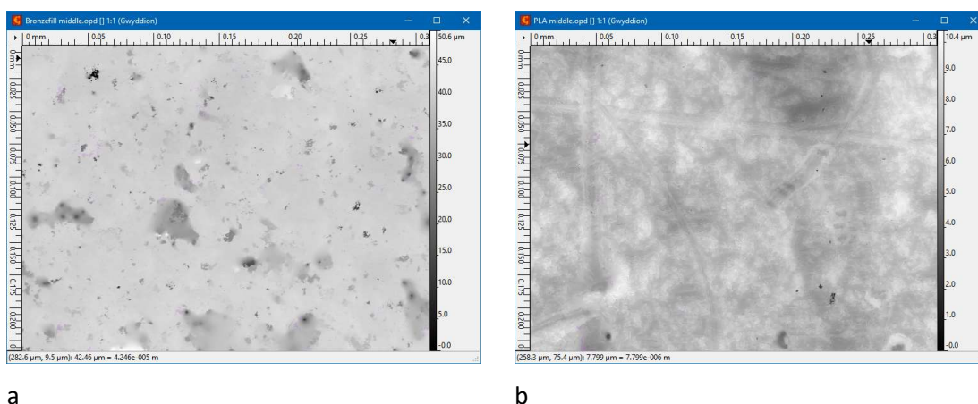
Figure 4-8: a - Bronzefil (height colour scale: 0 – 50 \mu\text{m} ), b - PLA (height colour scale: 0 - 10.4 \mu\text{m} ), both on PEI, illustrating variation in maximum height between materials.
