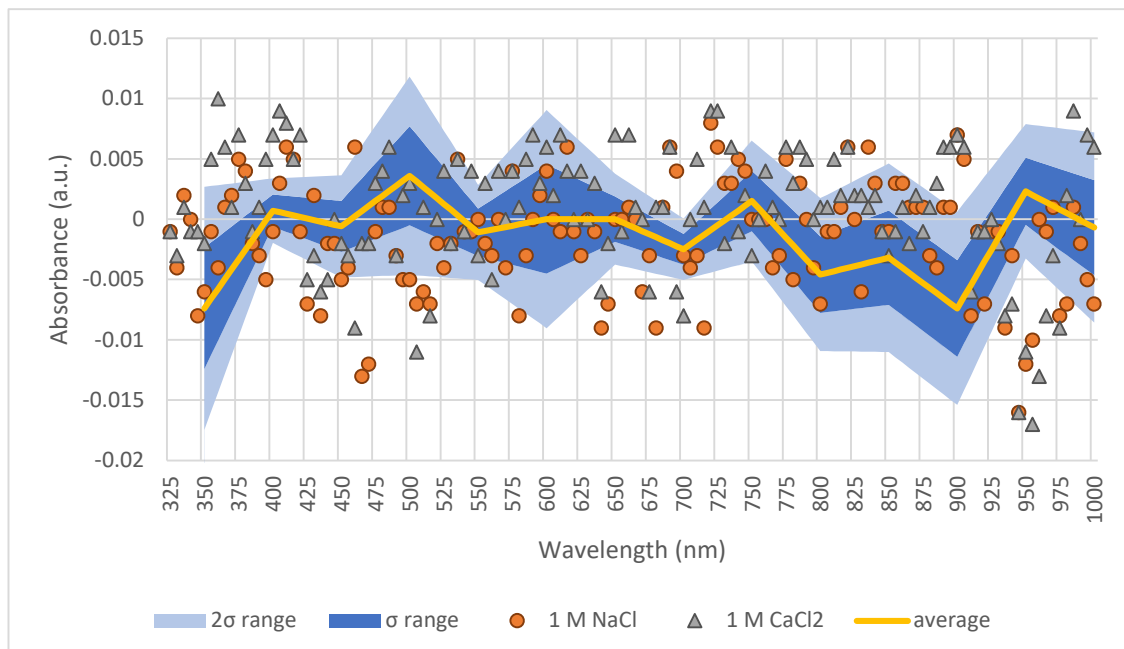
Figure 5-4: Salt solution measurements overlaid on 1σ and 2σ-variations based on repeated measurements of DI water.
