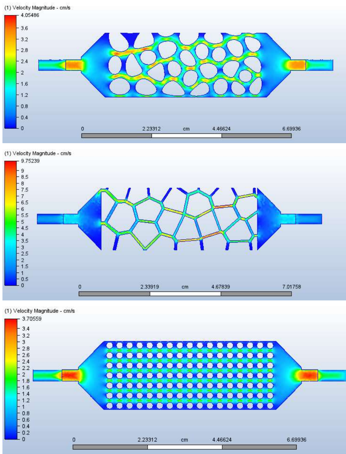
Figure 6-46: Simulation of flow of water in different flow cells after 180 s flow at 5 \text{ cm}^3/\text{minute} . Flow from right to left.
