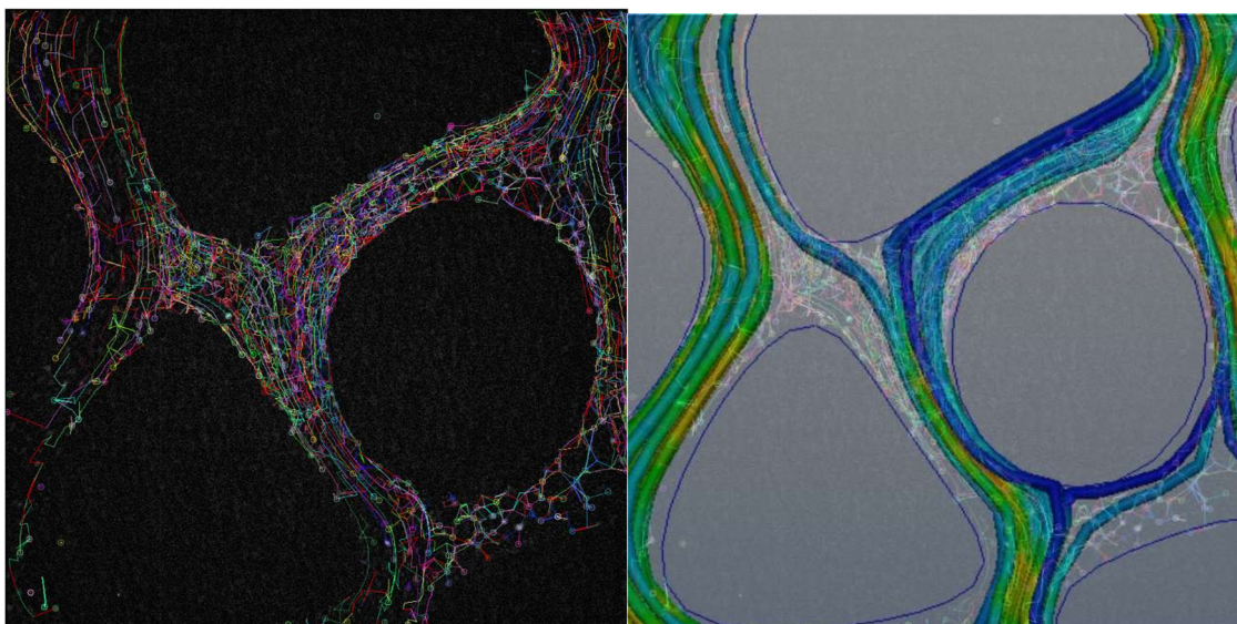
Figure 6-52: Tracked particles (L) and simulated particle flow pathways overlaid (R). Velocity magnitude colouring for simulated particle flow lines (blue – slowest, red – fastest)
