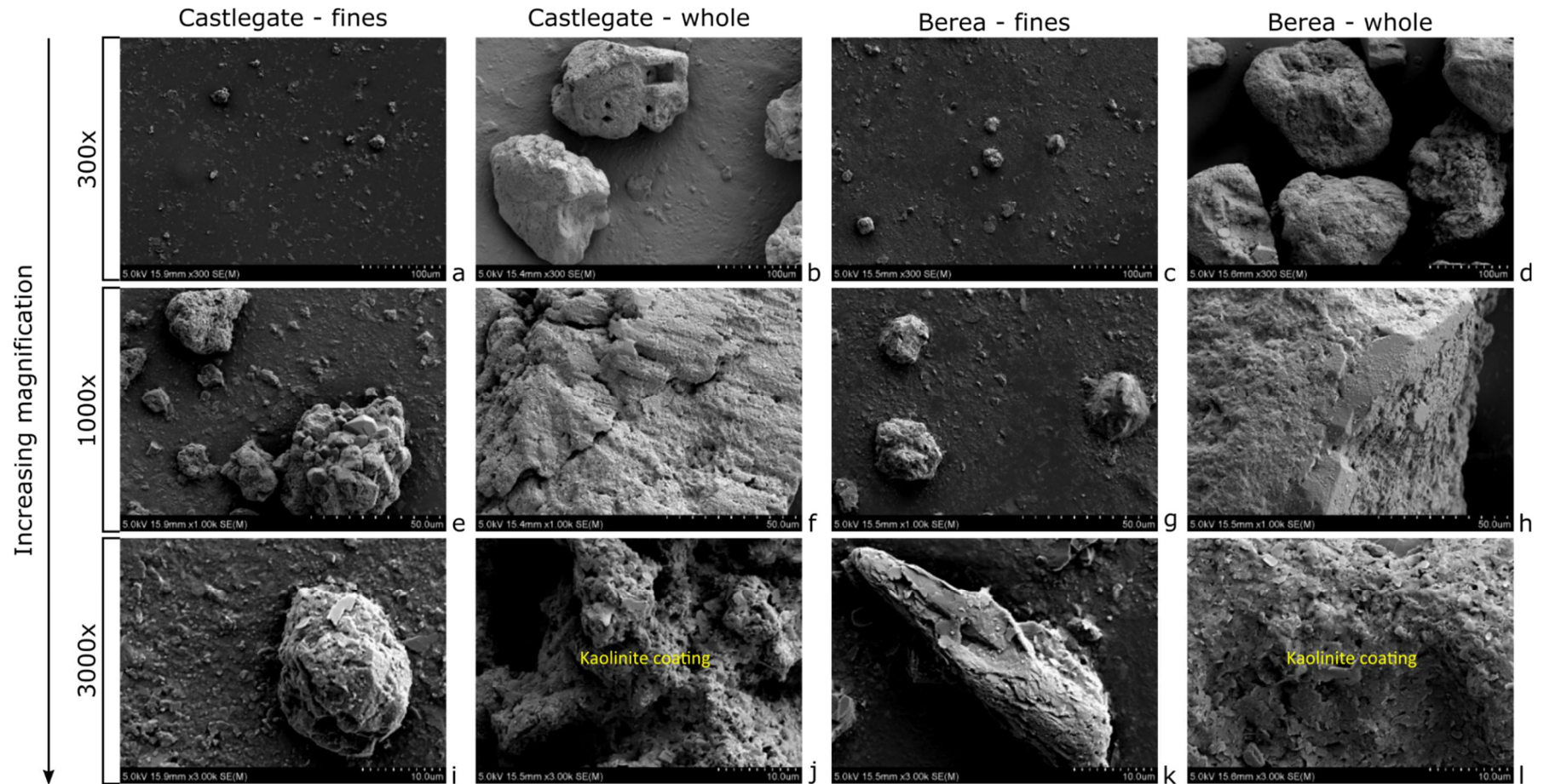
Figure 5-19: Castlegate and Berea sandstones treated with ultrasound to break apart the sandstone and remove the fines from the sand grains. a-d: 300x magnification, e-h: 1000x magnification, i-l: 3000x magnification.
