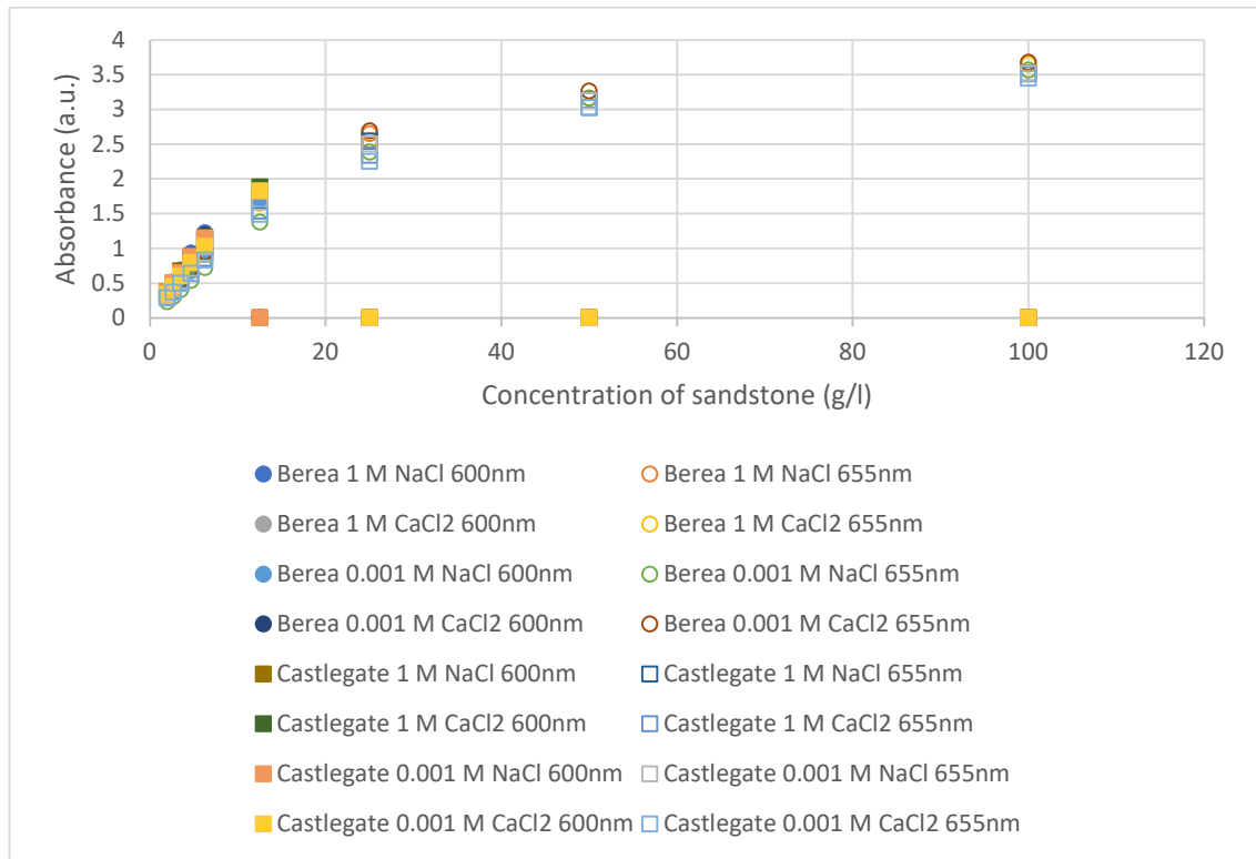
Figure 5-7: Calibration curve for lab-made model sandstones.
