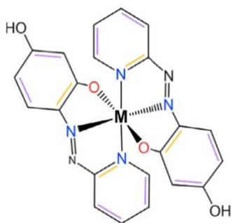
Figure 8 \text{Zn}(\text{PAR})_2 complex. Zn stated as M.
