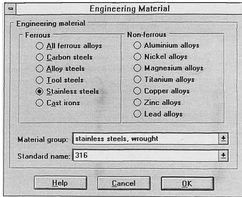
Figure 4.5: Material specification by AISI standard designation
