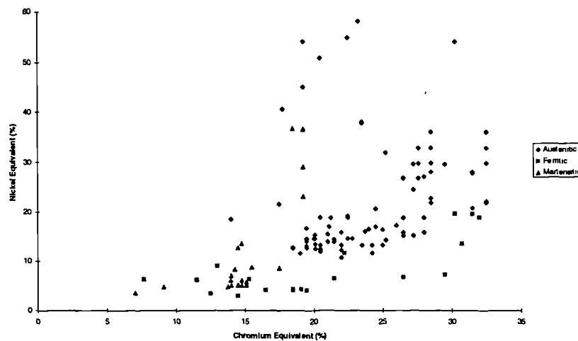
Figure 4.3: Stainless steel phase type plotted on the Schaeffler chromium equivalent against nickel equivalent graph
