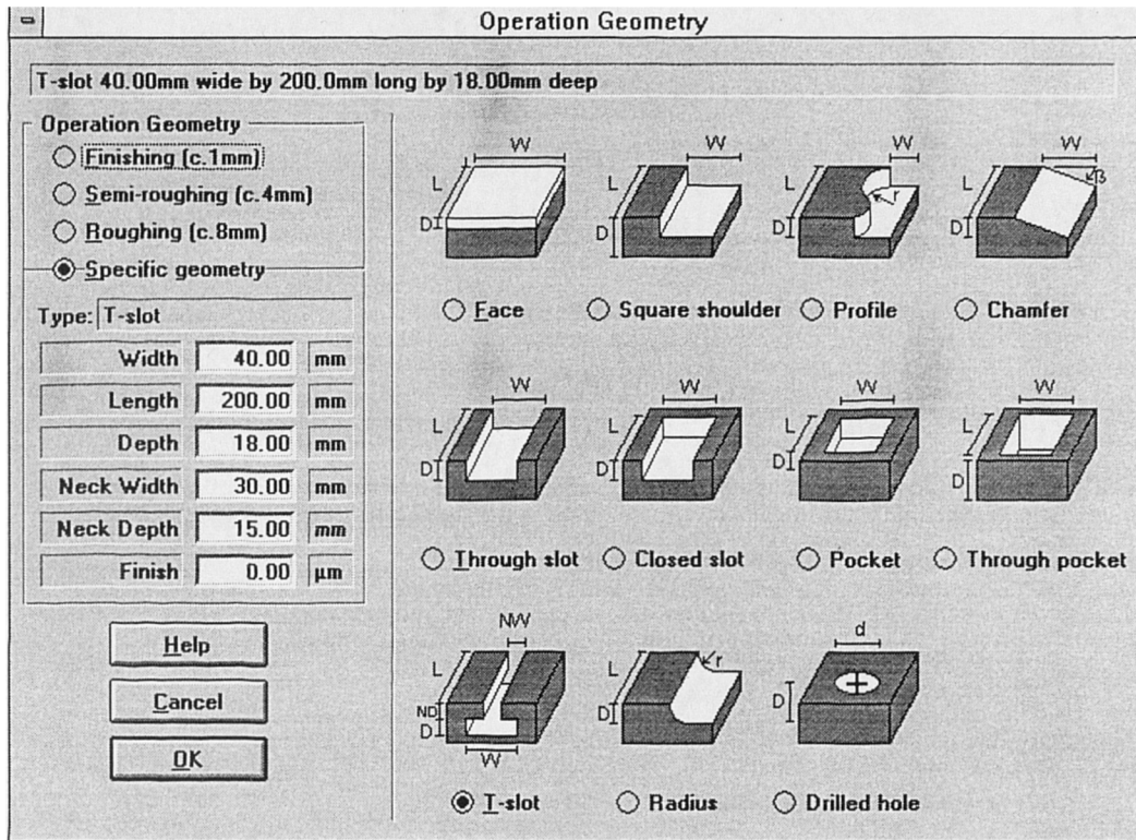
Figure 3.5: Operation definition interface
