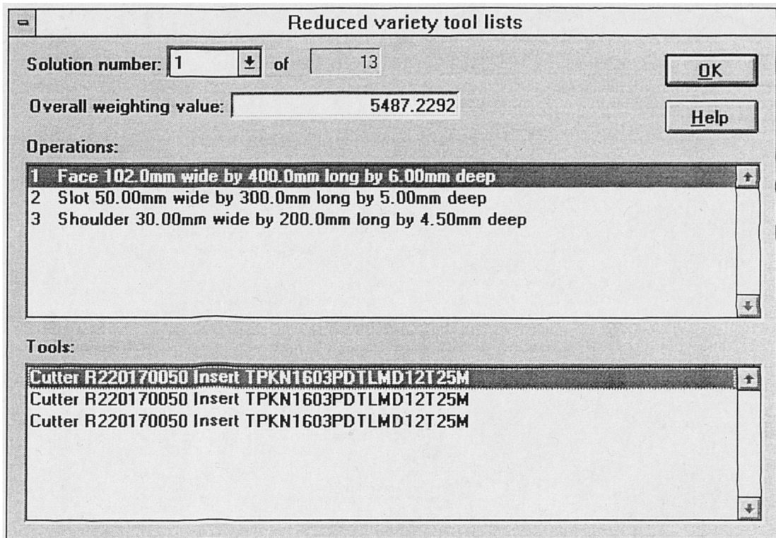
Figure 6.4: Results display of the tool variety reduction method
