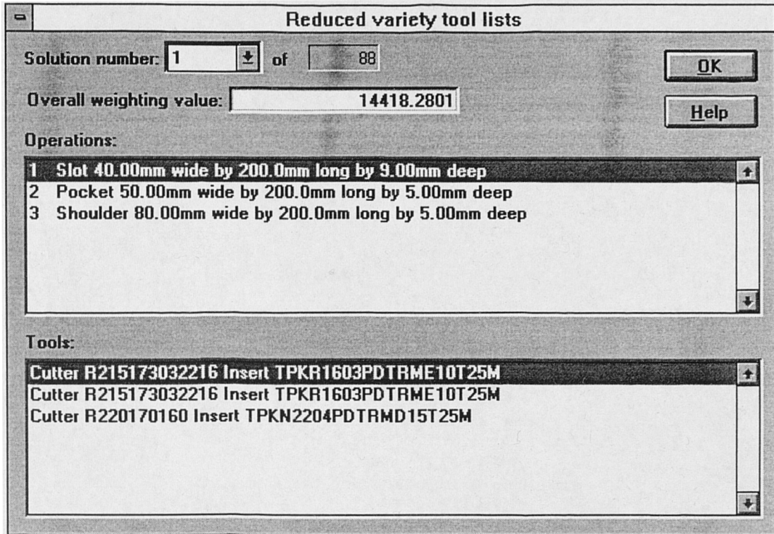
Figure 8.7: Tool variety reduction example results
