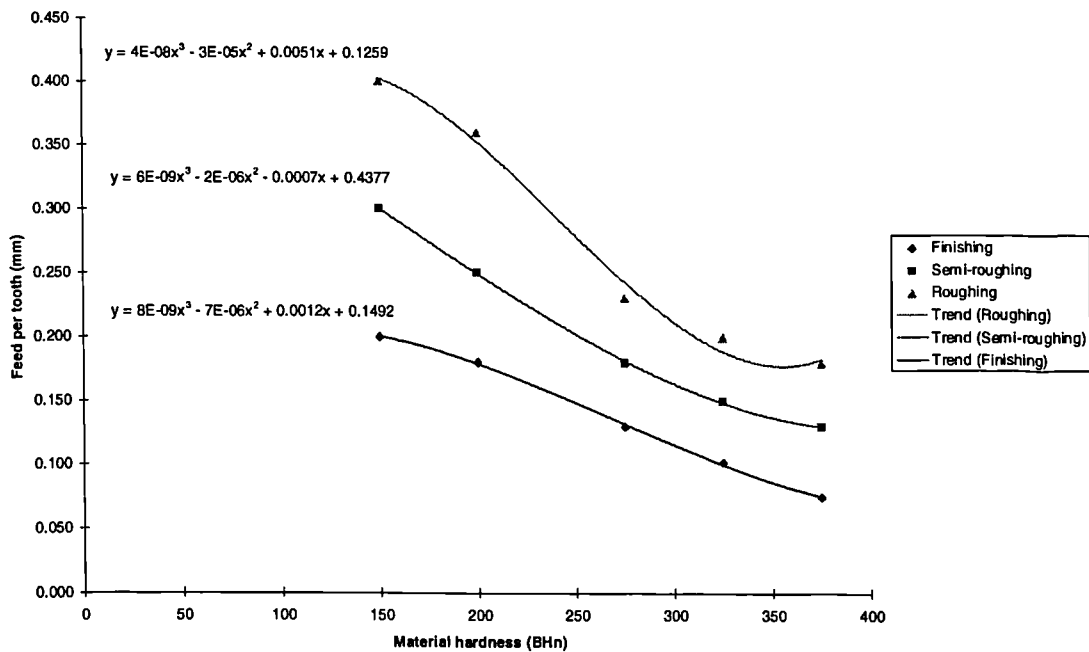
Figure E.2: Regression curves of fed per tooth against material hardness for free machining alloy steels, wrought (medium carbon resulfurized)
