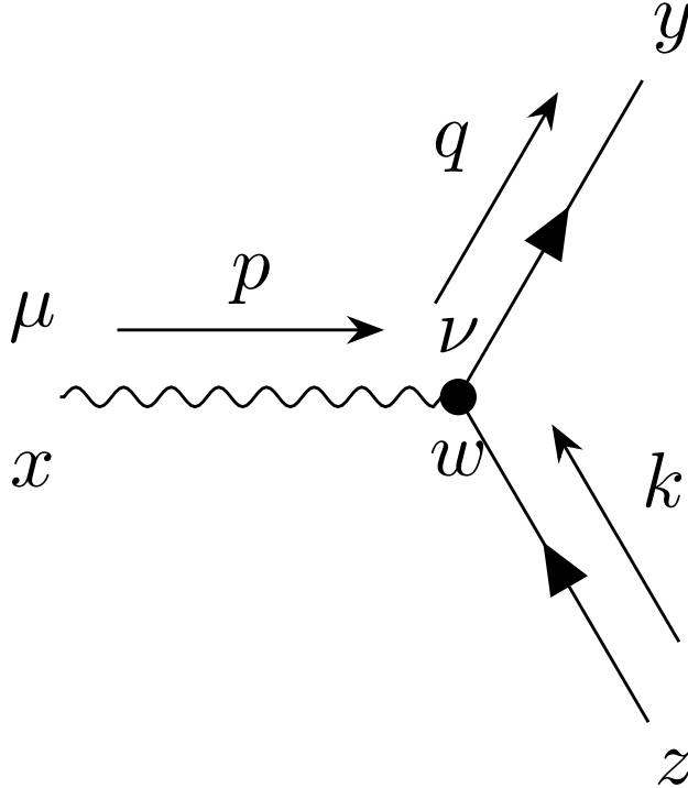
Figure 5.5: Feynman diagram for \langle \mathcal{T} A_\mu(x) \bar{\psi}(y) \gamma_\nu \psi(z) \rangle as used in the Dirac fermion calculation
