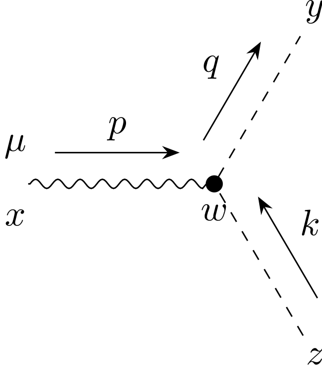
Figure 5.3: Feynman diagram for \langle \mathcal{T} A_\mu(x) \phi^\dagger(y) \phi(z) \rangle as used in the complex scalar calculation
