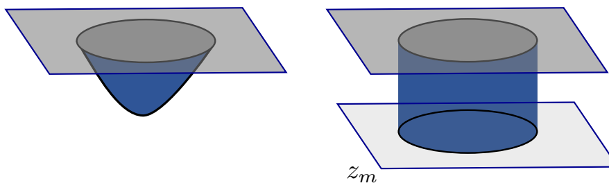
Figure 3.3: Two distinct topologies that are possible for the DBI monopole. On the left is the situation when the flavour sector is gapless; the D7 -brane then has no boundary, and the DBI monopoles hangs down into the bulk with a disc topology, whose action depends non-locally on the data describing the boundary curve. On the right, when the flavour brane ends, the D5 -brane is also allowed to end, permitting a cylinder topology. The action of this configuration depends only on the perimeter of the boundary curve.
