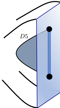
Figure 3.1: The hanging D5 -brane forms 1-dimensional worldline in the bulk; it is the boundary of N_c F-string worldsheets which also intersect the AdS boundary. At their intersection with the boundary they define the insertion of fundamental Wilson lines in the dual CFT.
