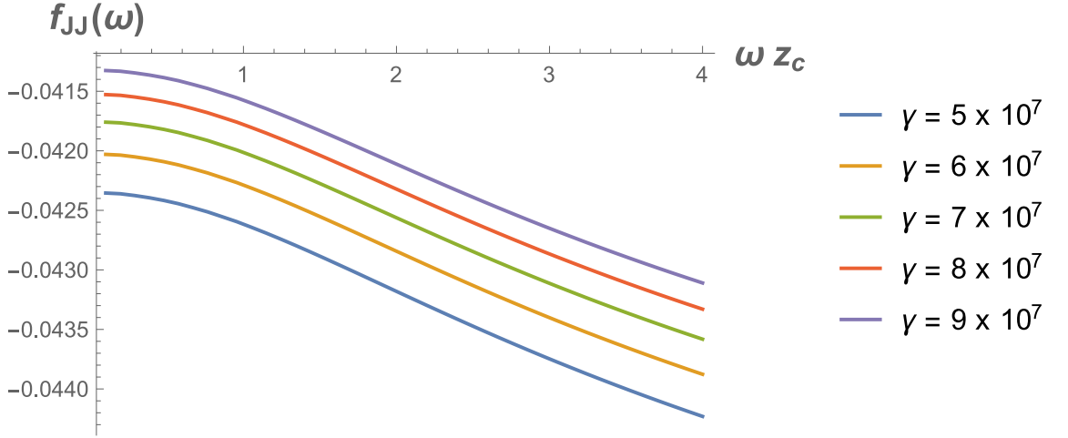
Figure 3.6: The symmetry current correlator at strong coupling as a function of w = \omega z_c for various masses, computed numerically using holography. For this plot we set \bar{z}_* = 10^{-8} .
