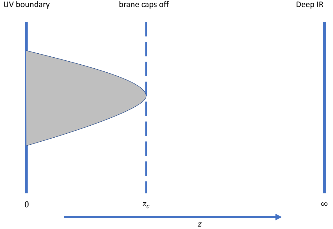
Figure 3.4: Brane caps off at z = z_c
