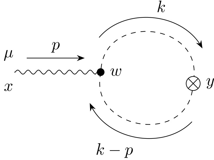
Figure 5.1: Feynman diagram for \langle \mathcal{T} J^{02}(x) T_{(S)}^{23}(y) \rangle formed by sewing together the ends of the three-point function \langle \mathcal{T} A_\mu(x) \phi^\dagger(y) \phi(z) \rangle
