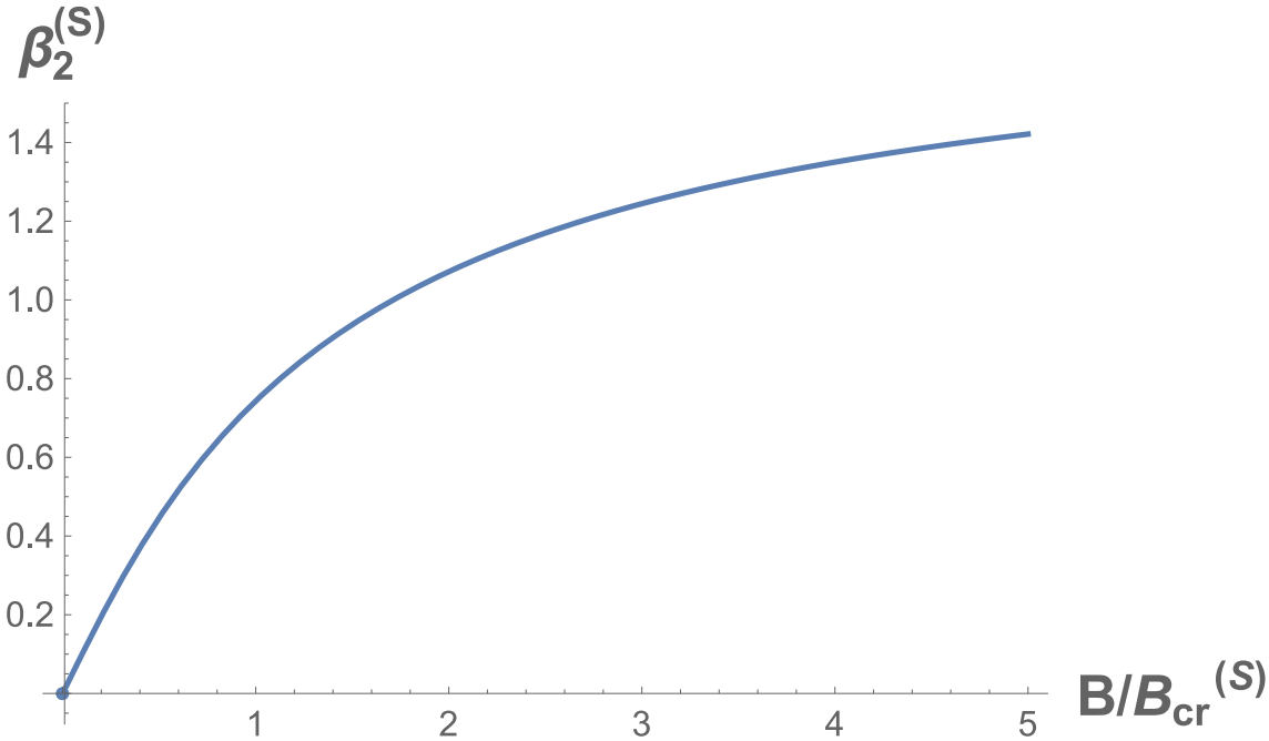
Figure 5.4: Plot of \beta_2^{(S)} (in units of \frac{e}{120\pi^2} ) for the complex scalar as a function of B/B_{cr}^{(S)}
