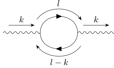
Figure 3.8: Fermion loop diagram contributing to correction of photon propagator
