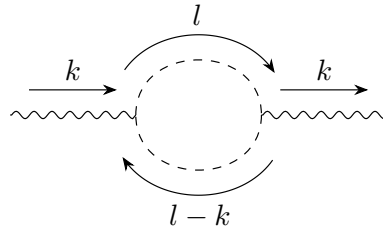
Figure 3.7: Scalar loop diagram contributing to correction of photon propagator
