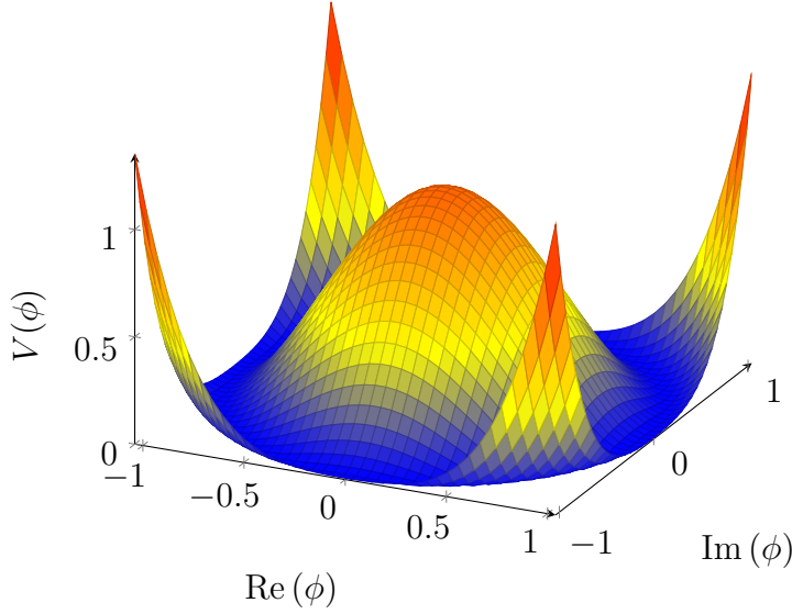
Figure 2.1: Plot of the “Wine Bottle” potential for \lambda = 4 and v^2 = 2
