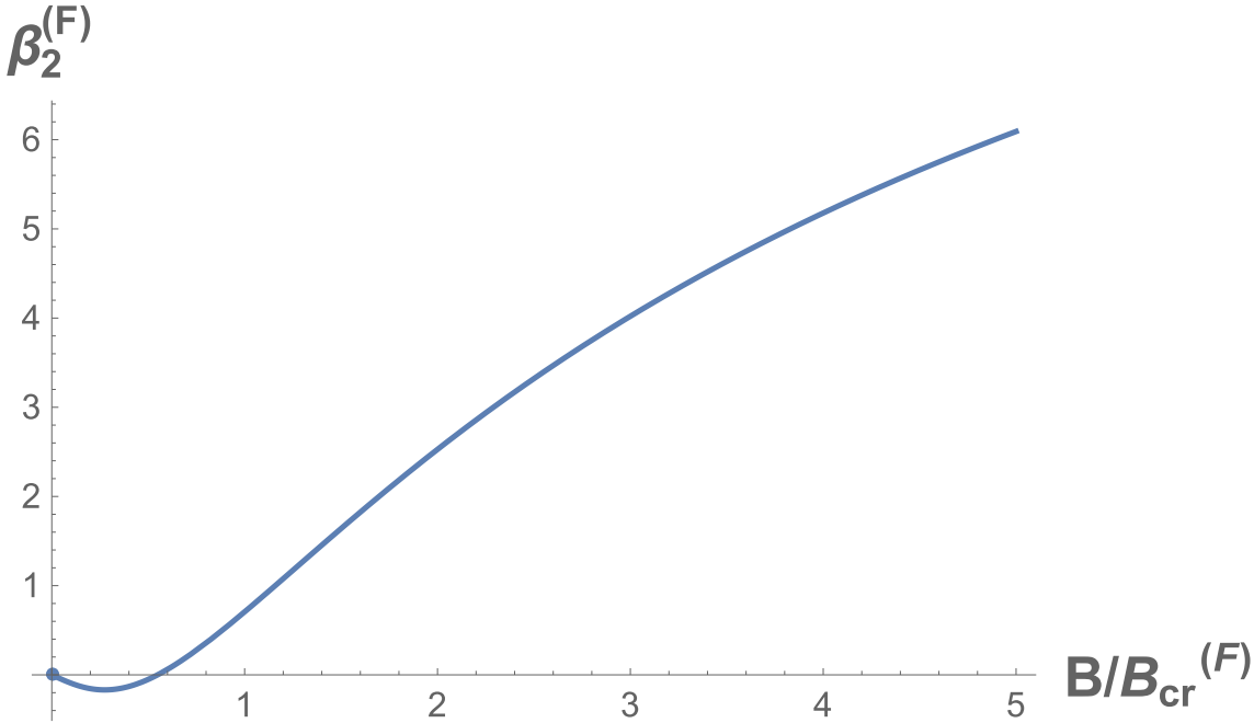
Figure 5.6: Plot of the transport coefficient in units in units of e/240\pi^2 for the Dirac fermion as a function of B/B_{cr}
