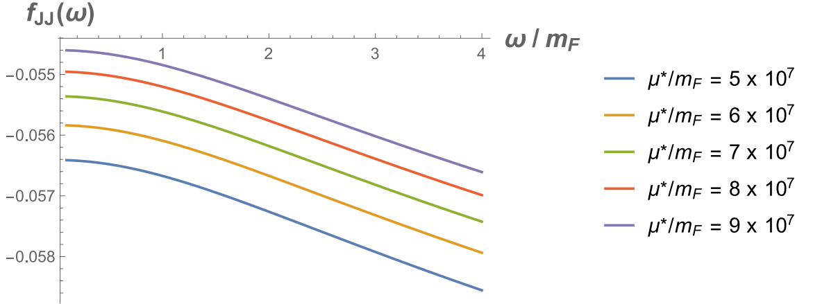
Figure 3.9: The symmetry current correlator at weak coupling as a function of \hat{\omega} = \omega/m_F , computed analytically in perturbation theory
