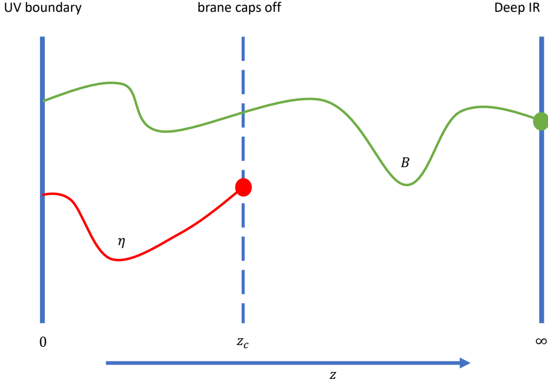
Figure 3.5: B_2 (in green) evolves continuously from the IR to the UV boundary; \eta_1 (in red) is “born” at the brane cap and evolves to the UV
