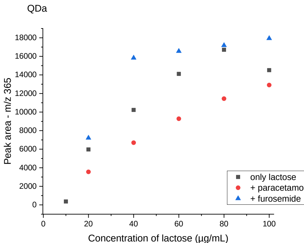
Figure 8.297 – QDa data showing the peak area of increasing concentrations of lactose in solution either alone (black squares), or with a concentration of 20 µg/mL of paracetamol (red circles) or furosemide (blue triangles). The SIM channel from which the signal was obtained followed m/z 365.
