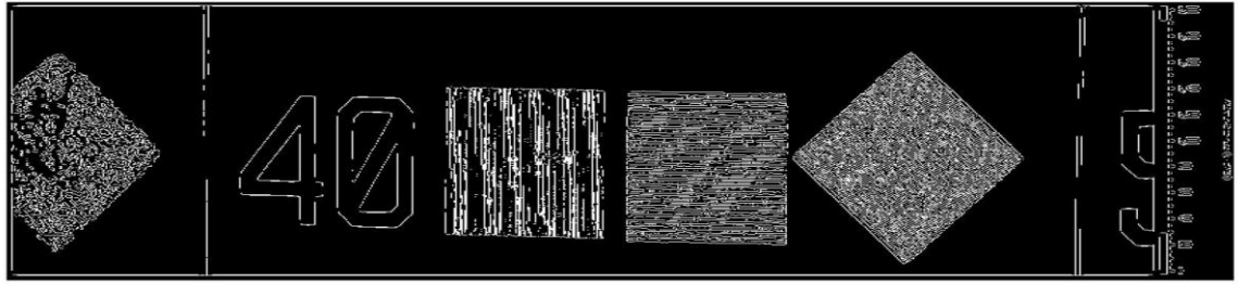
Figure 5.155 – Absorbance map using visible wavelength (520 nm) and 40 grid. Converted from Jet colour map to grey scale to black and white with a threshold of 100/255 and the canny edge function applied. Extracted from frame 360 of 591.
