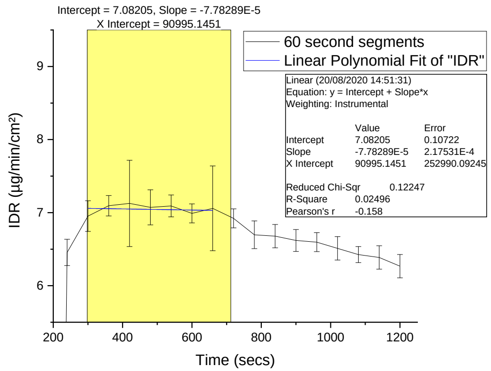
Figure 3.35 – Linear regression analysis for section of IDR between 300 and 720 seconds (highlighted region).
