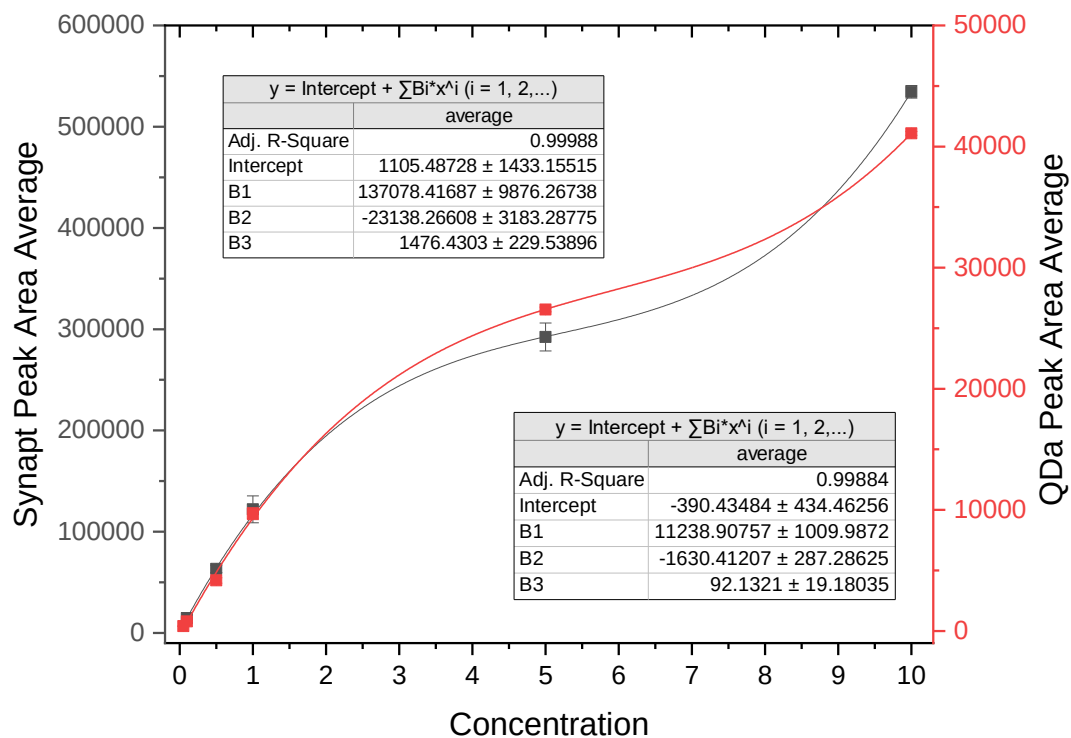
Figure 7.242 – Synapt and QDa calibration plots on left and right y-axes, respectively, showing only concentrations between 0.05 and 10 µg/mL. Each point is the average of three runs, with standard deviation shown using error bars.
