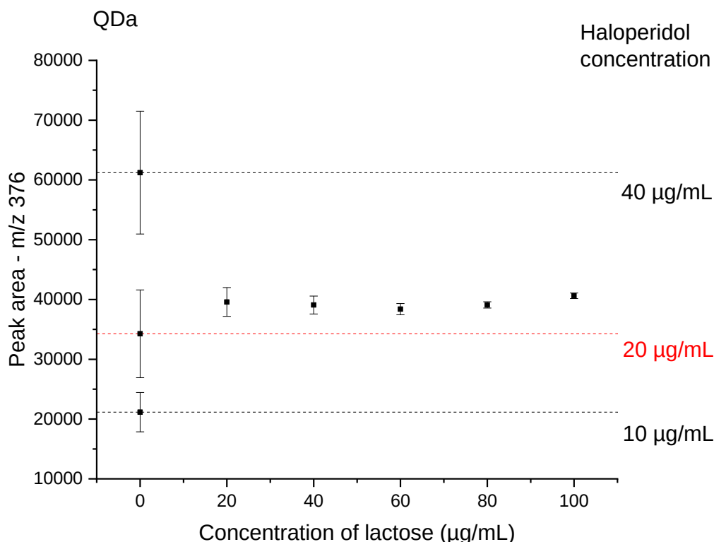
Figure 8.295 – QDa data showing the effect of increasing the concentration of lactose upon the peak area value (signal) obtained for haloperidol following an ES+ SIM channel of m/z 376. The concentration of haloperidol was kept constant at 20 µg/mL. Comparative signals obtained for haloperidol concentrations without lactose present are shown by the dashed lines, with a red line showing the concentration of 20 µg/mL, which is the same as that found in the solutions mixed with lactose, and two black lines showing 10 µg/mL and 40 µg/mL for comparison. Error bars showing standard deviation are included for each point, which are a result of each sample being run and analysed in triplicate.
