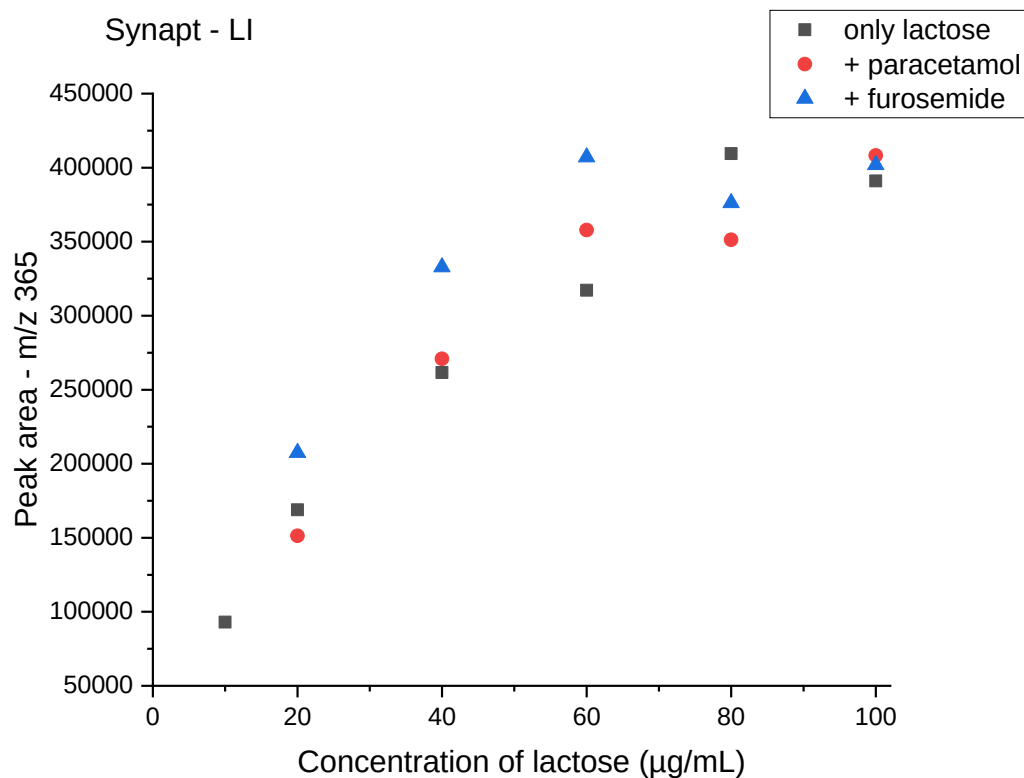
Figure 8.309 – Synapt data showing the peak area value (signal) of increasing concentrations of lactose in solution either alone (black squares), or with a concentration of 20 µg/mL of paracetamol (red circles) or furosemide (blue triangles). The SIM channel from which the signal was obtained followed m/z 365.
