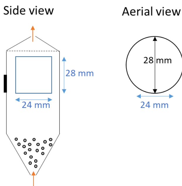
Figure 4.50 – Diagram showing inside the SDi2 whole dose cell from the front (side) and from above (aerial), with orange arrows showing the flow of solvent in and out of the cell. The imaging window is shown in blue. The side view shows the position of the numerous 2 mm glass beads in the bottom section, the wire mesh across the top and the holder for inserting the sample into the cell on the left. Not drawn to scale.
