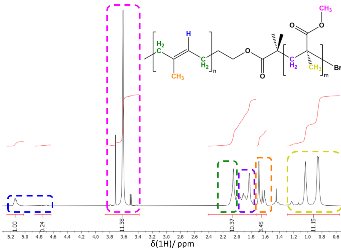
Figure 3.5: ^1H NMR spectrum for a PI - b - PMMA block copolymer. In this instance the sample shown is PI_{32} - b - PMMA_{107} , prepared by ATRP of MMA from the PI_{32} -Br macroinitiator.
