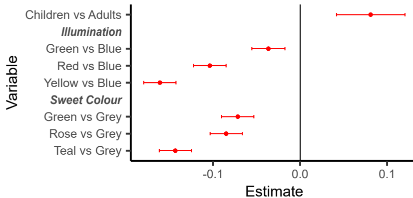
Figure 3.13: Main effects model results. Red circles are estimates, with error bars showing 95% CIs. For estimates greater than 0, the comparison condition predicts higher CCIs; for estimates lower than 0 the reference condition predicts higher CCIs.
