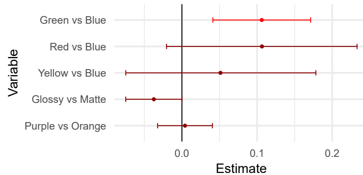
Figure 4.9: Results of lme main effects model on children’s CCIs, with fixed effects of Illumination, Material, and Sweet, and random effect of observer. The reference conditions were Blue illumination, Matte material, and Orange sweets. Any estimates greater than 0 indicate that CCIs under the factor on the left of the Variable equation (e.g. Green in the first row) are greater than the reference (e.g. Blue in the first row). Estimates below 0 indicate that CCIs under the reference condition are higher. Bright red bars show significant effects whereas dark red bars show non-significant effects. Error bars are 95% confidence intervals.
