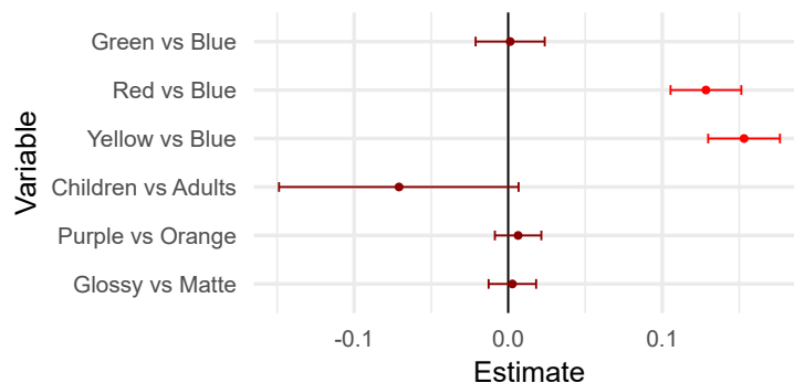
Figure 4.12: Results of lme main effects model with fixed factors of Illumination, Age Group, Sweet, and Material, and random effect of observer, in the same format as Fig. 4.9.
