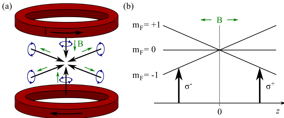
Figure 3.4: MOT operating principles. (a) Setup of orthogonal circularly polarised beams with anti-Helmholtz coils to generate the magnetic field gradient. (b) Magnetic field produces a spatially varying Zeeman shift. For z > 0 \sigma^+ transitions are closer to resonance; for z < 0 the \sigma^- transitions are shifted closer to resonance.
