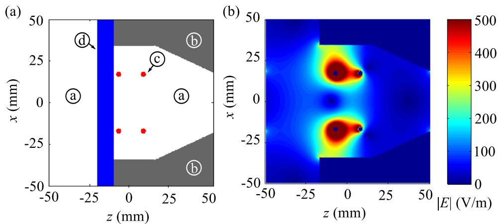
Figure 6.8: (a) Geometry of the key features of the potential used in the electric field calculation. The labelled areas are: (a) free space; (b) the metal bulk of the vacuum chamber; (c) the electrodes; and (d) the dielectric. (b) Resulting electric field magnitude calculated by including only the potential at the electrodes and vacuum chamber.
