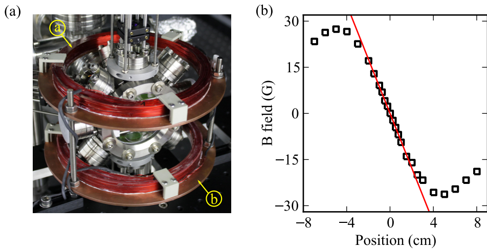
Figure 3.6: MOT coils setup. (a) The coils are labelled ① and their copper heatsinks ②. (b) Shows the magnetic field produced by the coils; the gradient of the central linear region is found to be 8.8 G/cm.
