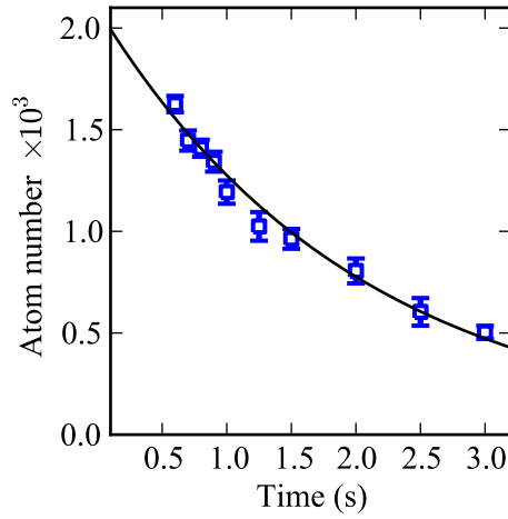
Figure 3.20: Atom number in the dipole trap as a function of the hold time. The atom number is found by collecting fluorescence produced when the atoms are illuminated using the MOT beams set to resonance. The 1/e lifetime is 2.0 \pm 0.1 s.
