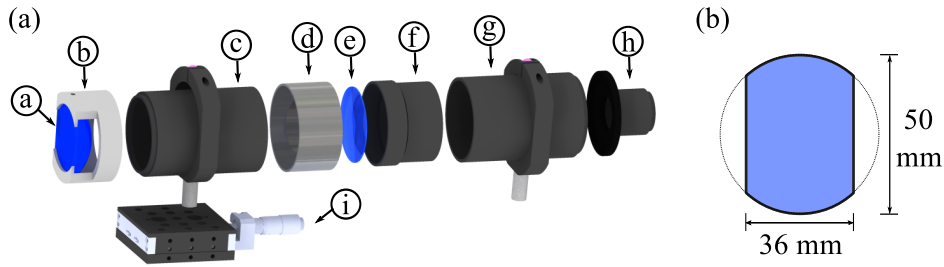
Figure 3.7: Imaging optics setup. (a) Pair of lenses mounted in a sequence of lens tubes collimate light from the MOT and focus it onto the CCD chip, all labels are described in the text. (b) dimensions of the collimating lens showing the modification in its shape made so that the MOT beams may pass without being blocked when the lens is close to the position of the MOT.
