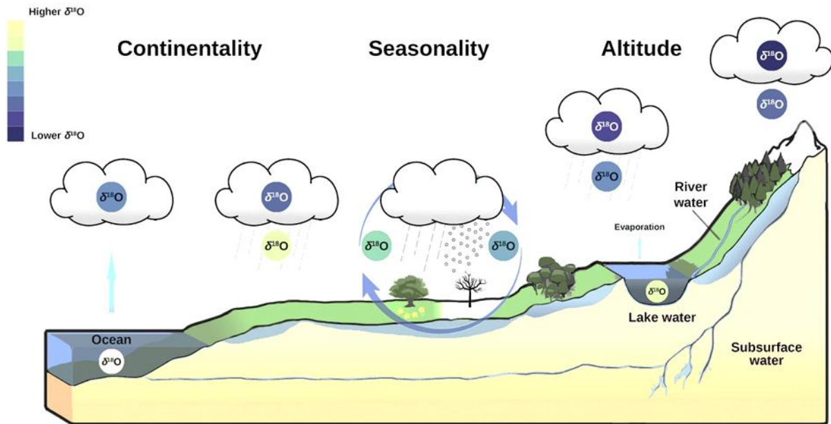
Figure 3.8 Diagram of the Rayleigh fractionation system and the variables that will affect \delta^{18}\text{O} values in evaporation, condensation, and precipitation (Pederzani and Britton 2019: 79). Open Access.
