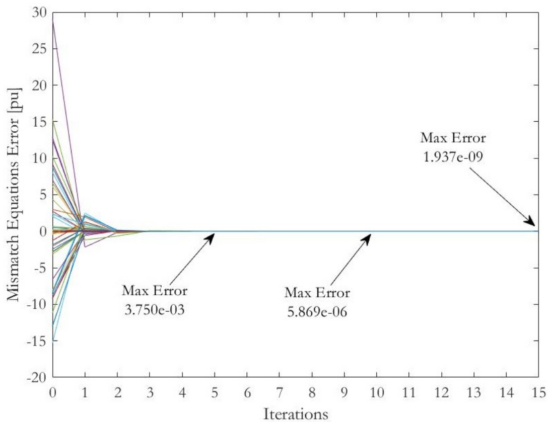
Figure 4.9: Modified Pegase Convergence for all State Variables
