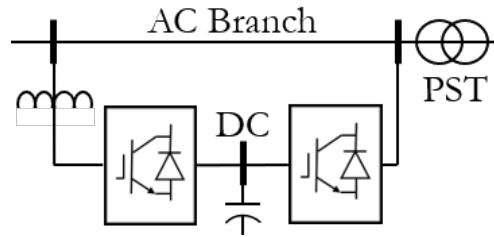
Figure 3.8: UPFC schematic representation using in-models
