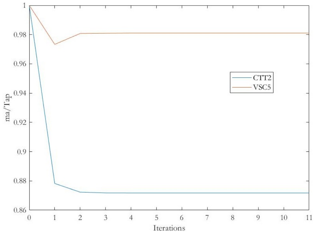
Figure 4.7: Modified IEEE 30 Modulation amplitude for Vt control
