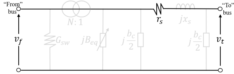
Figure 3.3: DC Branch in-model
