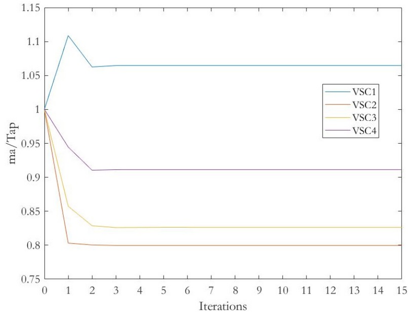
Figure 4.11: Modified PEGASE Modulation amplitude for Vt control
