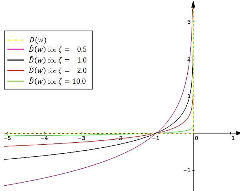
Figure A.1: Indicator D and approximation \hat{D} functions for different values of \zeta
