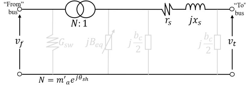
Figure 3.4: Transformer in-model
