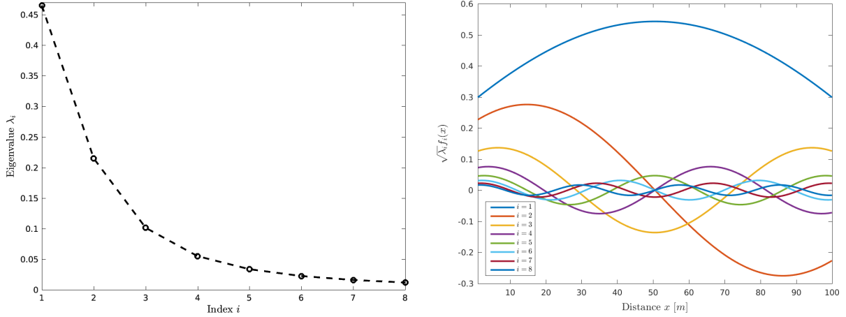
Figure 5.3: Eigenvalues (left plot) and associated eigenfunctions (right plot) of the correlation matrix in the KL decomposition for the dam-break problem over a flat bed.
