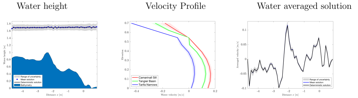
Figure 6.16: Uncertainty range in the water level (left plot), velocity profiles (middle plot) and averaged water velocity (right plot) for the flow recirculation in the Strait of Gibraltar.
