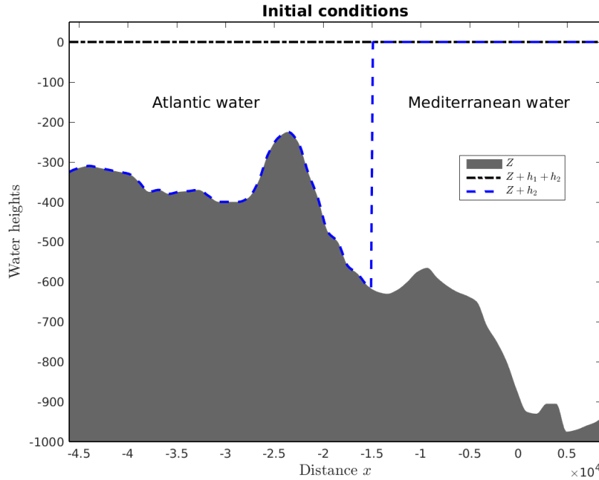
Figure 5.15: Initial conditions for the flow exchange through the Strait of Gibraltar.
