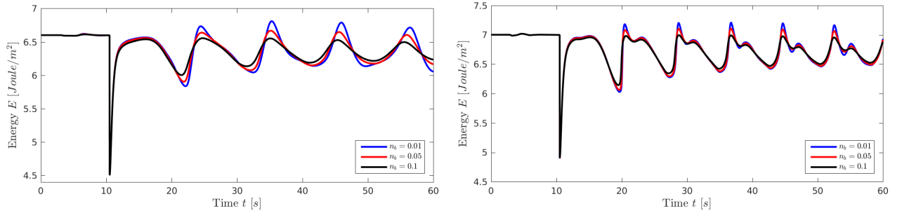
Figure 3.13: Time evolution of the hydraulic energy for free-surface flow problem over a deformable bed using different Manning coefficients with \beta = \frac{\pi}{5} (left) and \beta = \frac{\pi}{10} (right).
