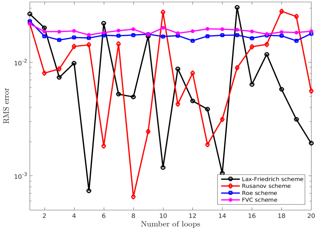
Figure 7.3: RMS errors for the bed reconstruction using different finite volume schemes.
