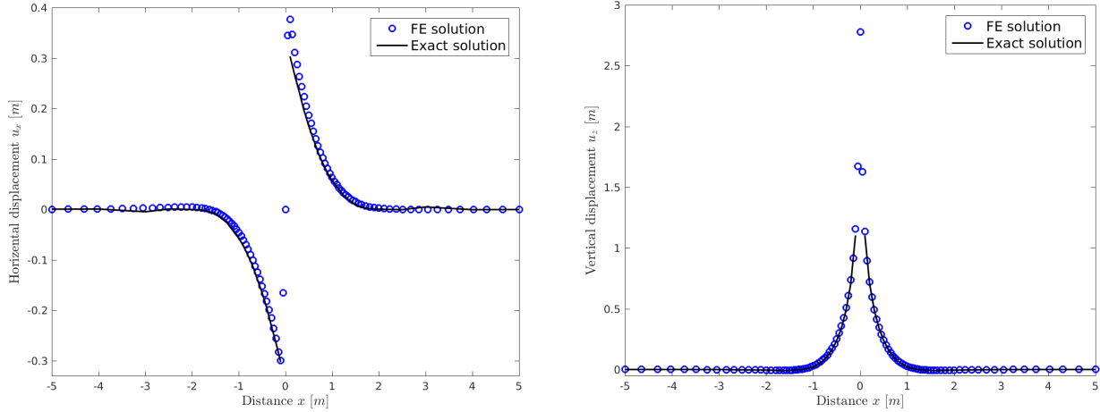
Figure 4.4: Horizontal displacement (left) and vertical displacement (right) obtained for the accuracy test example using the finite element method.
