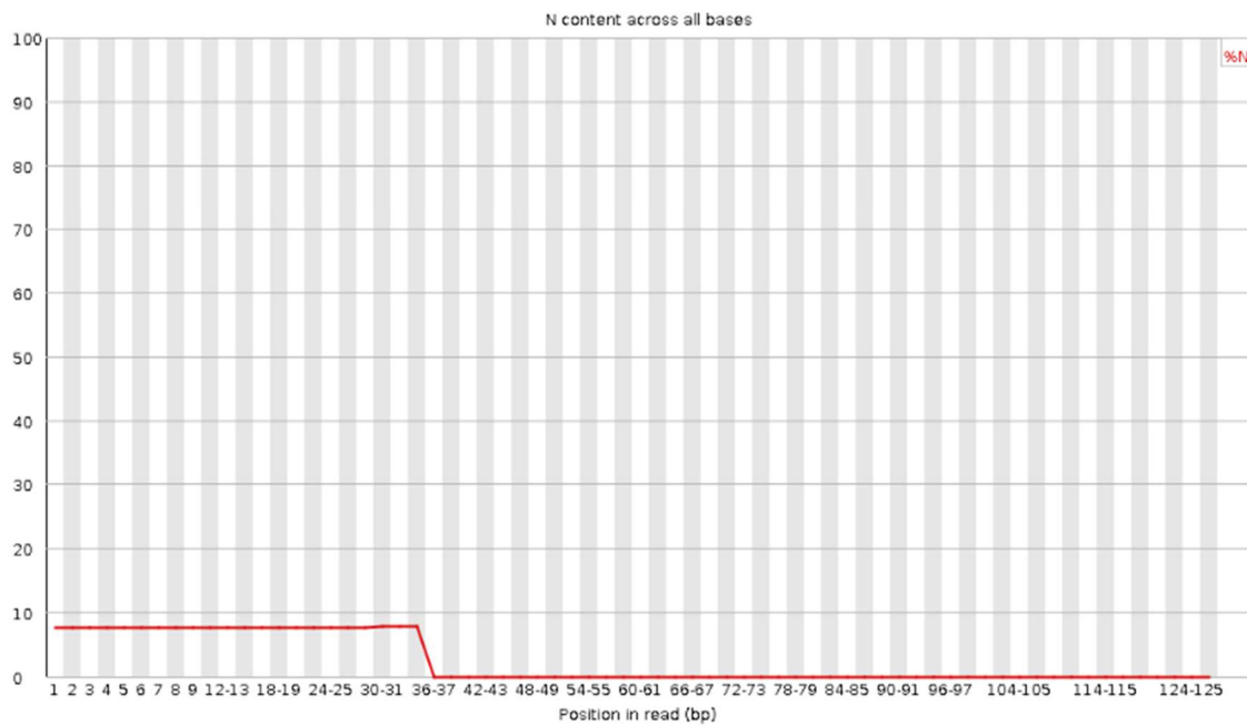
Figure 3.7, FastQC results showing the percentage of undetermined reverse sequences with an uncalled base in each base pair position.
