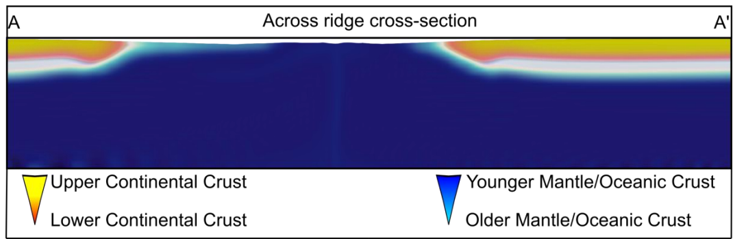
Figure A16 – Control experiment (Figure 4.3) cross sections. For cross-section locations refer to Figure A15.
