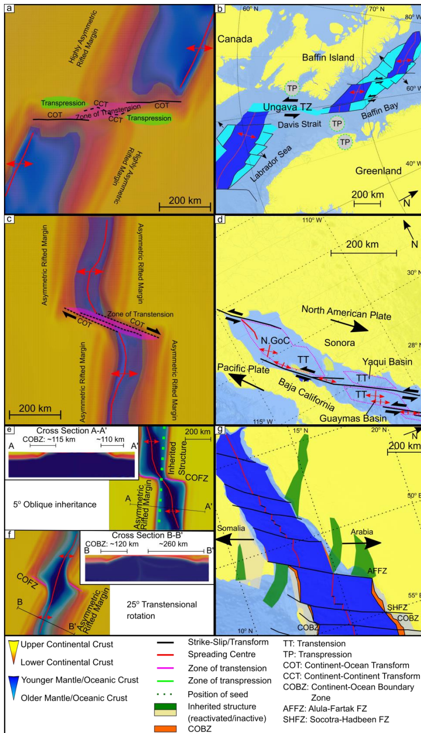
Figure 4.8 – Comparison with natural examples. a-b) Comparison of a -25^\circ transpressional rotated model snapshot at 20 (+5) Ma with the Davis Strait. Note the zones of compression/transpression within the outer corners of the continent-ocean transforms shown in green; in the natural example, similar areas are indicated with grey circles marked TP (location of transpression from Peace et al., 2017). Also note the transtensional zone shown in pink between the two segments of the COT due to the nature of the rotation. c-d) Comparison of a 5^\circ transtensional rotated model snapshot at 10 (+5) Ma with the Gulf of California. Note the zone of transtension in the model
