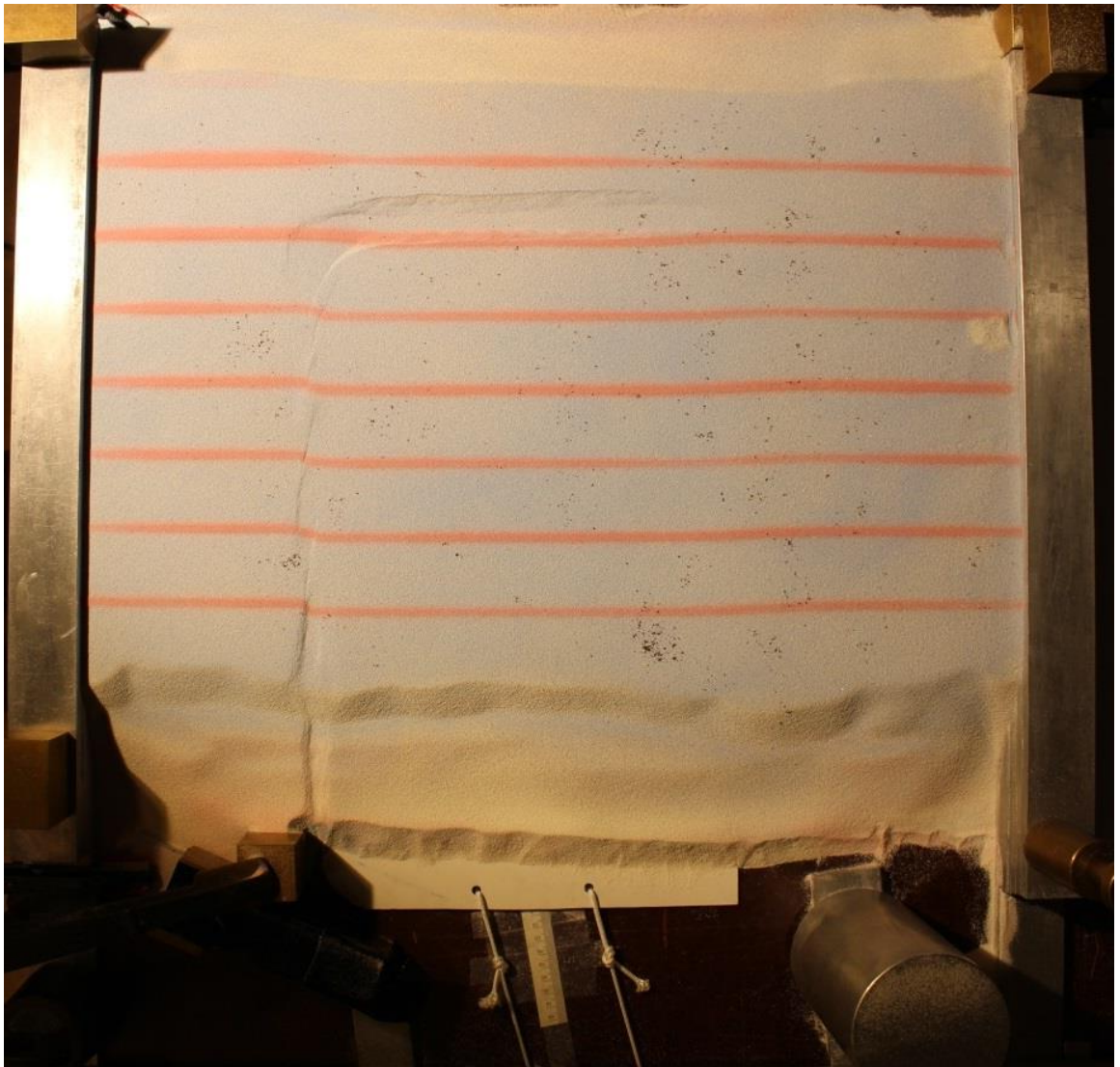
Figure B9 – Top view of Experiment 4 at the end of orthogonal rifting, without interpretation.
