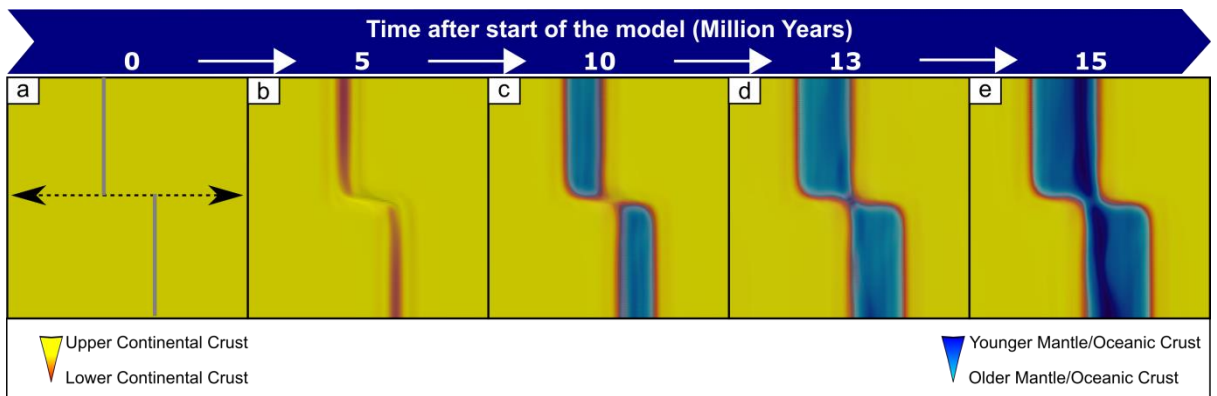
Figure A14 – Uninterpreted version of Figure 4.3 in the thesis.
