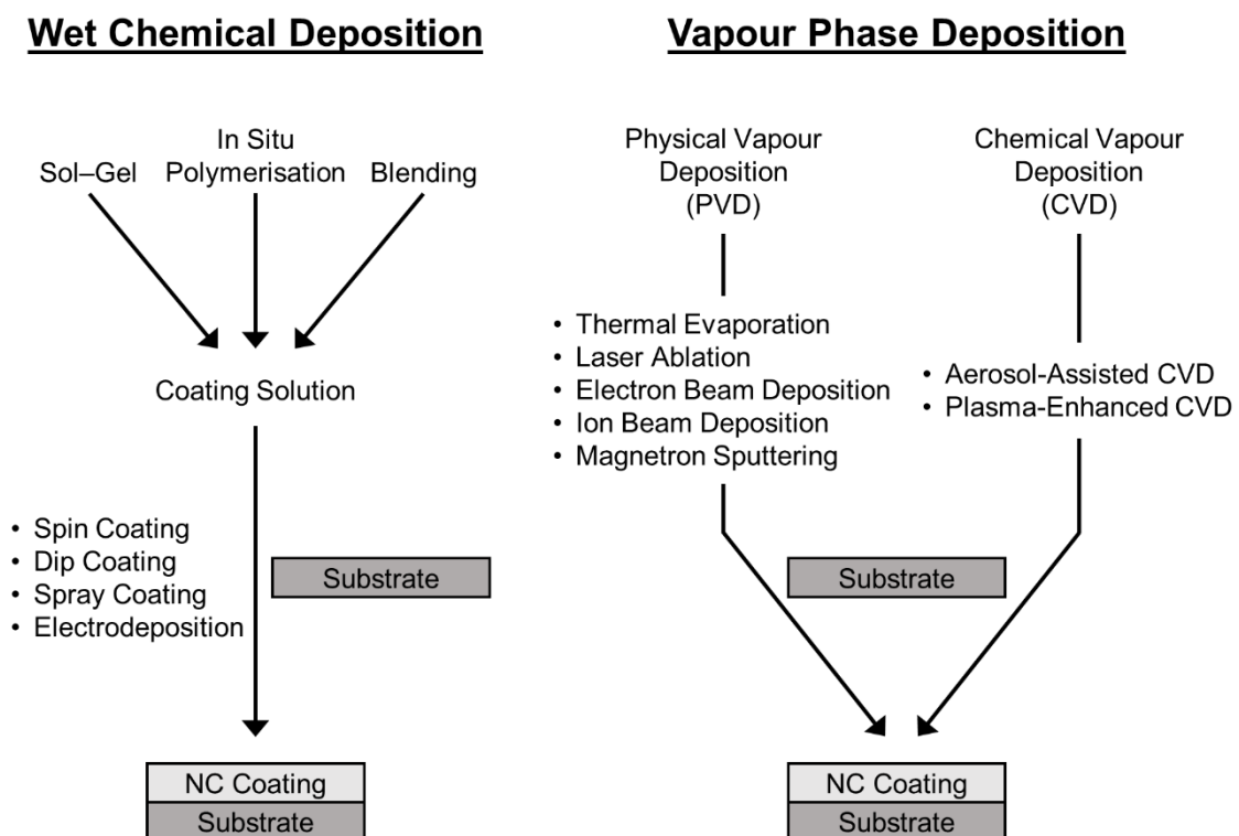
Figure 1.3: Overview of the main fabrication methods for the preparation of nanocomposite (NC) coatings.
