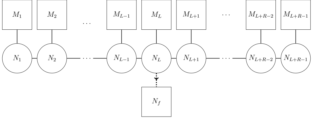
Figure 5.2: Quiver diagram for a generic gauged SMM from the brane construction.
