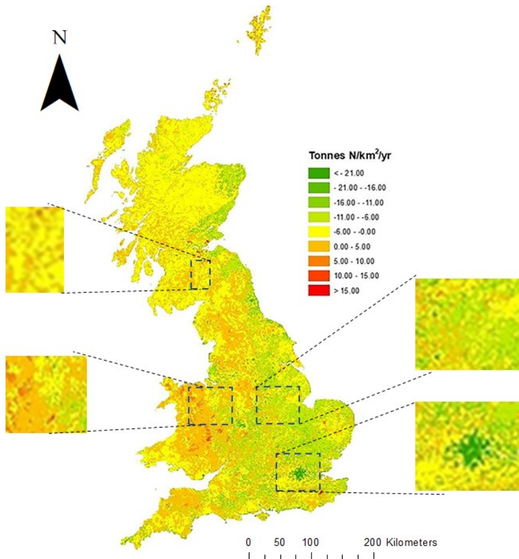
Figure 2.15: Calculated Total Nitrogen Budget of Great Britain at 1 km 2 for 2015
