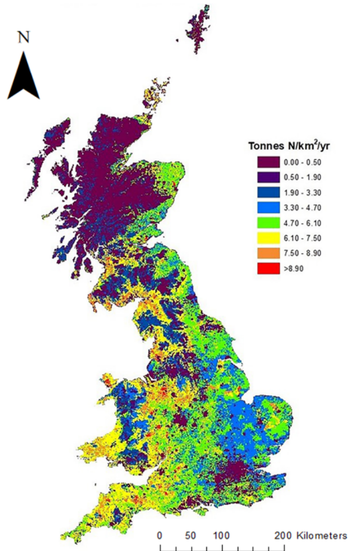
Figure 2.7: Calculated Atmospheric Nitrogen Emission for 2015.
