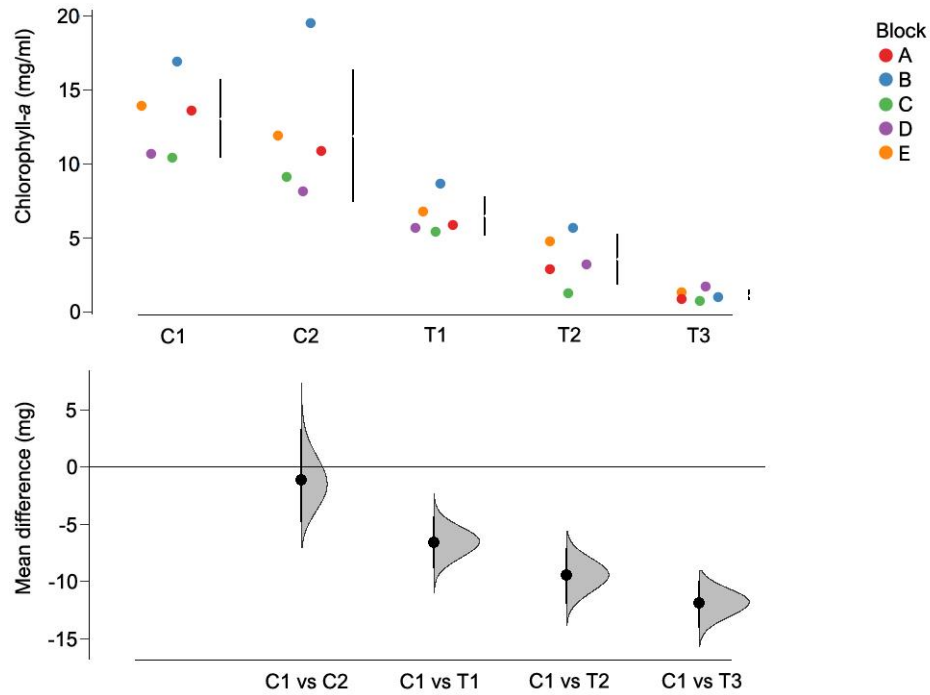
FIGURE 2.14 Impact of signal crayfish, in terms of effect sizes, on chlorophyll- \alpha levels in different groups ( C_1 , control without fish or crayfish; C_2 , bullhead control; T_1 , T_2 and T_3 are low, medium and high crayfish density treatments respectively), compared to first control ( C_1 ). Dots and vertical bars next to dots (on the right of each group) in the upper panel represent data points and mean ( \pm SD) error bars. Mean values are indicated by the gaps in the lines. Lower panel represents the mean difference (the effect size) and its 95% confidence interval (95% CI) as a point estimate and vertical bar respectively.
