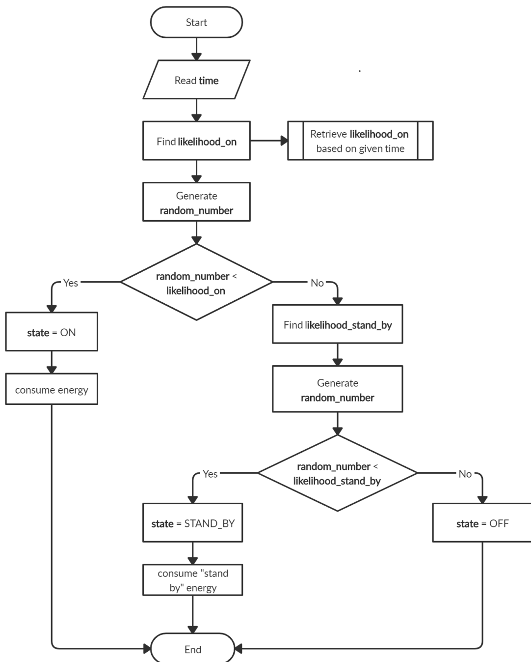
Figure 5.3: Flowchart of agent step method.
