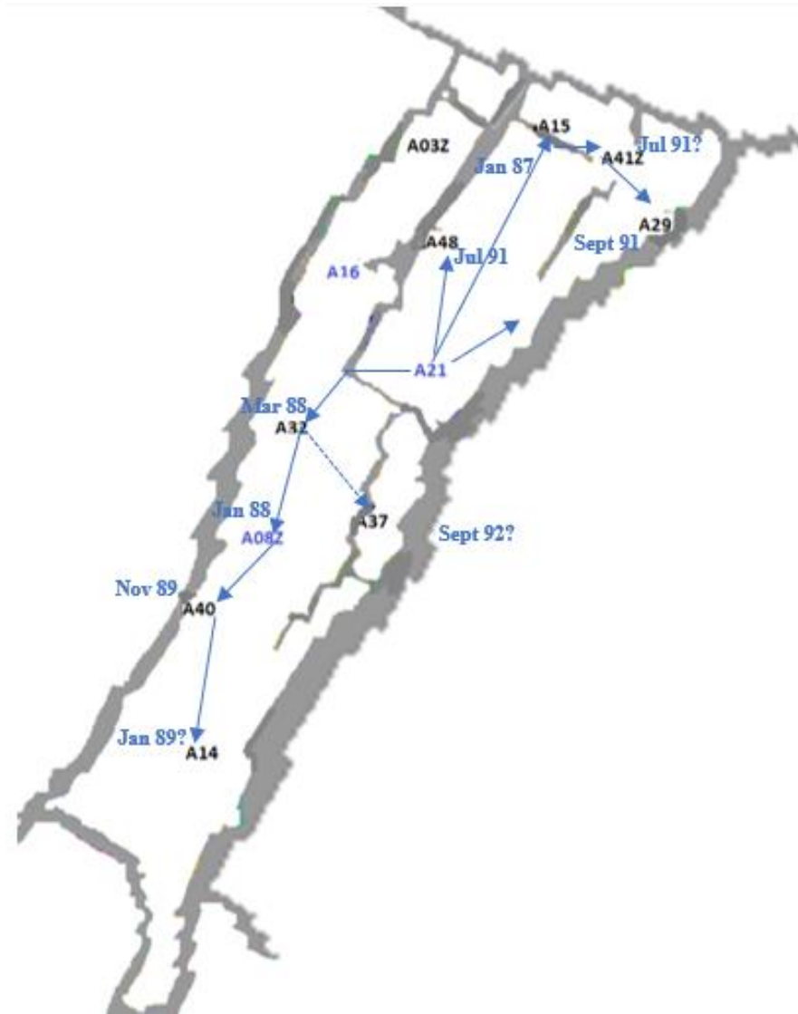
Figure 100- Water Injection Paths of A21, with Water Breakthrough Dates
