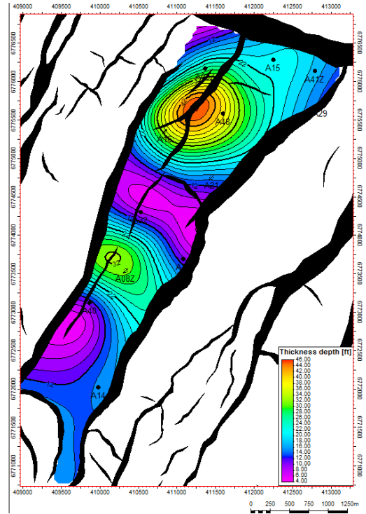
Figure 20- Isopach Map of LNE, Lower Ness Formation
