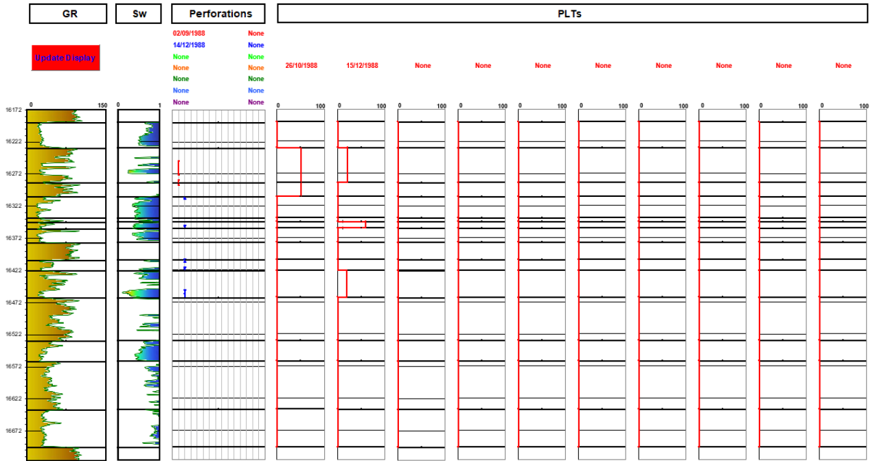
Figure iii)i - A37 PLT
