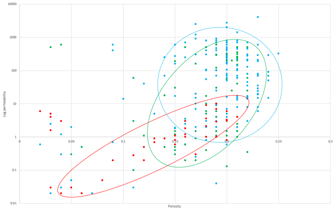
Figure 35- Porosity and Permeability of Reservoir Sandstone Facies Associations
