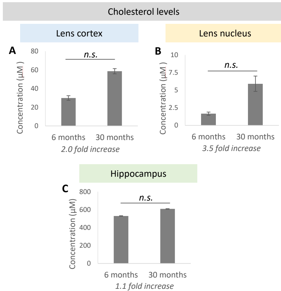
Figure 7.3: LC-MS quantification of cholesterol concentration in the eye lenses and hippocampi of 6 and 30 month-old mice. 20 \mu\text{M} of cholesterol-d6 was added as the internal standard and was subsequently used to calculate the concentration ( \mu\text{M} ) of cholesterol in the samples. A) Cortical fraction of the eye lens, B) nuclear fraction of the eye lens and C) hippocampus. General Linear Model Analysis of Variance followed by Tukey pairwise comparison post hoc test using time and location as independent factors and concentration as dependent factor was applied for statistical analysis, *p < 0.05 n = 3 for hippocampus and n = 2 \times 8 pooled eye lenses, n.s.: not significant.
