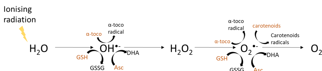
Figure 8.1: Scheme of free radicals generated by ionising radiation and the non-enzymatic anti-oxidants that can neutralise them. GSH, \alpha -toco and Asc convert OH^\bullet into H_2O_2 while being oxidised to GSSG, \alpha -toco radical and DHA respectively. GSH, \alpha -toco, Asc and carotenoids convert O_2^\bullet into O_2 while being oxidised to respectively GSSG, \alpha -toco radical, DHA and carotenoids radicals. \alpha -toco: \alpha -tocopherol, \alpha -toco radical: \alpha -tocopheryl radical, GSH: glutathione, GSSG: glutathione disulphide, Asc: ascorbic acid and DHA: dehydroascorbate anion
