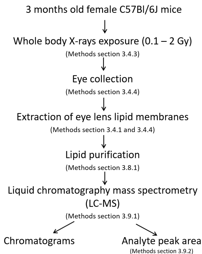
Figure 6.2: Schematic representation of the experimental design of the in vivo IR-induced oxysterol formation analysis. Section numbers refer to the material and methods chapter section in which the protocol was described.
