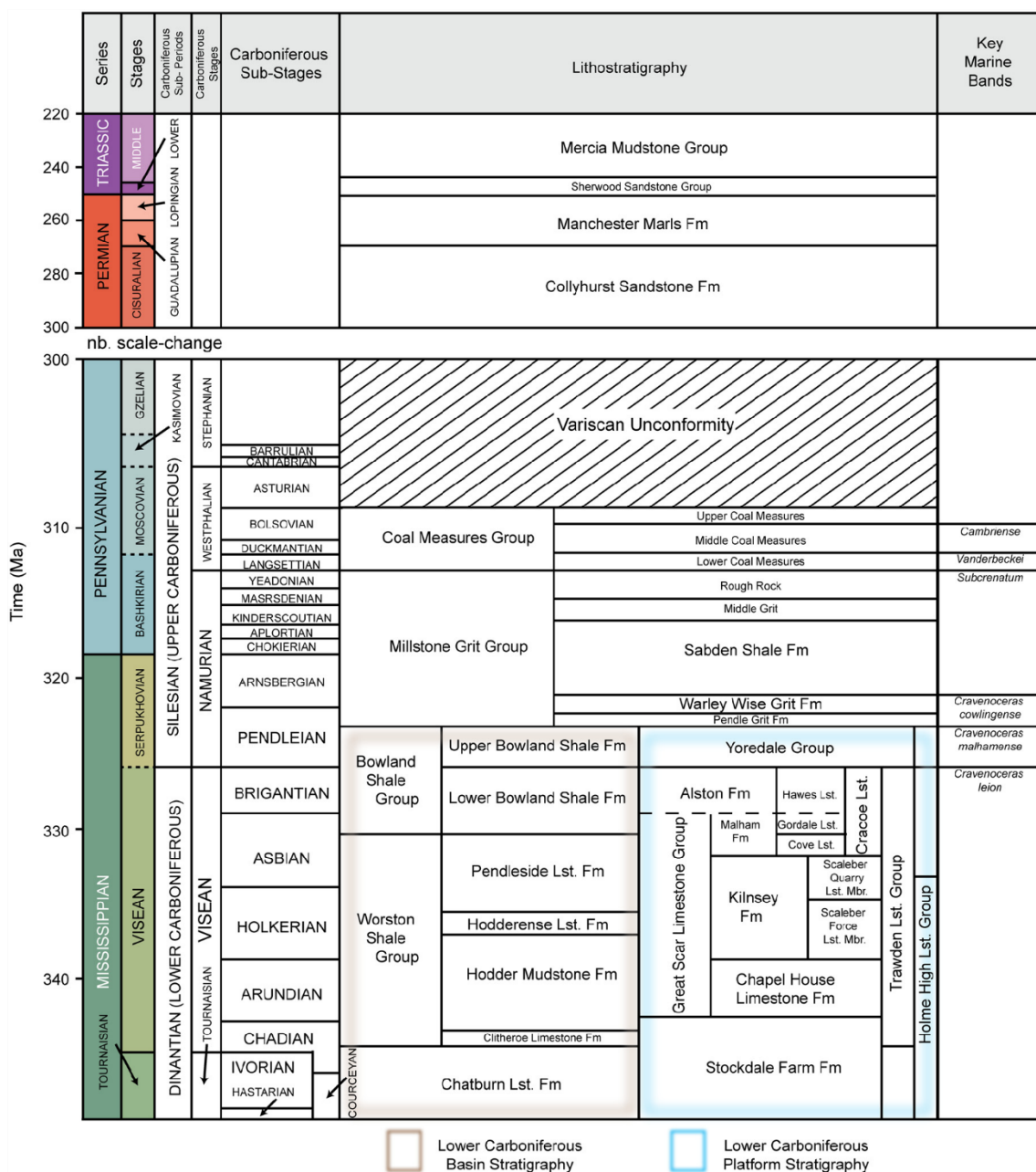
Figure 1.12 Stratigraphic chart for the Carboniferous, Permian and Triassic sequences of northwest England. Image adapted from Anderson and Underhill [2020].
