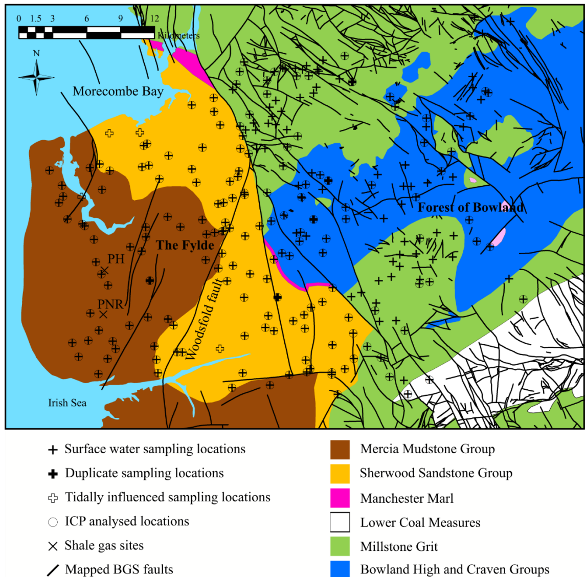
Figure 5.2 Map of the study region showing surface water sampling locations with respect to underlying bedrock geology and faults mapped by the BGS. PH and PNR are the shale gas fracking sites of Preese Hall and Preston New Road, respectively. Contains BGS data © Crown copyright and database right (2019). A BGS/EDINA supplied service.
