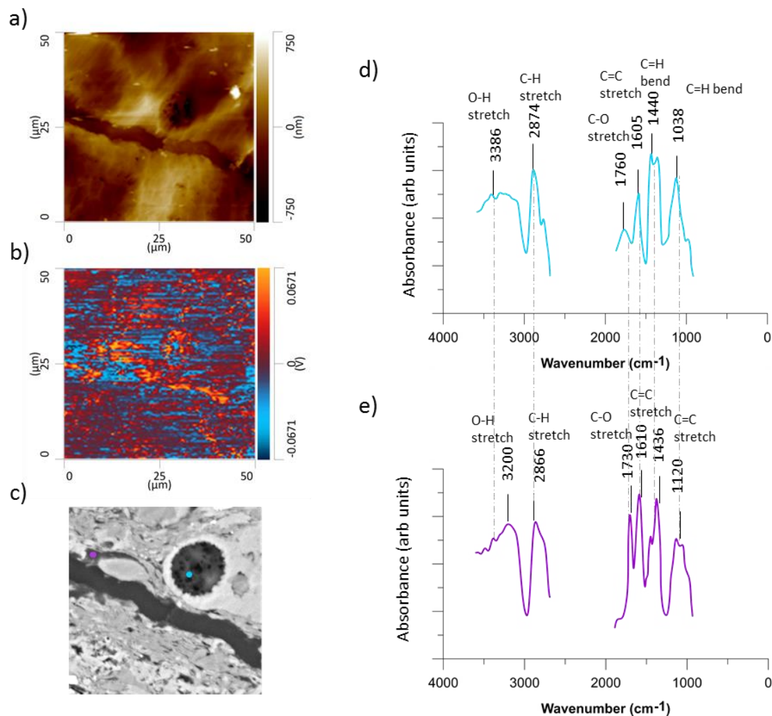
Figure 5.24: AFM-IR experiments on a polished surface of sample GW3 ( R_0 1.2%). a) is a topographic map of the analysed area, taken simultaneously to b) which is the frequency map at the set wavenumber of 2920\text{ cm}^{-1} . c) is the corresponding area under the SEM and d) the IR spectrum of bitumen, indicated in the SEM image with the colour celeste and e) the IR spectrum of an inertinite, indicated in the SEM image with the colour purple. The dots on the SEM image correspond to the points where the spectra were acquired.
