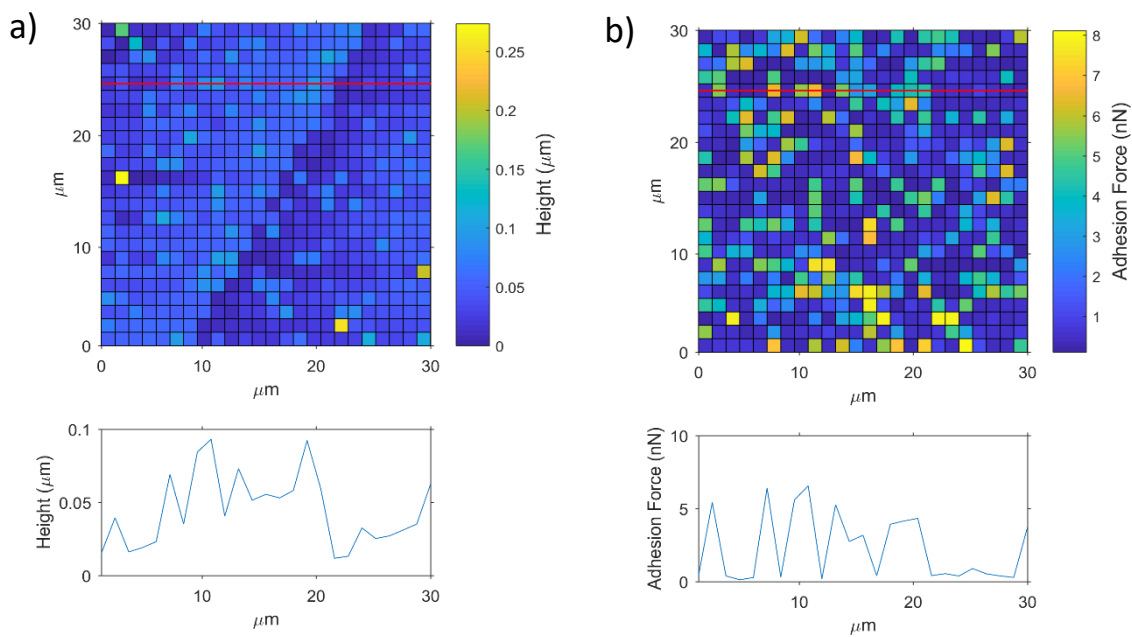
Figure 4.11: a) Topography and b) corresponding adhesion map of area 01 on calcite surfaces aged in dodecane. At the bottom of each map, the cross-section profile taken across the red line in the maps.
