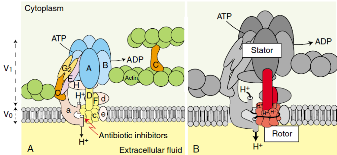
Figure 1.2 Model of the eukaryotic V-ATPase proton pump expressed in a cell membrane. (A) Molecular model. The cytosolic V_1 complex consists of eight different subunits identified with uppercase letters (A-H), G exists as a dimer G_2 . The integral membrane bound V_0 complex is made up of four different subunits identified with lowercase letters (a,c,d,e). Subunit c and its isoforms form a hydrophobic proton binding ring. (B) Mechanistic model. V_0 is connected to V_1 by a central rotating shaft (D and F) and a peripheral stationary shaft (C, E, G, H and a). The rotor consists of the central rotating shaft and the c-ring of V_0 (red) the remaining subunits make up the stator (grey). Hydrolysis of ATP drives rotation of the rotor. Subunit a provides two half proton channels which are offset, rotation of the c-ring moves protons from one channel to the other (Beyenbach and Wieczorek, 2006).
