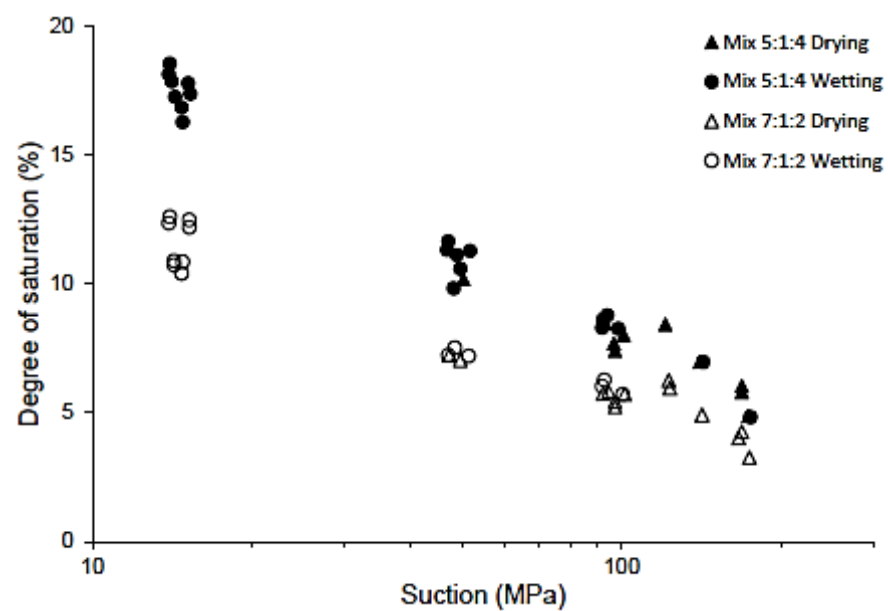
Figure 2.3: Drying curves for coarse earth Mix 7:1:2 and fine earth Mix 5:1:4 (after Beckett and Augarde, 2012).
