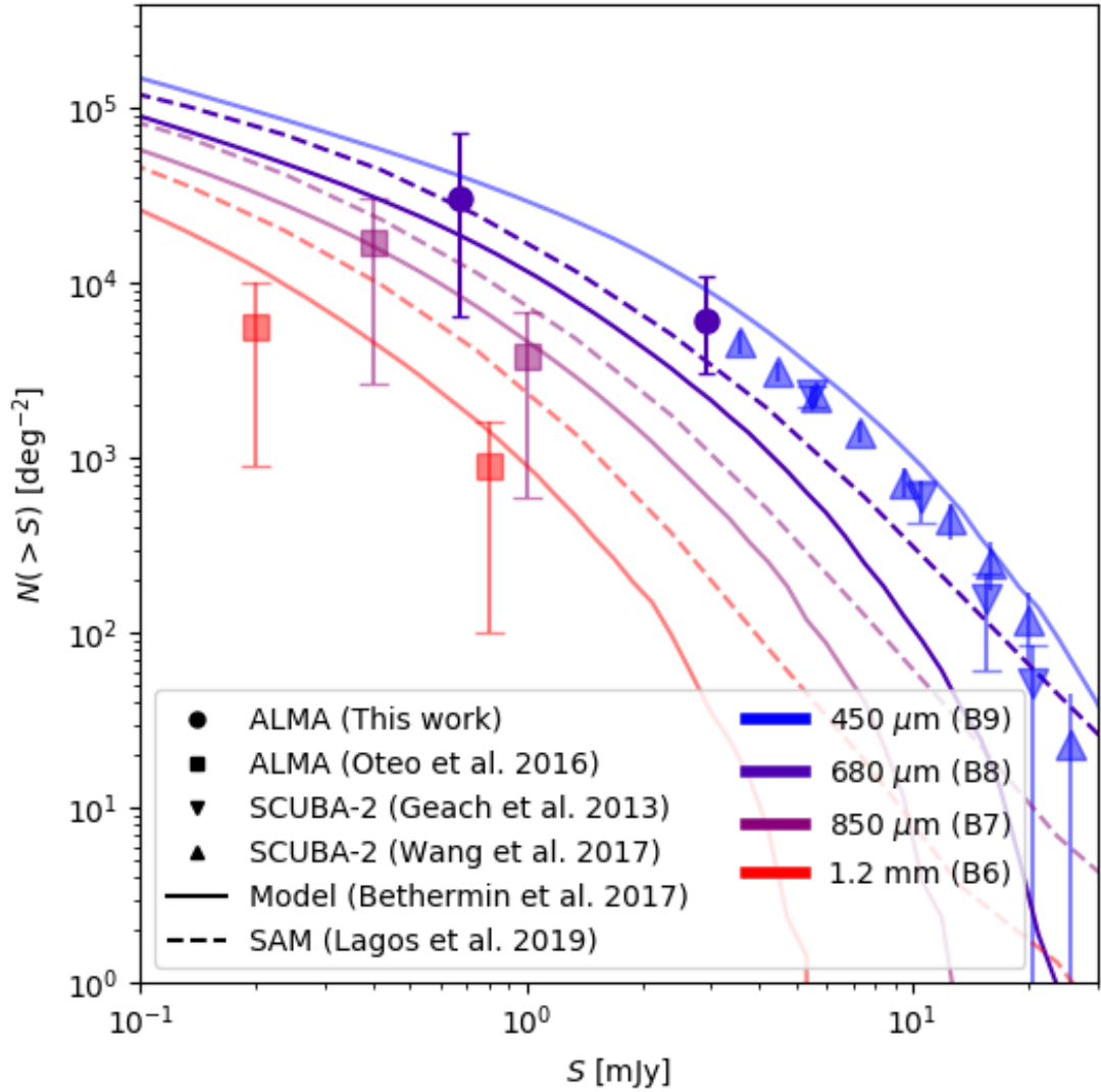
Figure 7.10: Cumulative number counts of DSFGs at 680 \mu\text{m} (in ALMA Band 8, at 440 \text{ GHz} ). For comparison we show number counts from observations at different wavelengths as well as predictions from an empirical and semi-analytical model (B  thermin et al., 2017; Lagos et al., 2019). We use those models to calculate a model prediction for the number counts at 680 \mu\text{m} by linearly interpolating between the 500 \mu\text{m} and 850 \mu\text{m} number count models. The number counts reported by Geach et al. (2013) are shifted by -2.5 \text{ mJy} to the low flux end of the bin.
