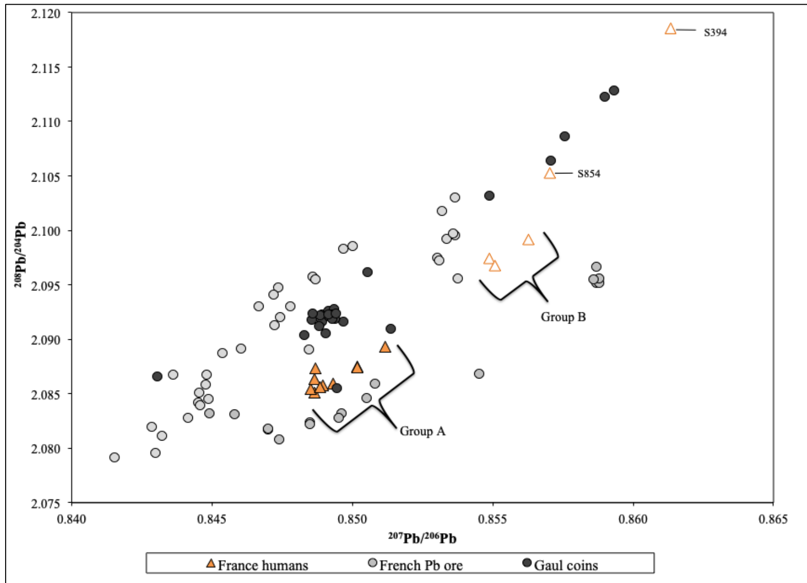
Figure 8.6 –Plot of ^{208}\text{Pb}/^{206}\text{Pb} versus ^{207}\text{Pb}/^{206}\text{Pb} showing the relationship between France tooth enamel samples and the France lead ore field. Ore data taken from Butcher and Ponting, (2014) and OXALID. Analytical error is within the symbols
