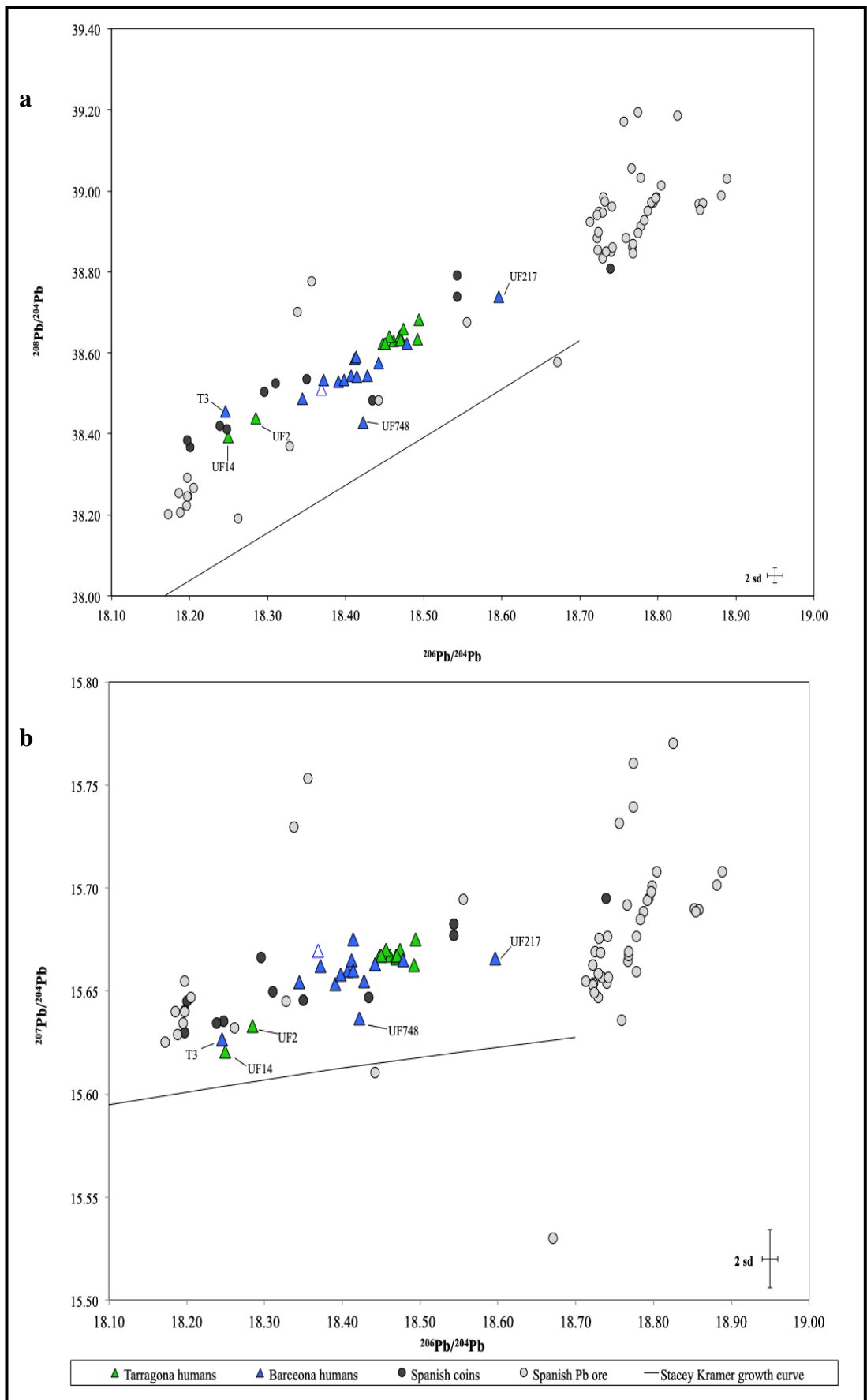
Figure 8.9 –Plots of ^{208}\text{Pb}/^{204}\text{Pb} versus ^{206}\text{Pb}/^{204}\text{Pb} (a) and ^{207}\text{Pb}/^{204}\text{Pb} versus ^{206}\text{Pb}/^{204}\text{Pb} (b) showing the relationship between Spain tooth enamel samples and the Spain lead ore field. Ore data taken from Butcher and Ponting (2014) and OXALID. Analytical error shown to 2 sd.
