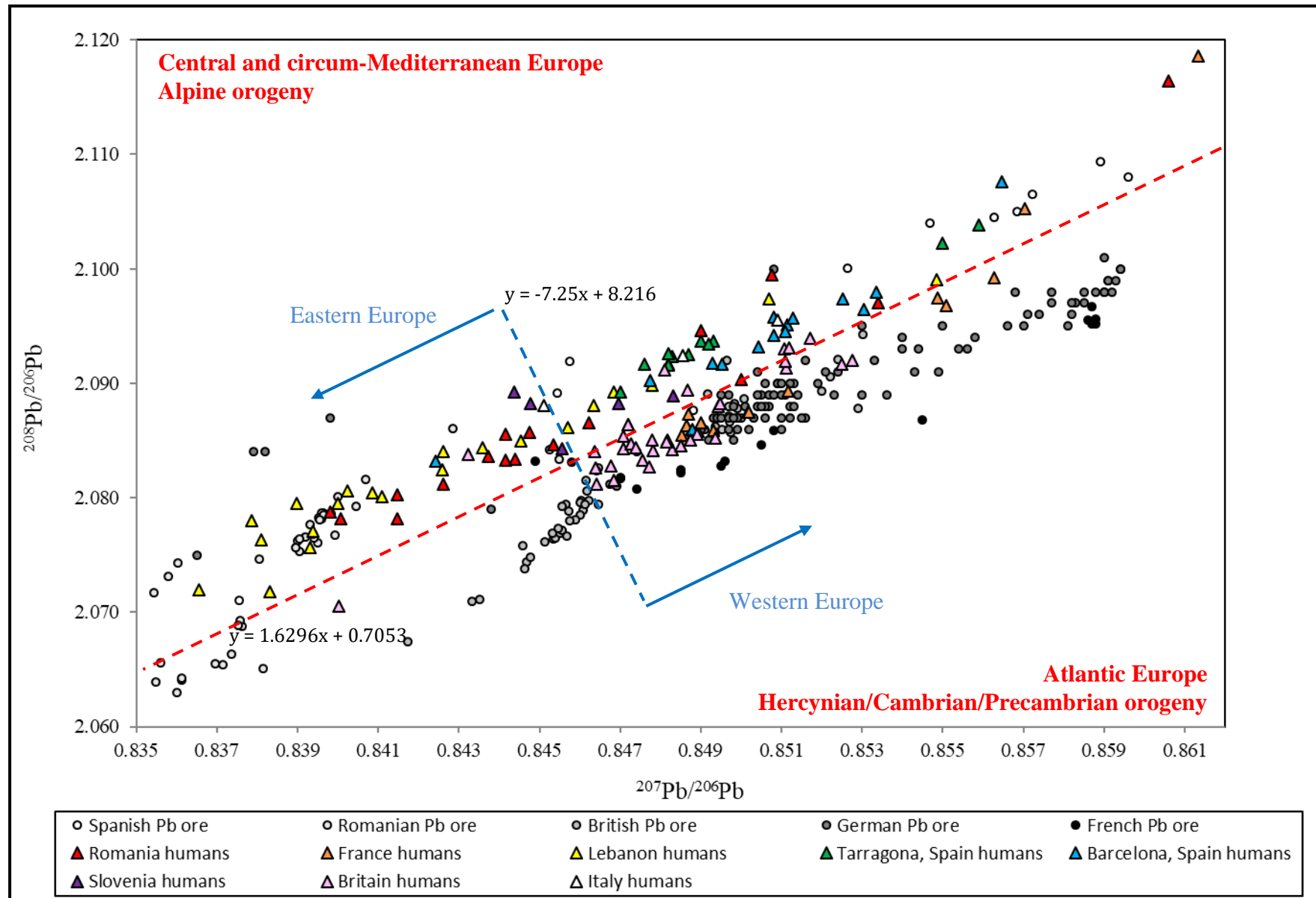
Figure 8.15 – Plot of ^{208}\text{Pb}/^{206}\text{Pb} versus ^{207}\text{Pb}/^{206}\text{Pb} showing how the tooth enamel samples and lead ore data group according to orogenic age and region of Europe (east vs. west). Analytical error is within the symbols
