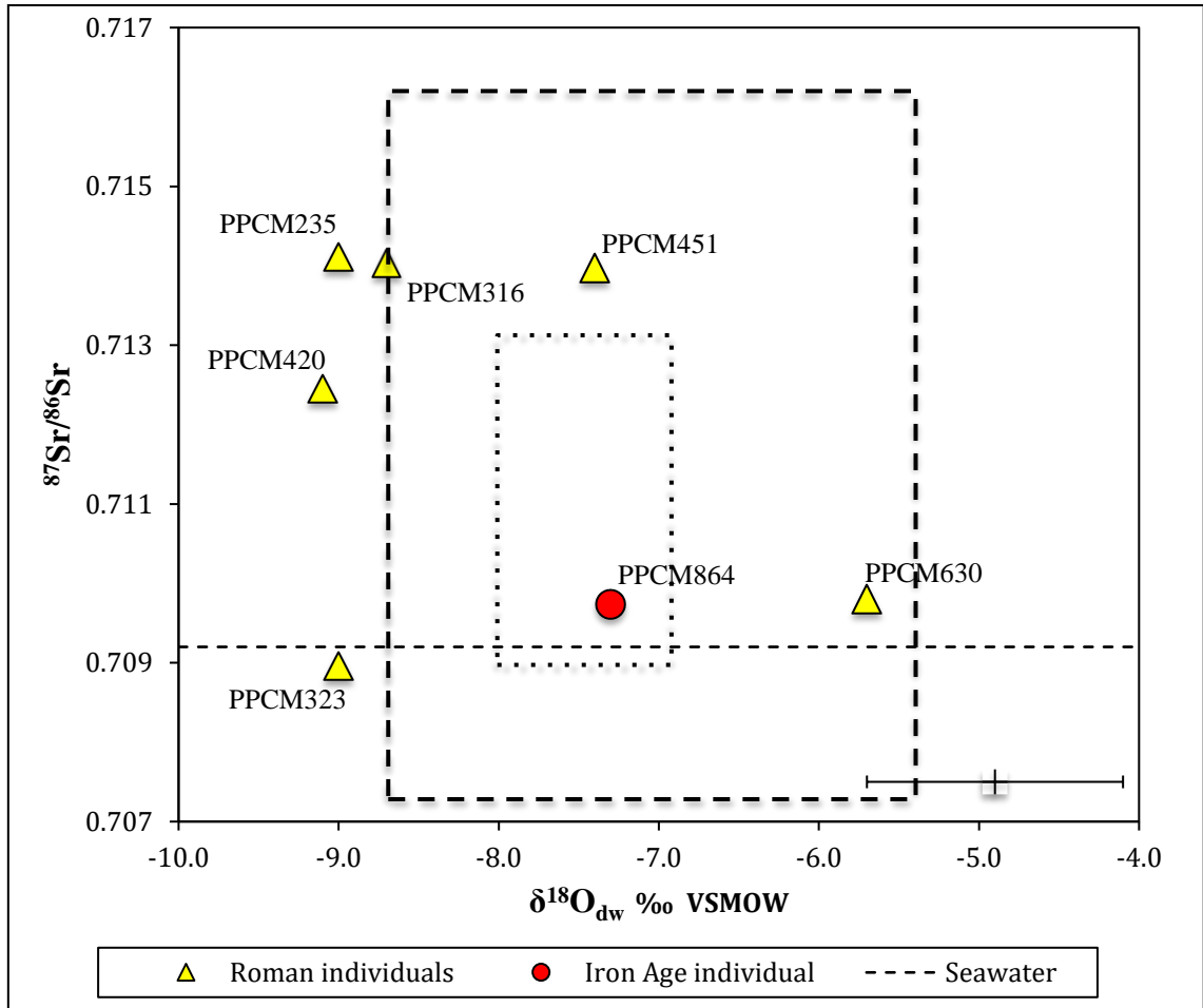
Figure 8.34 – ^{87}\text{Sr}/^{86}\text{Sr} and \delta^{18}\text{O}_{\text{dw}} values for enamel samples from the Musselburgh Roman ( n = 6 ) and Iron Age ( n = 1 ) individuals. Also showing the estimated range of UK \delta^{18}\text{O}_{\text{dw}} (mean -7.4 \pm 1.7\text{‰} , 2\sigma ) and ^{87}\text{Sr}/^{86}\text{Sr} (0.7078 - 0.7165) values (dashed box) obtained from previous archaeological studies (Evans et al., 2012b) as well as the estimated ^{87}\text{Sr}/^{86}\text{Sr} and \delta^{18}\text{O}_{\text{dw}} range for the Lothian area (dotted box) according to (Darling and Talbot, 2003). ^{87}\text{Sr}/^{86}\text{Sr} 2\sigma errors are within the symbol
