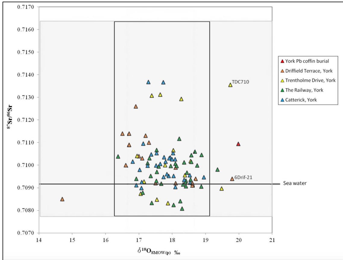
Figure 8.31 – Bivariate plot showing ^{87}\text{Sr}/^{86}\text{Sr} against \delta^{18}\text{O}_{\text{vSMOW(p)}} . The black box represents the UK range for \delta^{18}\text{O}_{\text{vSMOW(p)}} ( \pm 2 sd) and the shaded area represents the UK range for ^{87}\text{Sr}/^{86}\text{Sr} (Evans et al., 2012). Comparative Roman York data from: Driffield Terrace (Müldner et al., 2011); Trentholme Drive and The Railway (Leach et al., 2009); Catterick (Chenery et al., 2011).
