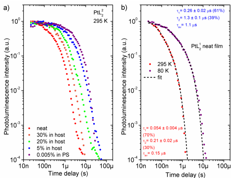
Figure 6.3. a) Photoluminescence decay of PtL_2 in OLED host (mCP:OXD7 80:20), polystyrene matrix (PS) and neat film at 295 K. The percentage represents weight concentration of the emitter in the chosen matrix. b) Photoluminescence decay of a neat film of PtL_1 at 295 K and 80 K. \lambda_{exc} = 355 \text{ nm}
