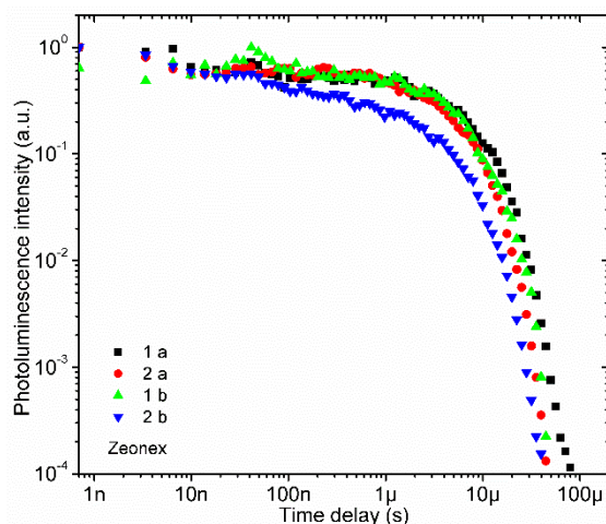
Figure 5.3. Photoluminescence decay of 0.1 % Zeonex films at 295 K, \lambda_{\text{exc}} = 355 \text{ nm} .
