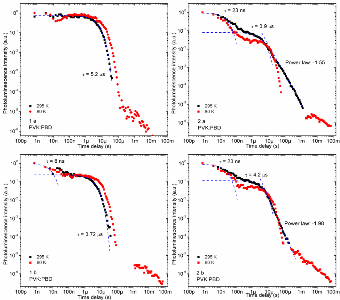
Figure 5.5. Photoluminescence decay of PVK:PBD (60:40) doped films at 295 and 80 K, \lambda_{exc} = 355 nm. Decay at 295 K is fitted with monoexponential and power law expressions. Power law expression used for fitting: y = ax^b , where a and b are fitting parameters, while x is time and y is photoluminescence intensity. “Power law:” denotes the exponent b of the fit. Note: error limits not available.
