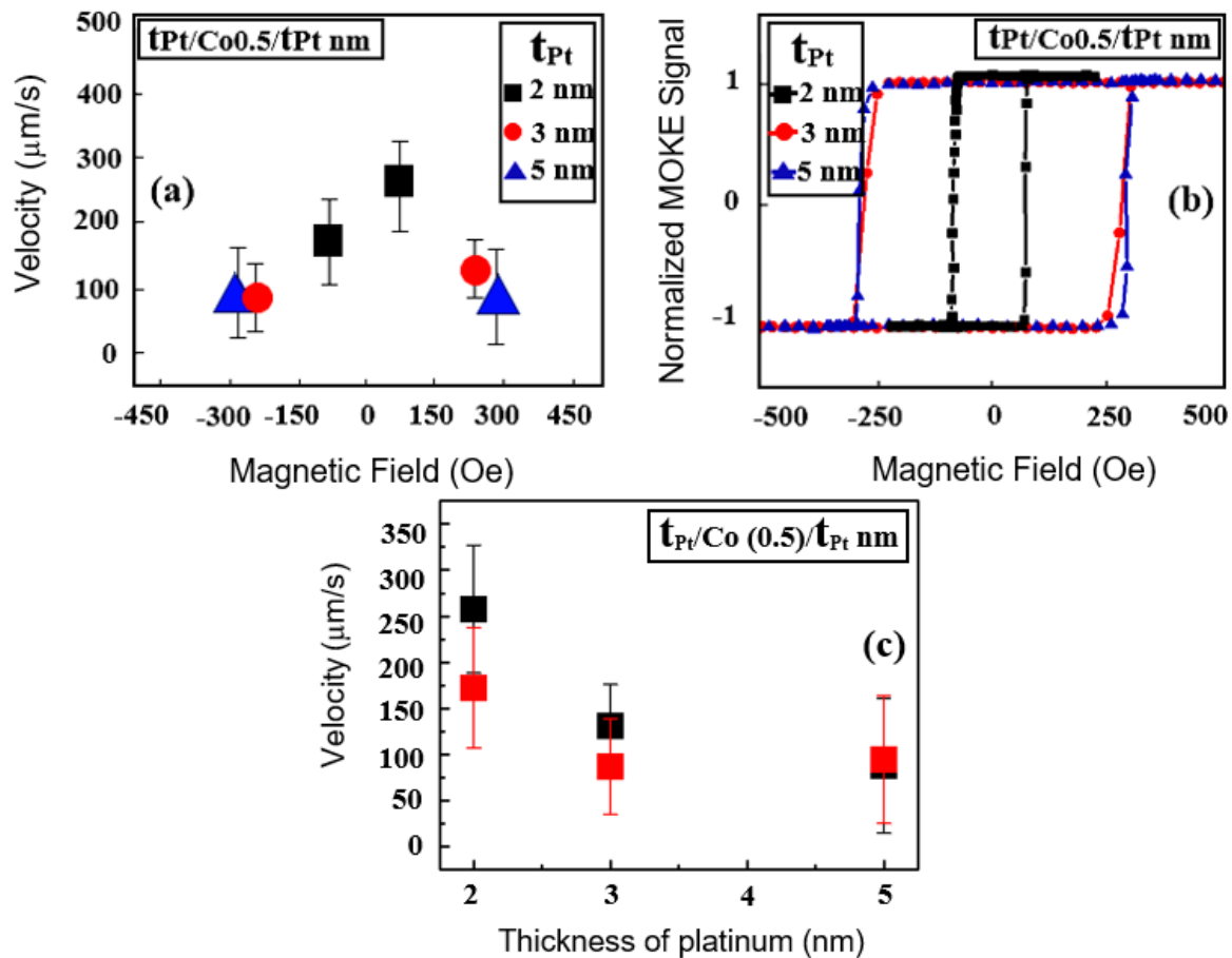
Fig. 8.8 a. Domain wall velocity of a t_{Pt}/t_{Co} (0.5)/t_{Pt} nm multilayers as a function of magnetic field. b. coercivity of a t_{Pt}/t_{Co} (0.5)/t_{Pt} nm multilayers as a function of magnetic field in (Oe). c. Domain wall velocity of a t_{Pt}/t_{Co} (0.5)/t_{Pt} nm multilayers as a function of thickness of platinum. The black and red symbols refer to the down-up and up-down reversal magnetization respectively.
