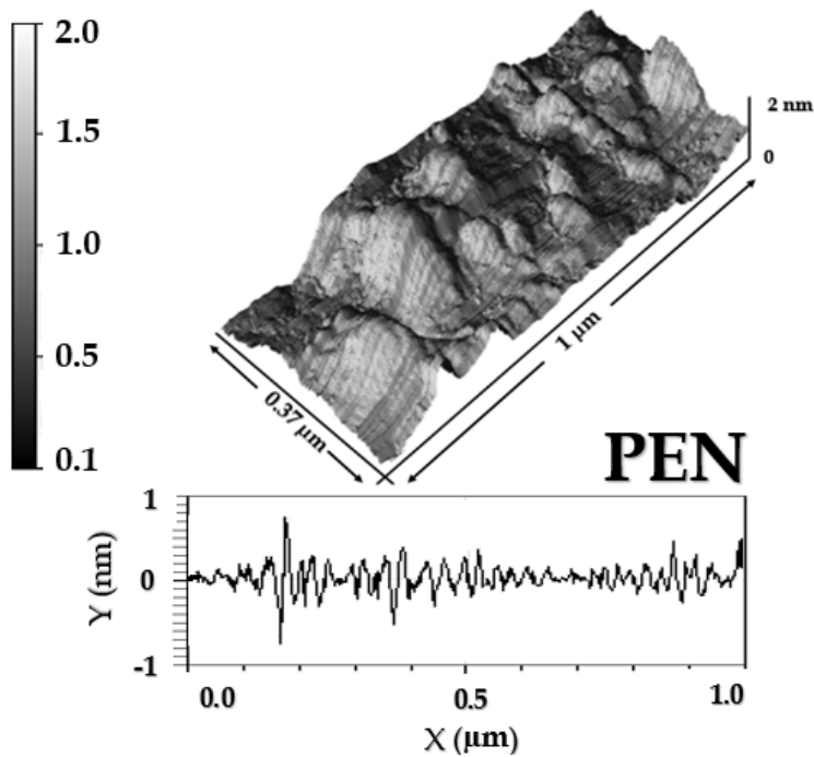
Fig. 6.6 Atomic force microscopy image of a Polyethylene Naphthalate substrate.
