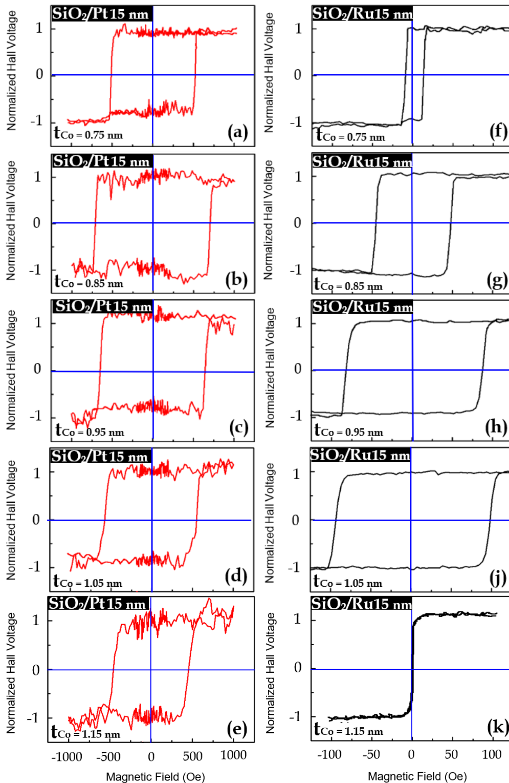
Fig. 7.9 Hysteresis loops for both Ru15.0/( t_{Co} )/Ru3.0 nm and Pt15.0/( t_{Co} )/Pt3.0 nm using SiO_2 substrate. Note different magnetic field scales for Pt and Ru data.
