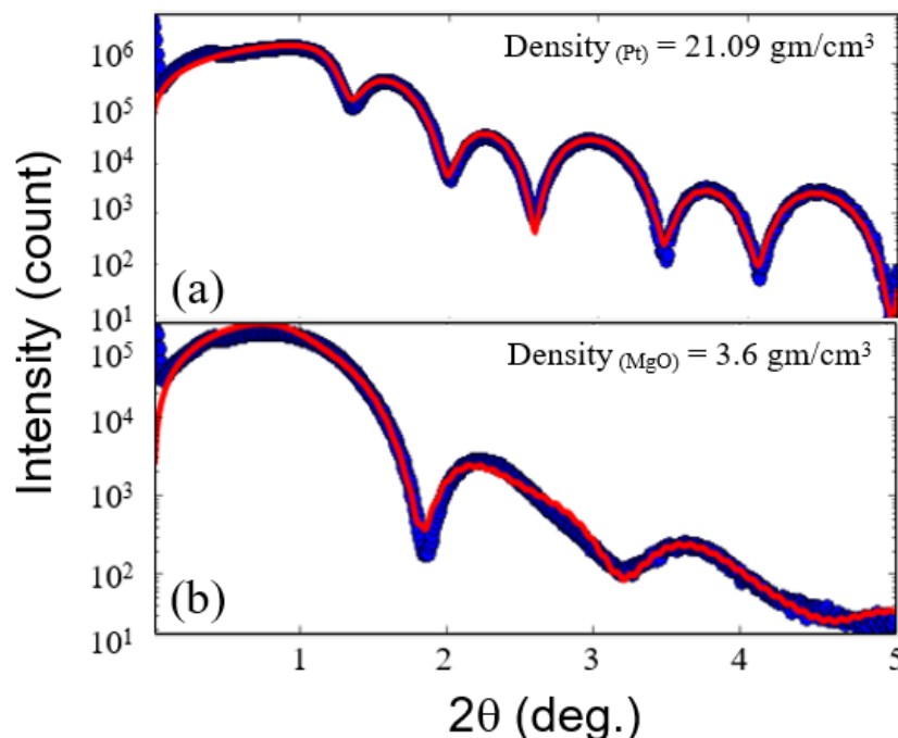
Fig. 5.6 X- ray reflectivity curves of different structure for both (a). t_{Pt}5.0/t_{Co}0.8/t_{Pt}5.0 nm and (b). t_{Pt}5.0/t_{Co}0.8/t_{MgO}5.0 nm respectively on SiO_2 substrates (film thickness 10.8 nm). The blue symbols indicate the measured data and the red lines the best fitting simulations.
