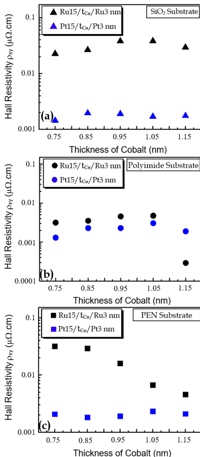
Fig. 7.16 (a,b,c) Hall resistivity for both Ru15.0/( t_{\text{Co}} )/Ru3.0 nm and Pt15.0/( t_{\text{Co}} )/Pt3.0 nm on SiO 2 , polyimide and PEN substrates respectively as a function of the cobalt thickness. The error bars are very small.
