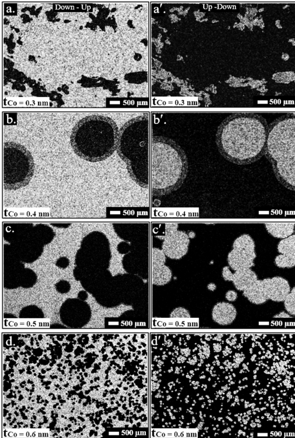
Fig. 8.1 MOKE images of the evolution of domain structure in the ultra thin cobalt as a function of Co thickness for t_{P1}5.0/t_{Co}/t_{P1}5.0 nm (a, a'), with H = +451 Oe and -334 Oe, (b, b'), with H = +169 Oe and -170 Oe, (c, c'), with H = +280.7 Oe and -278 Oe and (d, d'), H = +468 Oe and -464.9 Oe.
