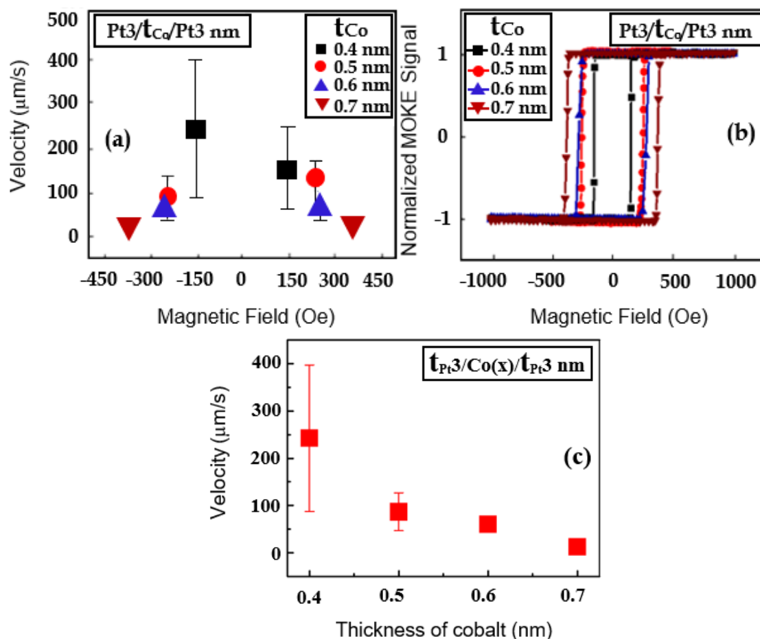
Fig. 8.6 a. Domain wall velocity of a t_{\text{Pt}} 3.0/t_{\text{Co}}/t_{\text{Pt}} 3.0 nm multilayers as a function of magnetic field. b. coercivity of a t_{\text{Pt}} 3.0/t_{\text{Co}}/t_{\text{Pt}} 3.0 nm multilayers as a function of magnetic field. c. Domain wall velocity of a t_{\text{Pt}} 3.0/t_{\text{Co}}/t_{\text{Pt}} 3.0 nm multilayers as a function of thickness of cobalt.
