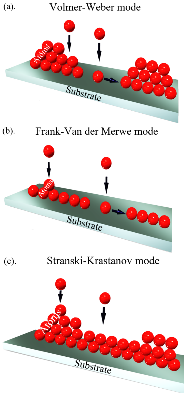
Fig. 3.3 Schematic illustration of the three film growth modes. The spheres is an atoms. Depending on the free energy contributions one finds (a) Volmer-Weber (VW), (b) Frank-van-der-Merwe (FvdM) and (c) Stranski-Krastanov (SK) growth.
