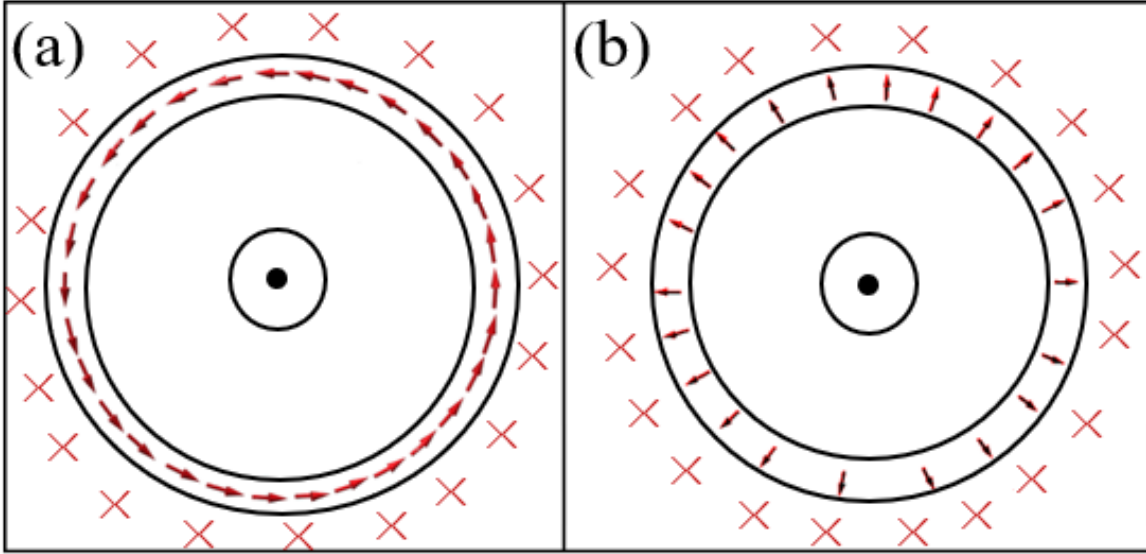
Fig. 2.8 Schematic configuration of a magnetic bubble. (a). [left] in case of bloch wall, the magnetization of the plane, which describes the domain wall between the circular bubble region ( magnetization is down) and the outer region (magnetization is up). (b). [right] same as in the left entry but the domain wall is a Néel wall.
