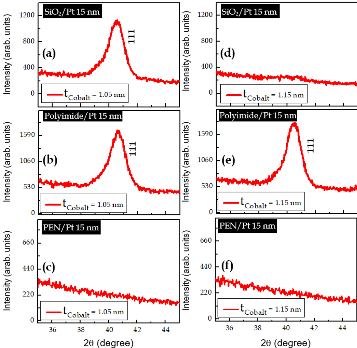
Fig. 7.18 (a,b,c). XRD patterns with 15 nm t_{Pt} with t_{Co} = 1.05 for SiO_2 , polyimide and PEN respectively. (d,e,f). XRD patterns with 15 nm t_{Pt} with t_{Co} = 1.15 for SiO_2 , polyimide and PEN respectively.
