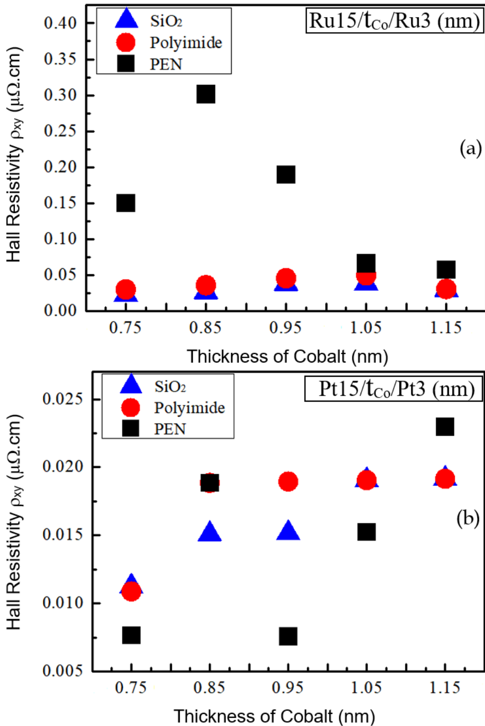
Fig. 7.17 (a,b) Hall resistivity for both Ru15.0/( t_{Co} )/Ru3.0 nm and Pt15.0/( t_{Co} )/Pt3.0 nm on SiO 2 , polyimide and PEN substrates respectively as a function of the cobalt thickness. The error bars are very small.
