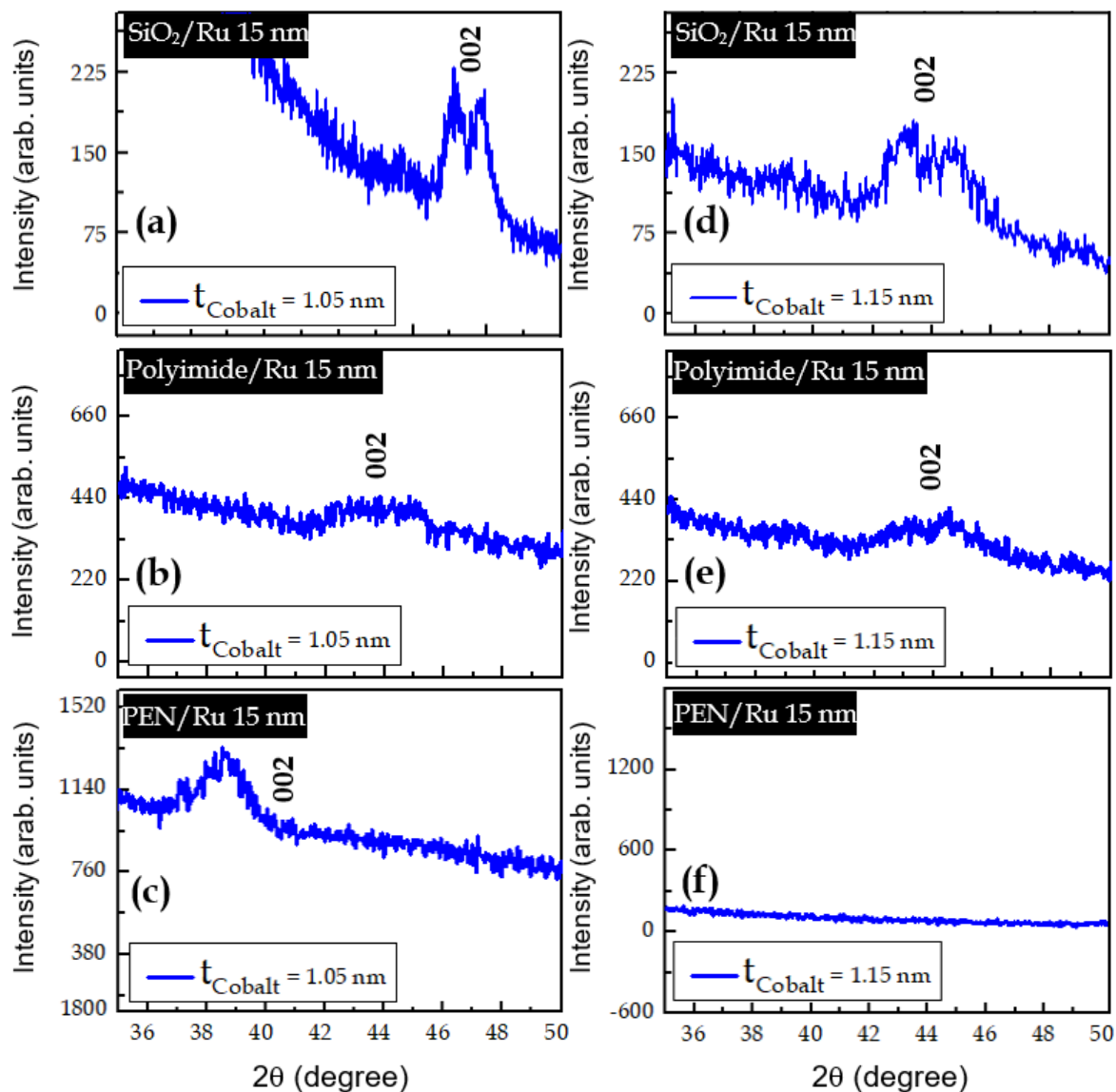
Fig. 7.19 (a,b,c). XRD patterns with 15 nm t_{Ru} with t_{Co} = 1.05 for SiO_2 , polyimide and PEN respectively. (d,e,f). XRD patterns with 15 nm t_{Ru} with t_{Co} = 1.15 for SiO_2 , polyimide and PEN respectively.
