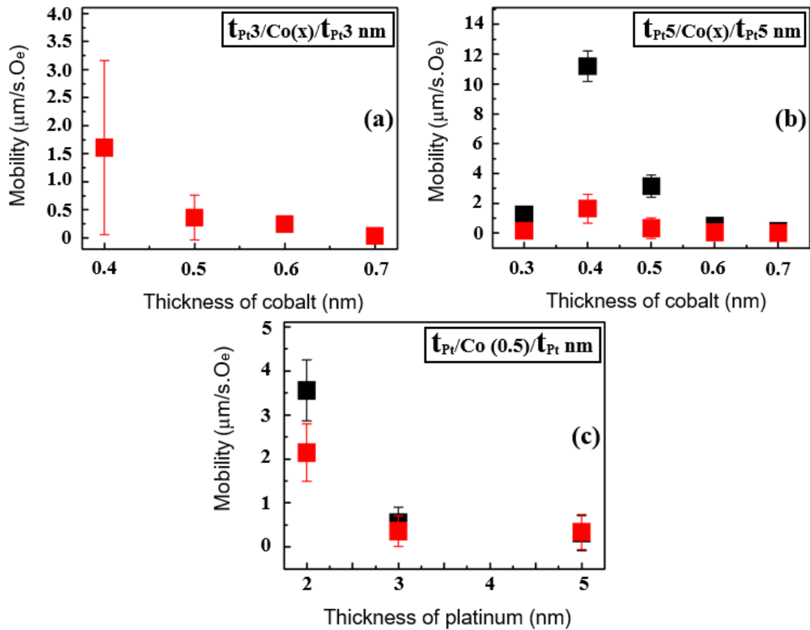
Fig. 8.9 a. Domain wall mobility of a t_{Pt} 3.0/t_{Co}/t_{Pt} 3.0 nm multilayers as a function of thickness of cobalt (nm). b. Domain wall mobility of a t_{Pt} 5.0/t_{Co}/t_{Pt} 5.0 nm multilayers as a function of thickness of cobalt (nm). c. Domain wall mobility of a t_{Pt}/t_{Co} (0.5)/t_{Pt} nm multilayers as a function of thickness of platinum (nm). The black and red symbols refer to the down-up and up-down reversal magnetization respectively.
