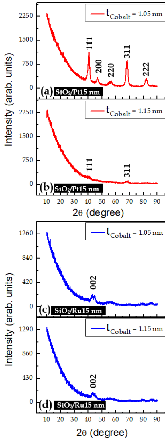
Fig. 7.6 X-ray diffraction scans of the (a,b) Pt15.0/(t_{Co})/Pt3.0\text{ nm} and (c,d) Ru15.0/(t_{Co})/Ru3.0\text{ nm} trilayer thin-films grown on SiO_2 substrate.
