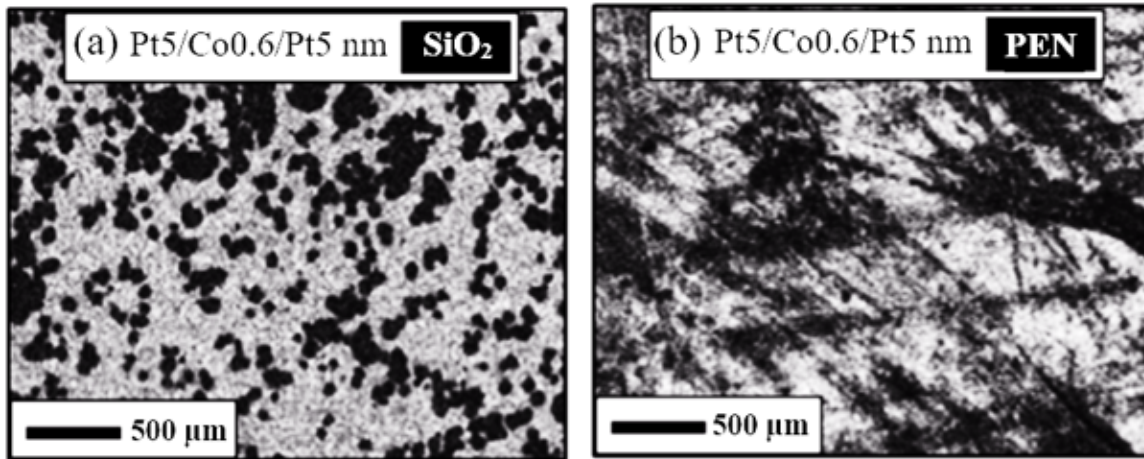
Fig. 4.12 Examples of MOKE microscopy imaging of magnetic films on (a) SiO 2 and (b) PEN using the MOKE microscope.
