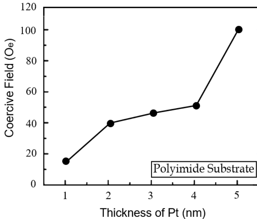
Fig. 6.15 Coercive field of t_{Pt}/Co\ 0.5/t_{Pt} nm as a function of platinum thickness grown on polyimide substrate. The error bar is very small.
