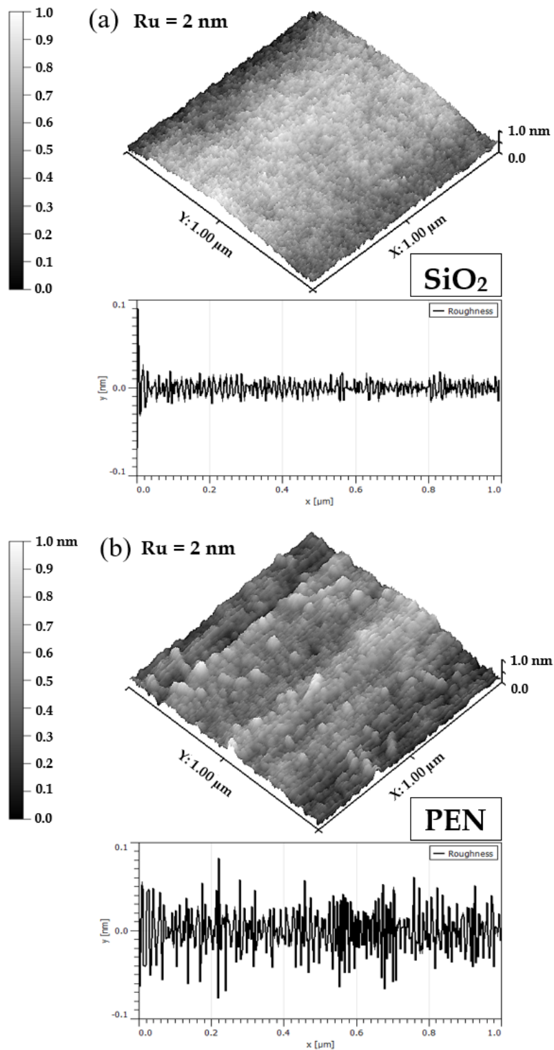
Fig. 5.11 Image illustrates the topography of 2.0 nm ruthenium grown on both (a). \text{SiO}_2 and (b). PEN substrates using atomic force microscopy machine.
