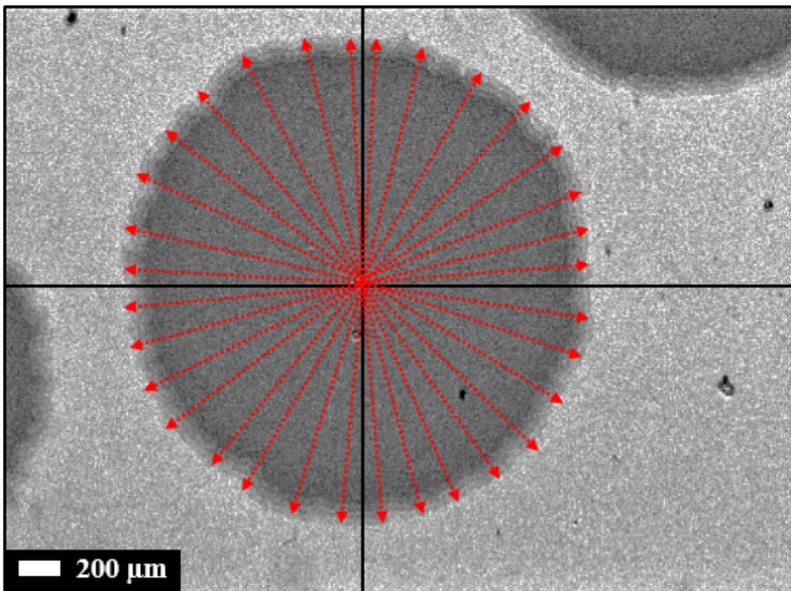
Fig. 2.6 Expansion of bubble for a t_{Pt} 2.0/t_{Co} (0.5)/t_{Pt} 2.0 nm at 80.7 Oe magnetic field.
