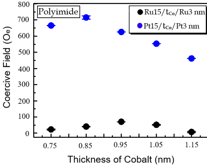
Fig. 7.12 Comparison between coercive field values with error bars for Ru15.0/( t_{Co} )/Ru3.0 nm and Pt15.0/( t_{Co} )/Pt3.0 nm using polyimide substrate.
