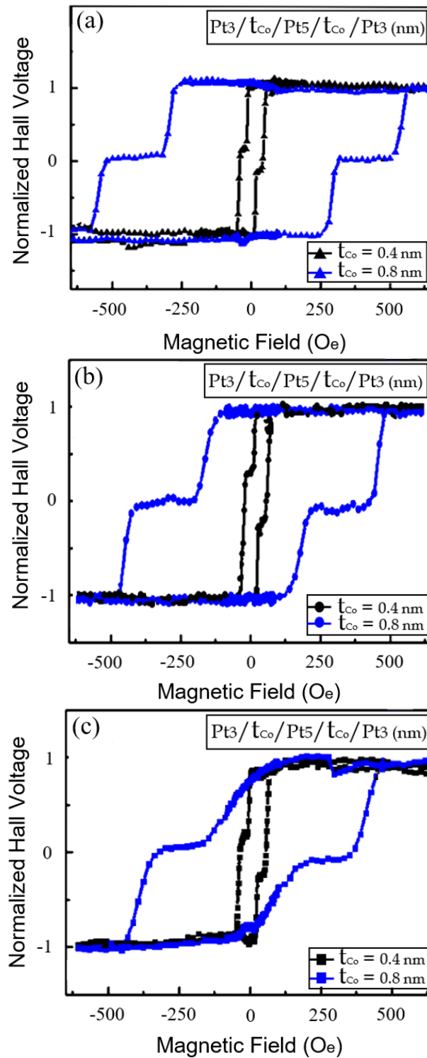
Fig. 6.21 (a,b and c) Graphs show two steps of hysteresis loops using different thickness of cobalt 0.4 nm and 0.8 nm respectively grown on (a). \text{SiO}_2 , (b). polyimide, and (c). PEN substrate.
