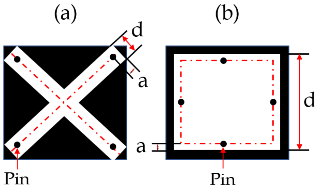
Fig. 4.17 Geometrical of the shadow mask with different shapes for Hall measurements for (a). Greek cross and (b). square shapes. Where, d is the length of deposition film and a is the distance between pin and the edge of deposition film. The white colour represents the deposition film region while the black colour represents the substrate region.
