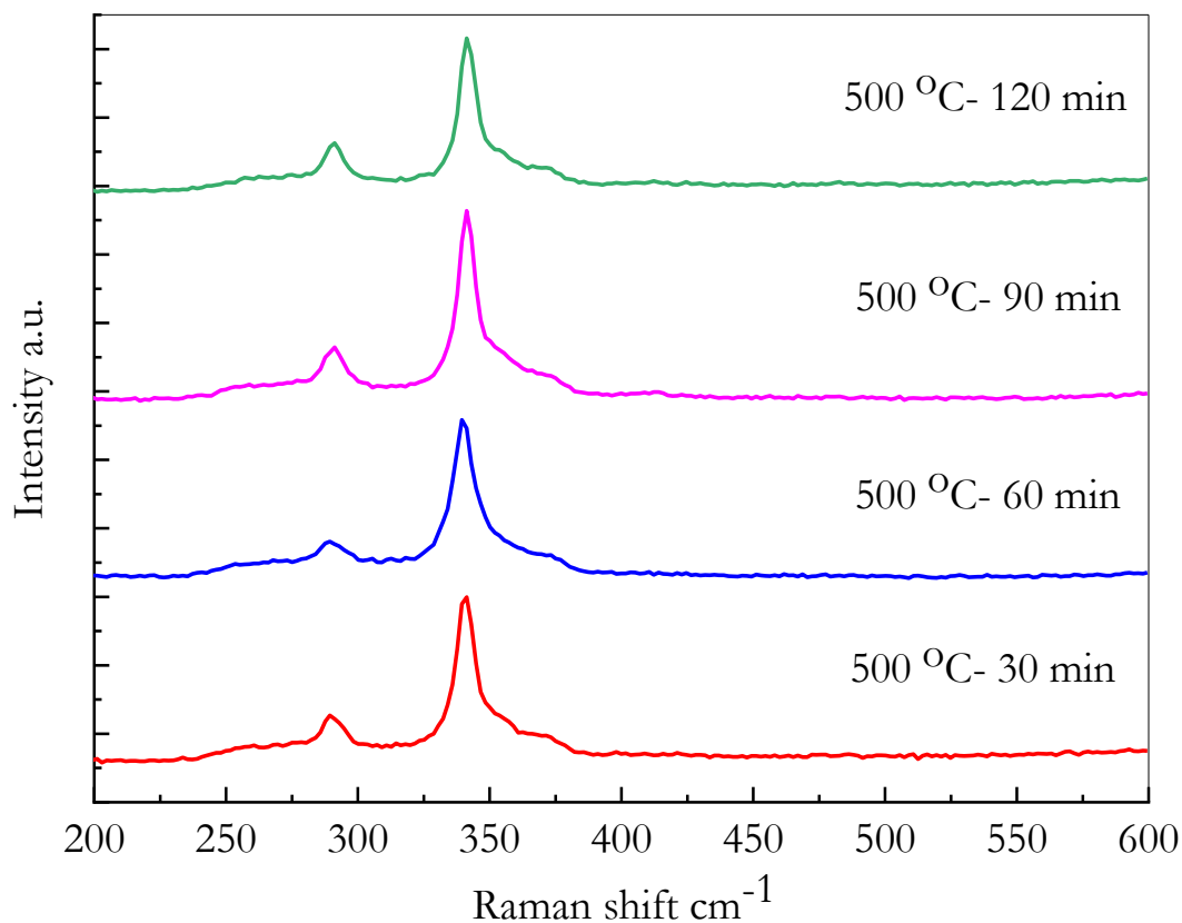
Figure 6.5 Raman measurements of CZTS films at different annealing times 30, 60, 90 and 120 min at 500\text{ °C}
