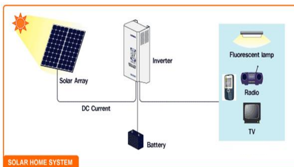
Figure 6:8 Components of a typical solar home system: Source: Author
