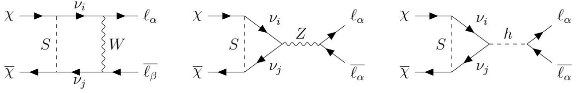
Figure 4.3: One-loop diagrams (in unitary gauge) contributing to annihilation of DM into charged lepton-antilepton pairs \ell_\alpha \bar{\ell}_\beta , \alpha, \beta = e, \mu, \tau . The indices i and j run from 1 to 4.
