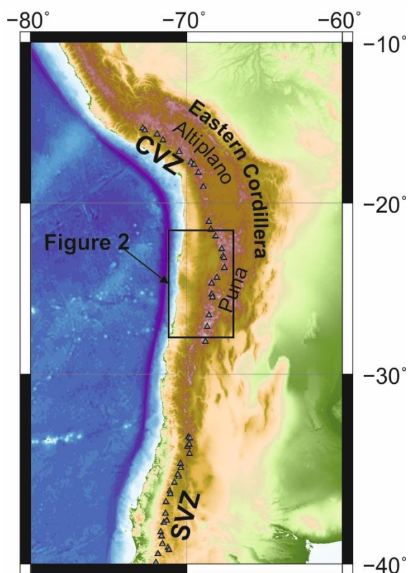
Figure 35: Overview map of the Andean Plateau. The active Central Volcanic Zone defines the Western Cordillera of the Andean Plateau. The Altiplano and Puna basins form the core of the Andean Plateau. The Eastern Cordillera fold and thrust belt make up the eastern boundary. The box shows the location of the study area for this Chapter, shown in further detail in Figure 2.
