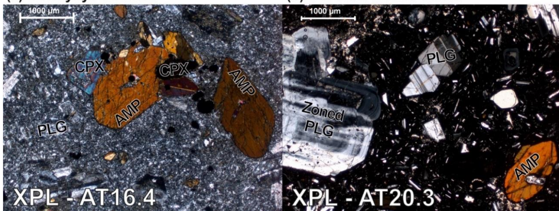
Figure 39: Two examples of samples containing amphibole phenocrysts, which are rare in most suites but common in both Cachiyuyo and Co. Chrisoteado suites. Both samples have strongly zoned plagioclase phenocrysts and euhedral to subhedral amphibole and plagioclase phenocryst phases.
