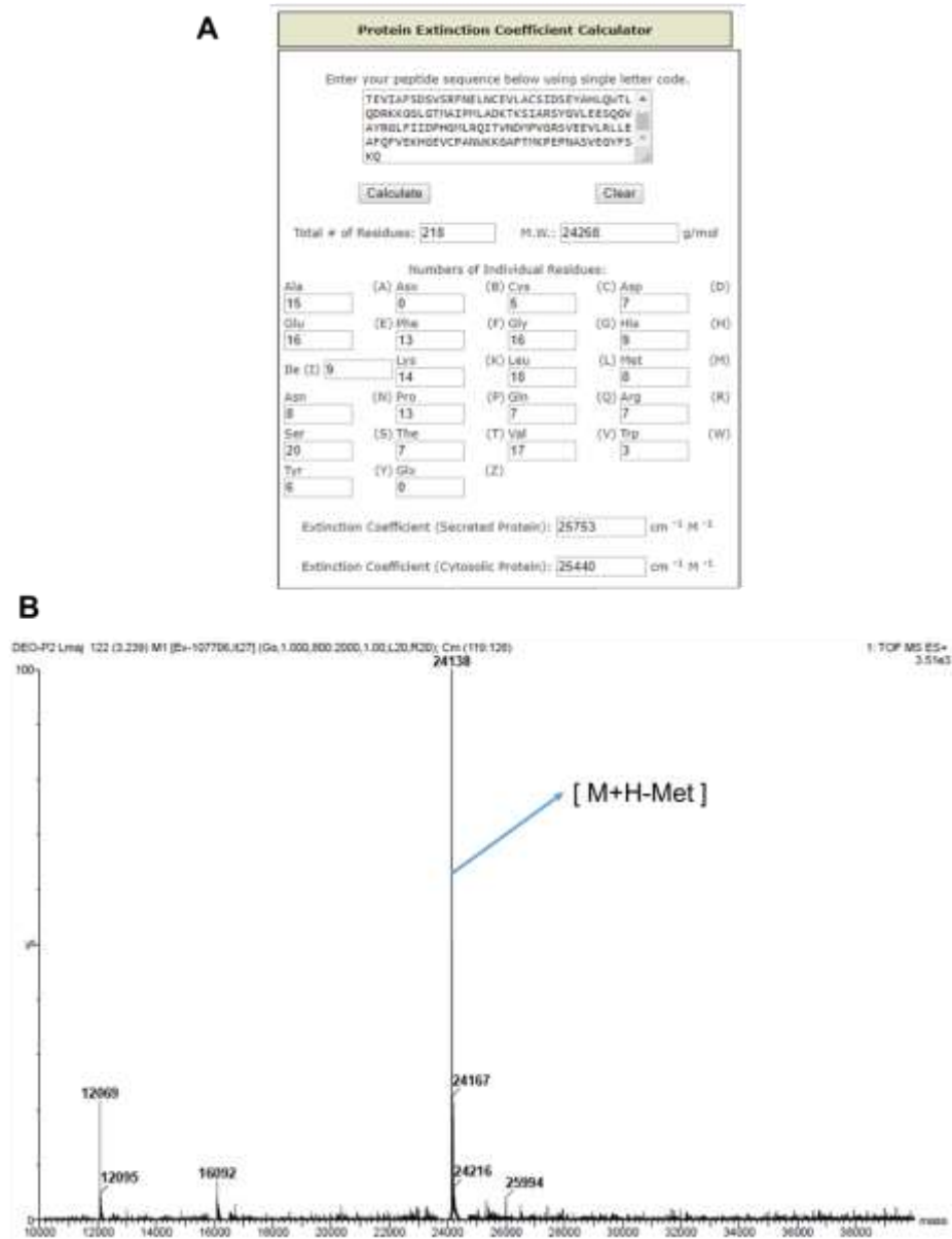
Figure 31. L. major cTXNPx mass spectrometry analysis. A- Protein mass and extinction coefficient of L. major cTXNPx calculated by biomol tool. B- L. major cTXNPx mass spectrum. M+H-Met requires 24138 Da.
