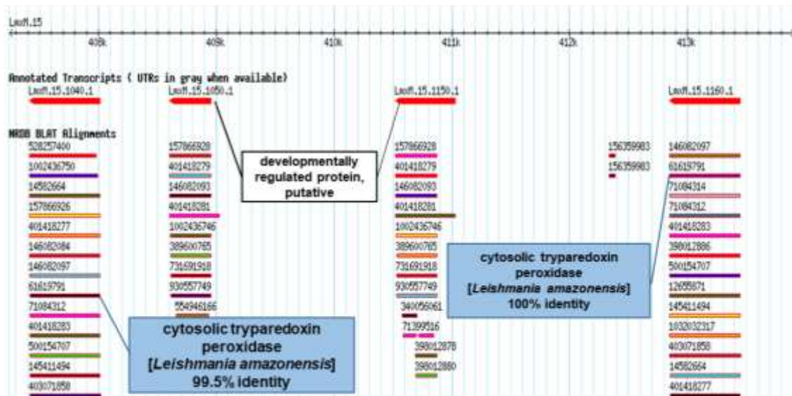
Figure 47. Localization of the genes encoding cTXNPx in the L. mexicana genome. A- Blue rectangles showing the encoding gene copies, LmxM.15.1040 and LmxM.15.1160, at chromosome 15. B- cTXNPx gene BLAT alignment between L. mexicana and L. amazonensis .
