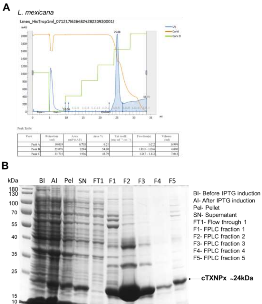
Figure 28. L. mexicana cTXNPx overexpression and purification by FPLC. cTXNPx protein overexpression was induced on BL21(DE3) cells by IPTG addition. All bacteria were disrupted by sonication and desired protein was purified from culture supernatant on Ni +2 -NTA columns by FPLC. A- FPLC chromatogram of L. mexicana cTXNPx purification. B- SDS-PAGE showing samples collected during all purification steps.
