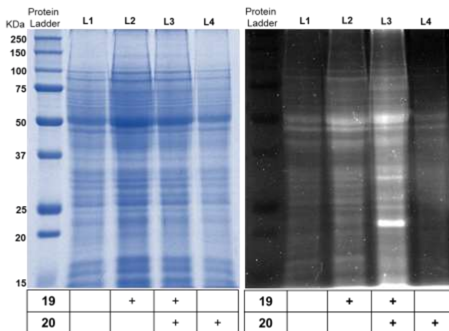
Figure 13. Chalcone probe binding on parasite proteins by SDS-PAGE. Proteins from L. amazonensis promastigotes pre-treated with 19 (0 and 5 \mu M) for 5 h were reacted with probe 20 (5 \mu M) for 1 h at RT. Proteins were analysed by 8% SDS-PAGE, left hand image shows proteins stained with comassie blue; Right hand image showed fluorescence signal detected by Gel Doc imager. L1- untreated parasites, L2- parasites treated with compound 19 , L3- parasites treated with chalcone 19 and linked to probe 20 , L4- untreated parasites linked to probe 20 .
