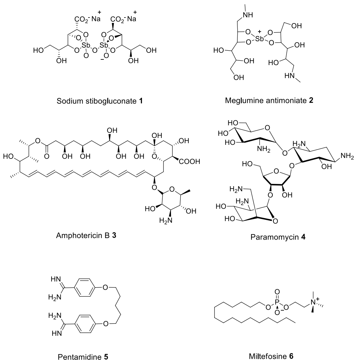
Figure 4. Chemical structures of the current treatments for leishmaniasis.
