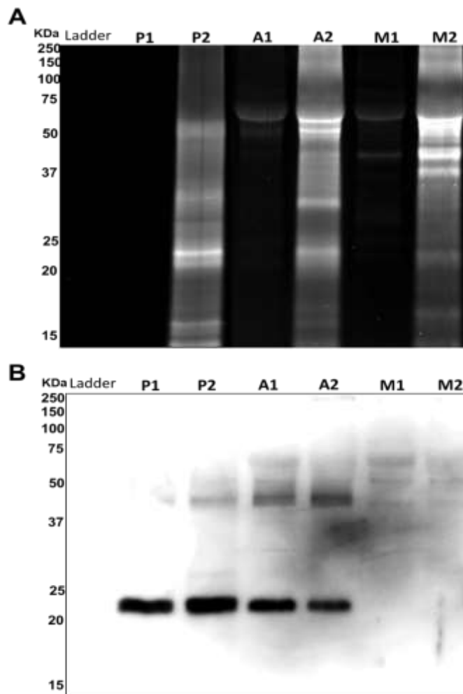
Figure 20. Chalcone target specificity for parasite. Proteins from L. amazonensis promastigotes, intracellular amastigotes and macrophages treated or not with 19 and linked to 20 were analysed by 10% SDS-PAGE. Proteins were visualised for their fluorescence and transferred to PVDF membrane. cTXNPx were detected on the membrane by western Blot using a polyclonal antibody anti-cTXNPx. A- Gel fluorescence image. B- cTXNPx detected by immunoblotting. P- Promastigotes proteins. A- Amastigotes proteins. M- Uninfected macrophages proteins. P1, A1 and M1- Samples non treated with 19 . P2, A2 and M2- Samples treated with 19 .
