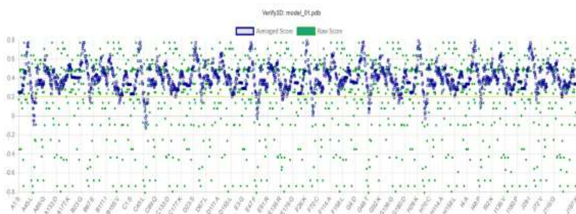
Figure 45. Validation of 3D model of L. amazonensis cTXNPx. The three-dimensional structure of the model proposed for cTXNPx were validated by the scores between 1D and 3D structures by Verify3D tool on SAVES.
