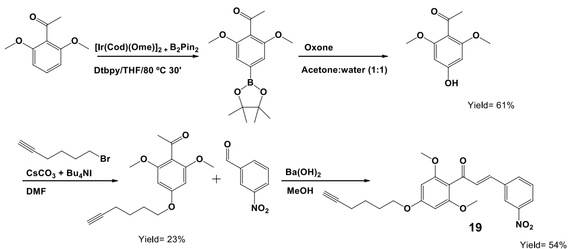
Scheme 3. Synthesis route of chalcone analogue ( 19 ) with an alkyne group.
