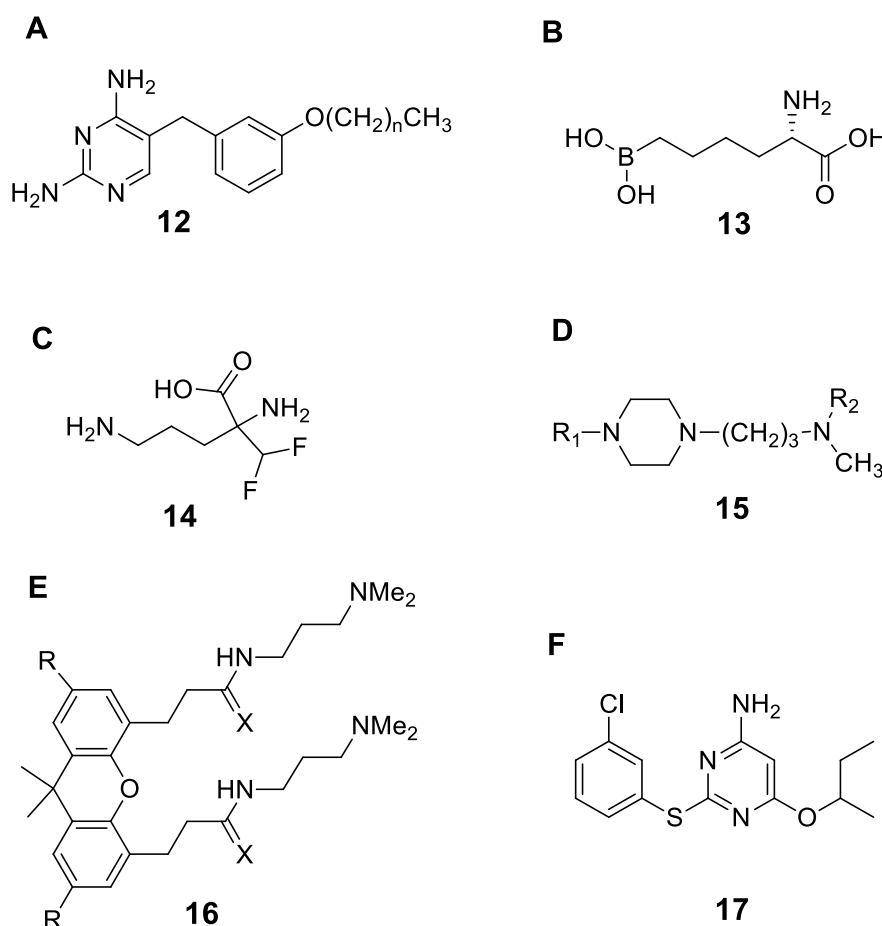
Figure 7. Inhibitors for essential parasite drug targets. A- 2,4-diaminopyridimine, 12 72 . B- 2(S)-amino-6-boronohexanoic acid, 13 86 . C- Eflornithine, 14 87 . D- Piperazine derivatives, 15 88 . E- 9,9-dimethylxanthene derivatives, 16 89 . F- Diaryl sulfide derivative, 17 90 .
