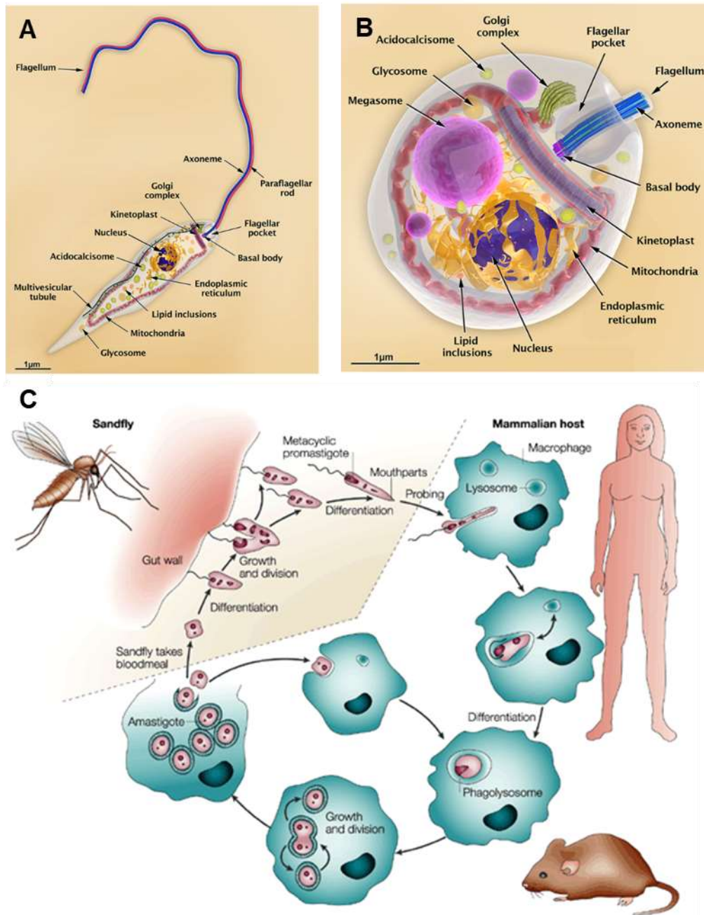
Figure 3. Leishmania spp. developmental stages and life cycle. A- Leishmania promastigote form. B- Amastigote form. C- Parasite life cycle including vertebrate and invertebrate hosts. Images were adapted from Teixeira et al 16 . and Sacks et al 17 .
