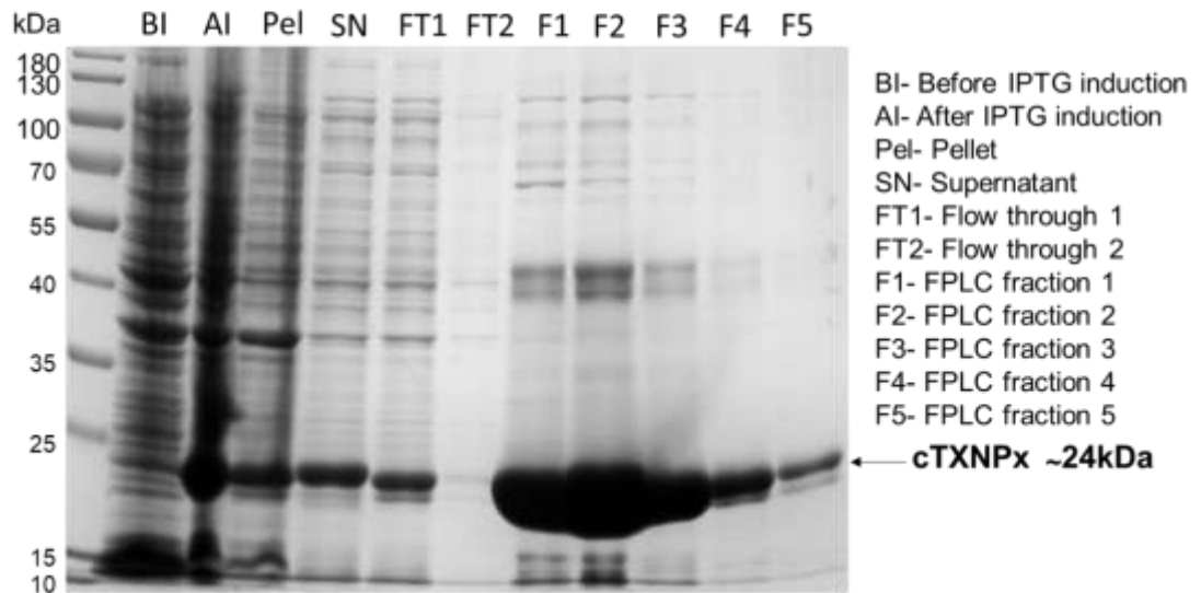
Figure 27. L. major cTXNPx overexpression and purification by FPLC. cTXNPx protein overexpression was induced on BL21(DE3) cells by IPTG addition. All bacteria were disrupted by sonication and desired protein was purified from culture supernatant on Ni 2+ -NTA columns by FPLC. A- FPLC chromatogram of L. major cTXNPx purification. B- SDS-PAGE showing samples collected during all purification steps.
