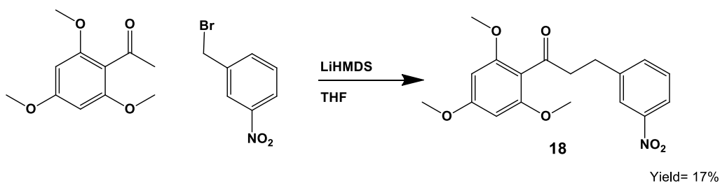
Scheme 2. Chalcone lacking enone group ( 18 ) synthesis.
