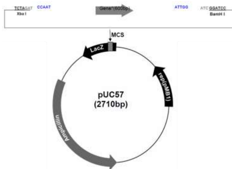
Figure 21. General plasmid construct map. The plasmid constructs were purchased from Genscript; the gene of interest were cloned at MCS position flanked by protective bases added by the company (Blue bases).
