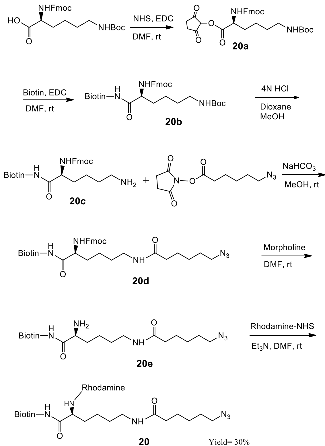
Scheme 4. Trifunctional probe ( 20 ) synthesis route.
