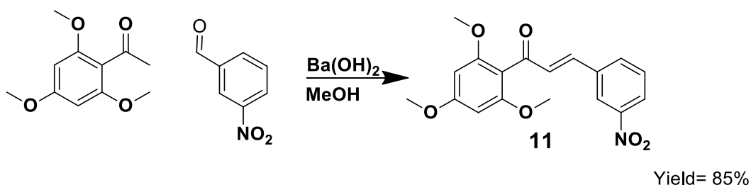
Scheme 1. Chalcone NAT22 ( 11 ) synthesis.
