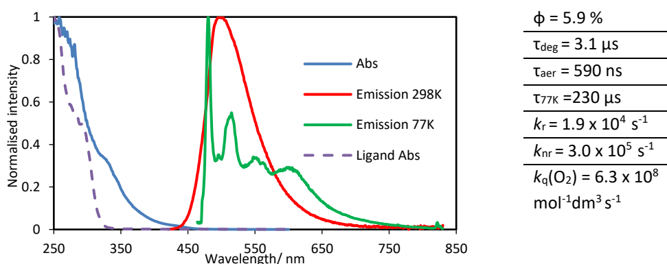
Figure 3.10: RT absorption and degassed emission spectra of [Pt(dpyb)L 1 Cl] + in DCM and 77 K spectrum in EPA.
