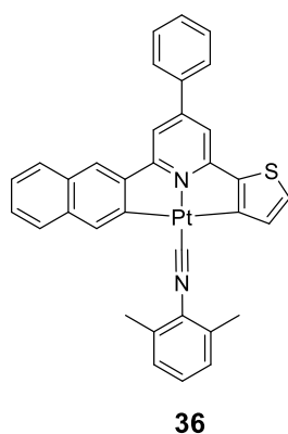
Figure 3.4: Structure of complex 36 and its PL and EL emission spectra. Reproduced from Kui et al. by permission of John Wiley and Sons. 126
