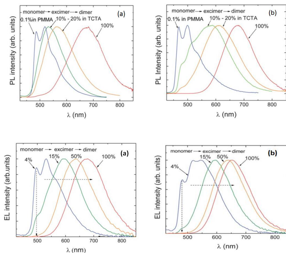
Figure 2.14: Top: Solid-state PL spectra of (a) 31 and (b) 32 and bottom: EL spectra of (a) 31 and (b) 32 with different dopant concentrations in the TCTA host. Reproduced from Brulatti et al. by permission of the Royal Society of Chemistry. 111
