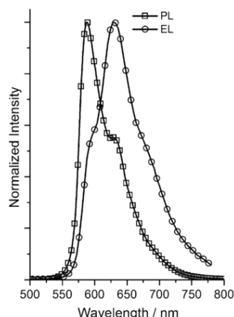
Figure 3.4: Structure of complex 36 and its PL and EL emission spectra. Reproduced from Kui et al. by permission of John Wiley and Sons. 126
