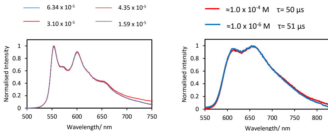
Figure 4.21: Concentration-dependent spectra for Pt and Pd complexes ML 19-22 . *Emission shown for PdL 19 and PdL 20 may represent a new species forming in solution.
