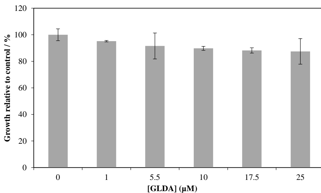
Figure 3-12. Inhibition profile of GLDA on E. coli grown at 37°C at 125 rpm until mid-log phase of growth. GLDA concentrations used were 0, 1, 5.5, 10, 17.5 and 25 \mu\text{M} . The data presented shows the growth of the sample when compared to an untreated control and is therefore a relative representation.
