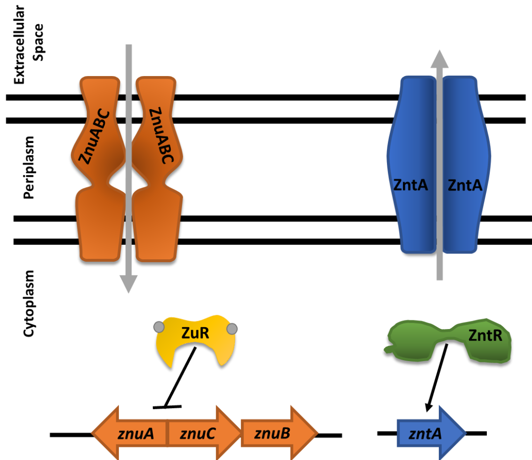
Figure 1-4. Zinc homeostasis in E. coli . Zinc(II) atoms are represented by grey circles. Grey arrows indicate the the direction of zinc ion transport. The black arrow represents transcriptional activation whereas the truncated (⊥) line indicates transcriptional repression. Adapted from Takahashi et al. (2015).
