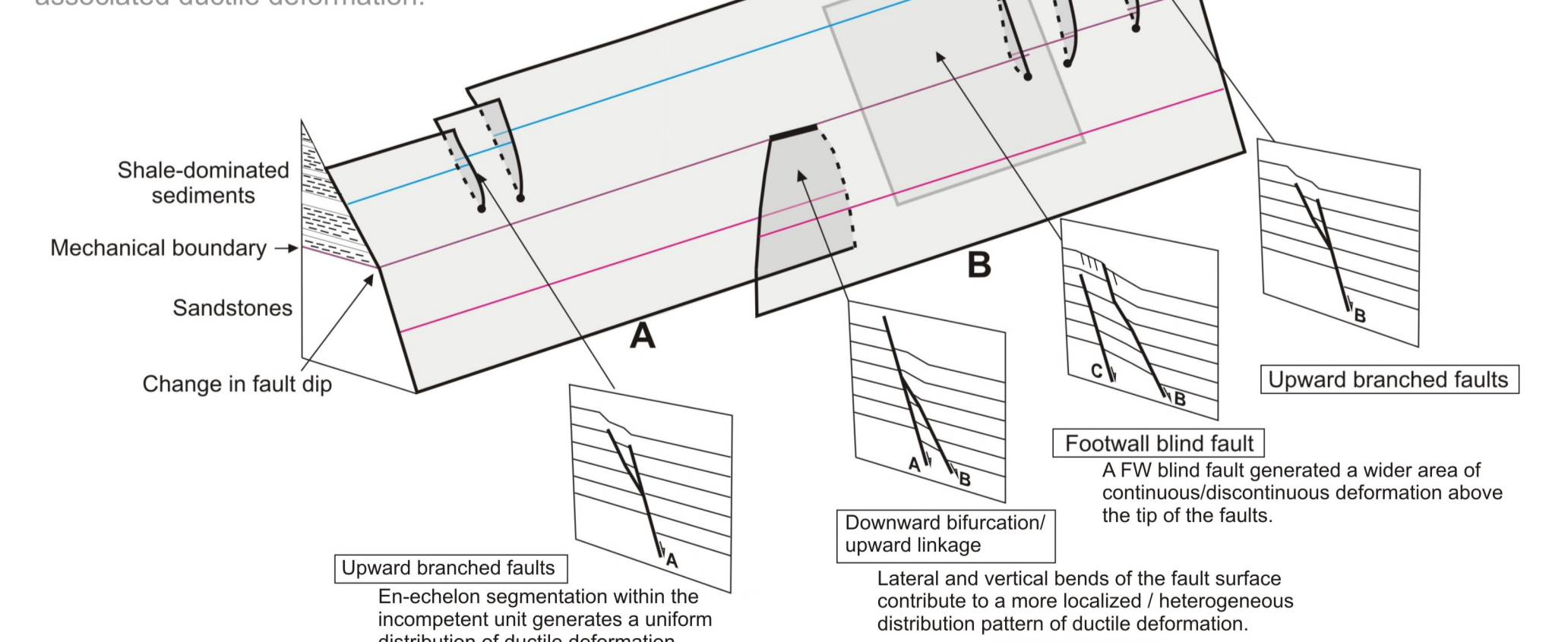
Figure 13. Fault segmentation and associated ductile deformation.
