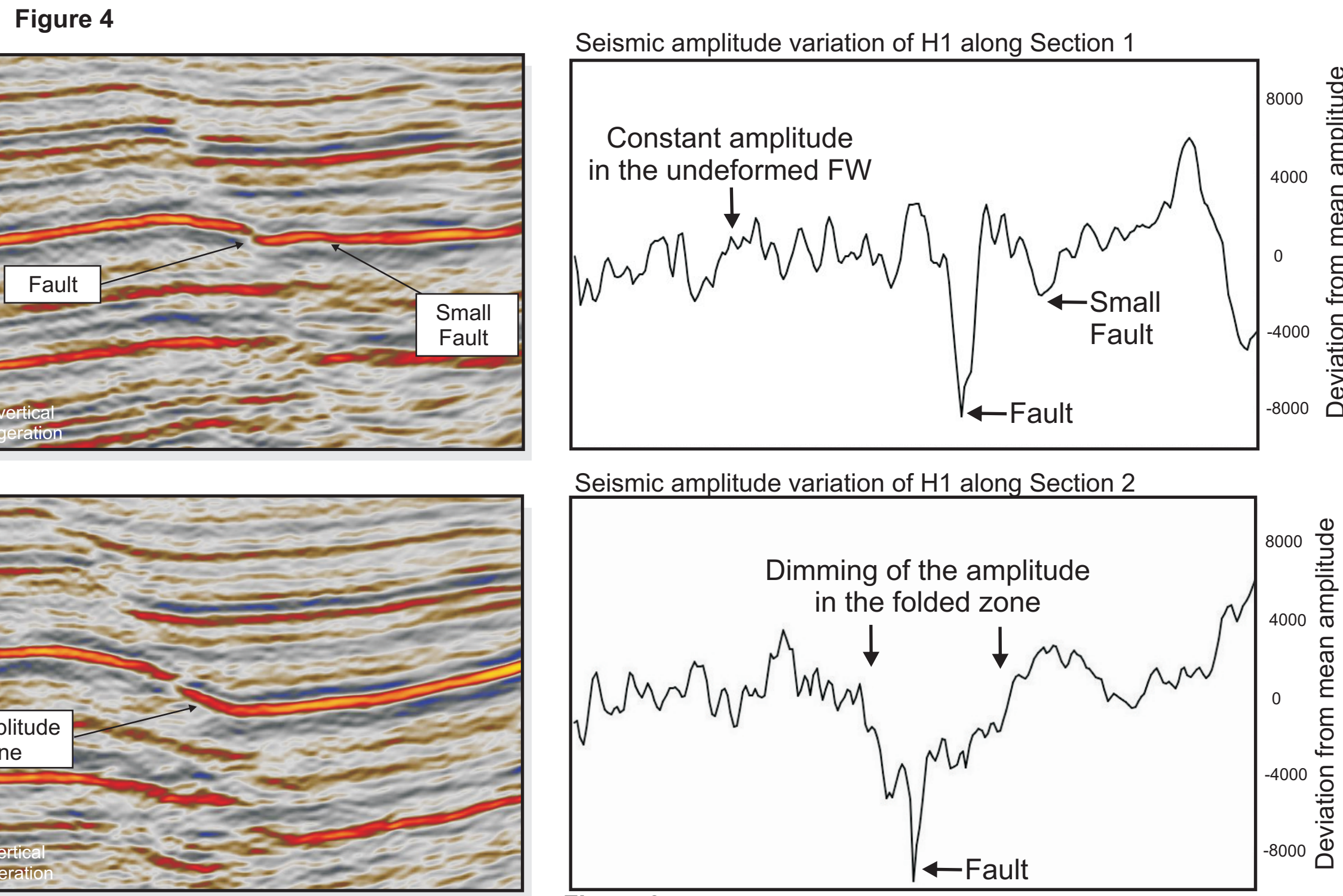
Figure 9 Seismic amplitude variation of H1 along Section 1 and Section 2.
