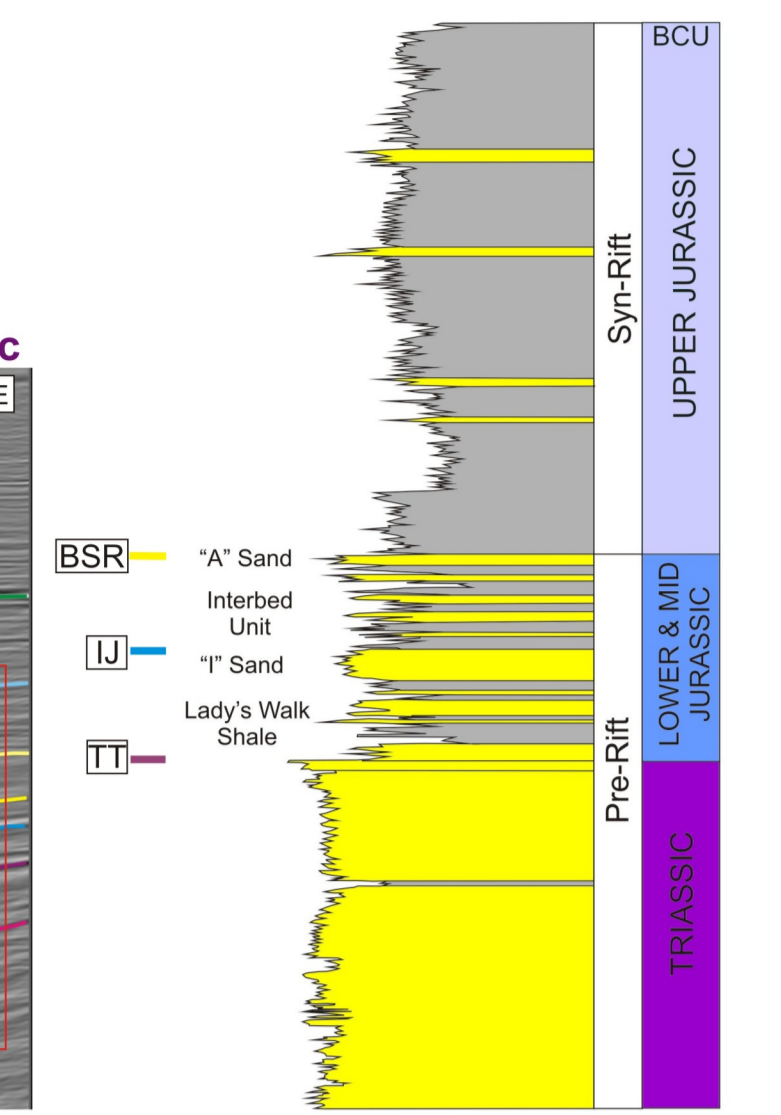
Figure 2. Jurassic-Triassic litho-stratigraphic column from the Beatrice Field.
