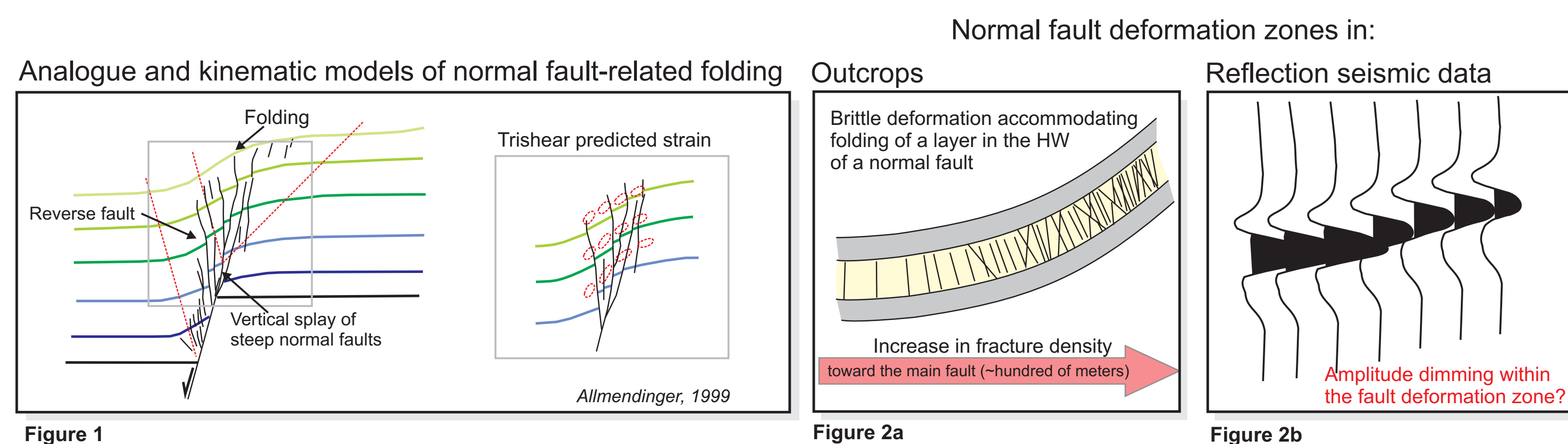
Figure 1 Analogue and kinematic models of normal fault-related folding. Figure 2a Outcrops. Figure 2b Reflection seismic data.
