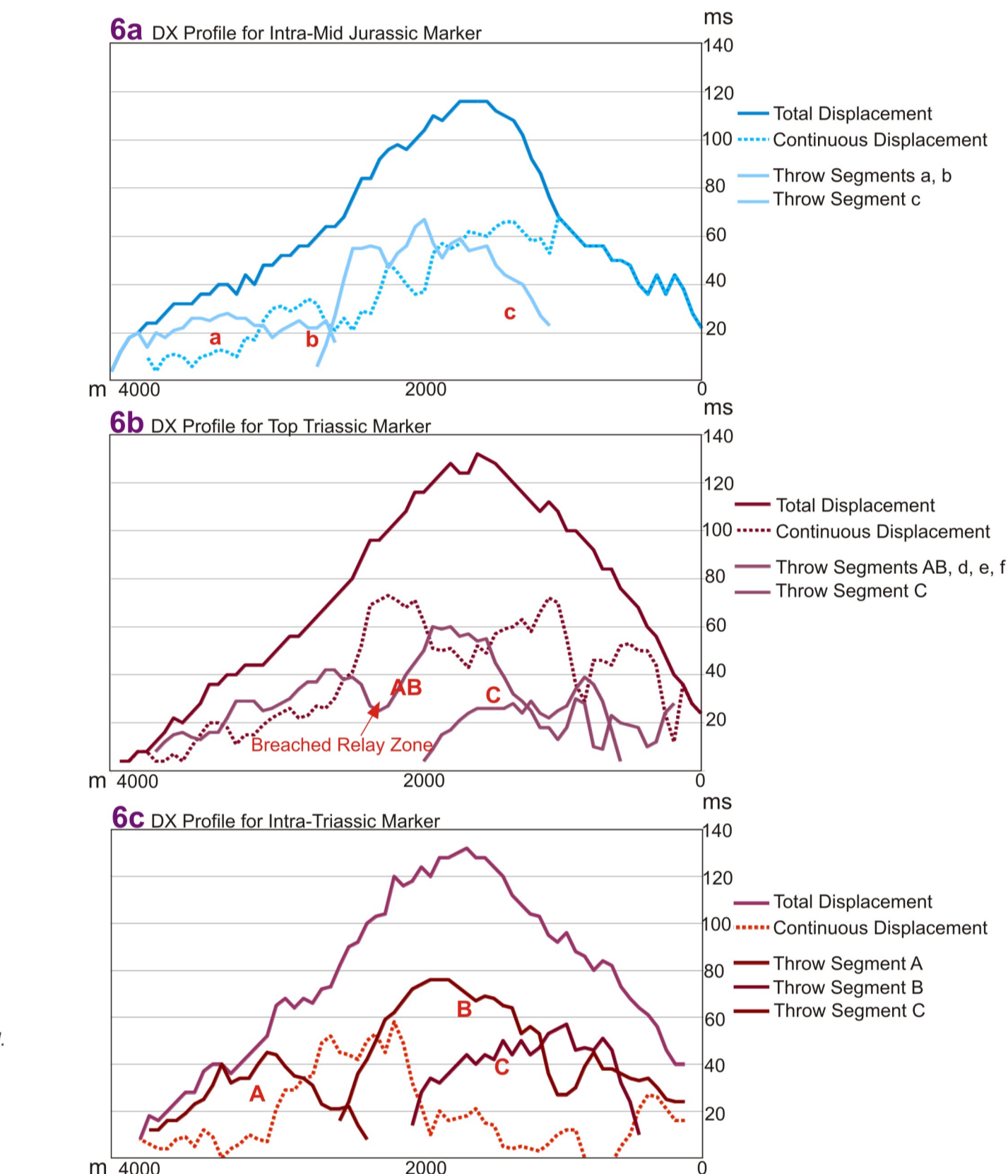
Figure 6a, b, c. Displacement-distance (DX) profiles for 3 of the mapped horizons.
