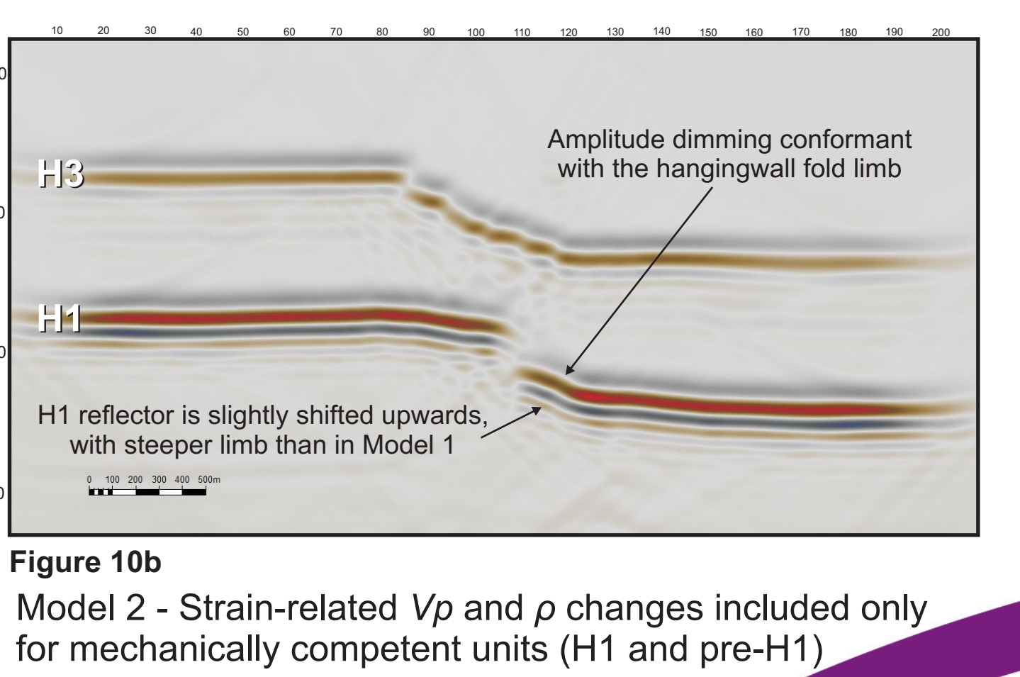
Figure 10b Model 2 - Strain-related V_p and \rho changes included only for mechanically competent units (H1 and pre-H1).
