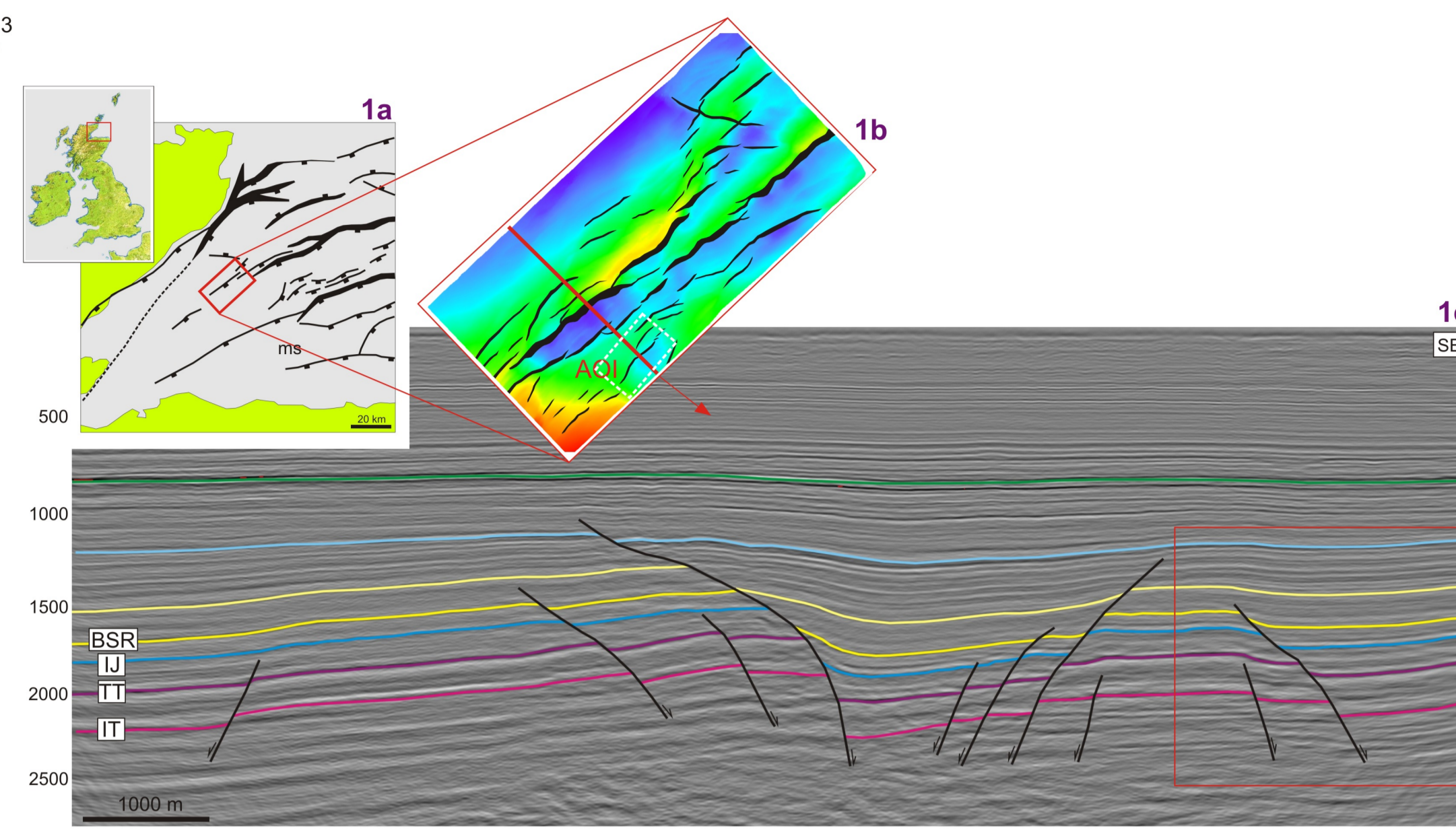
Figure 1 a, b, c. 1a - Schematic regional structural map of the Inner Moray Firth Basin (from Long and Imber, 2010) with the location of the interpreted 3D seismic volume. 1b - Top Triassic TWT structural map with the location of the studied fault-array. 1c - Seismic section orthogonal to the strike of the Jurassic normal faults; the analysed faults are bordered by the red square.
