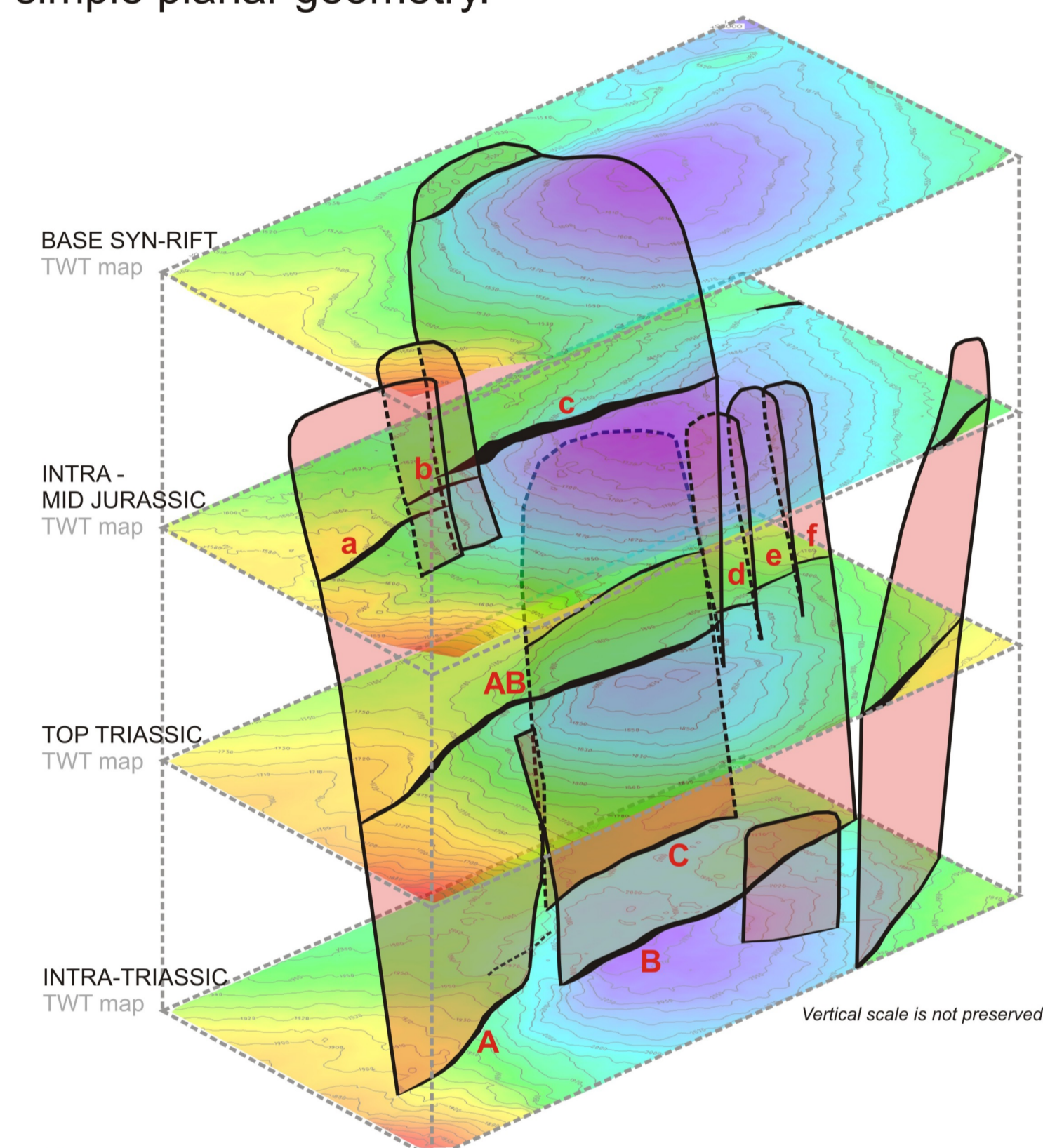
Figure 5. Structural maps of the main markers and the 3D geometry of the faults.
