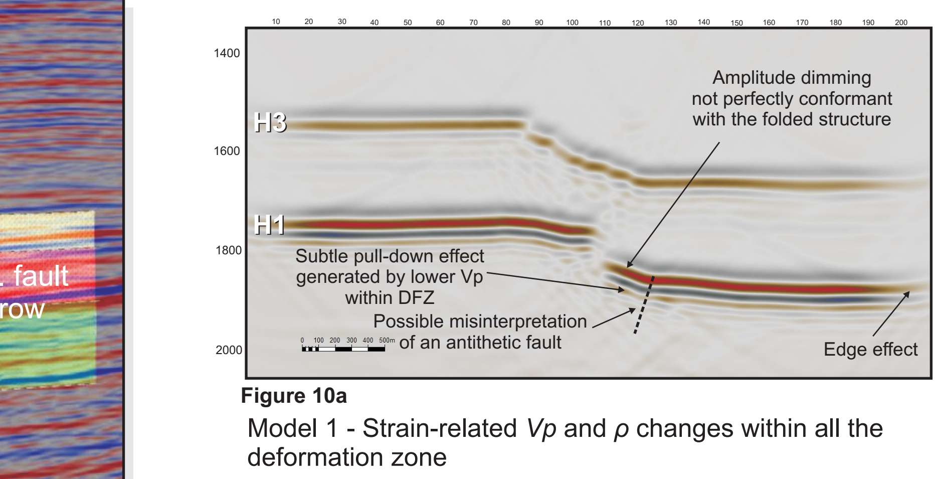
Figure 10a Model 1 - Strain-related V_p and \rho changes within all the deformation zone.
