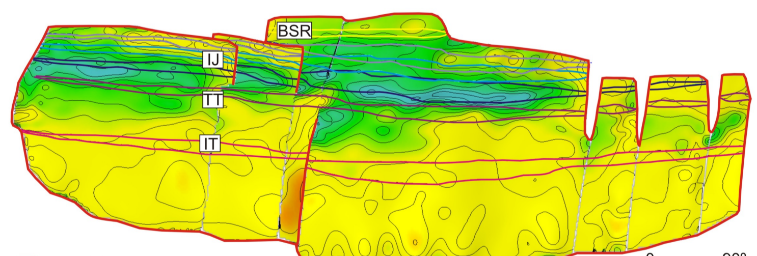
Figure 7. Fault dip
