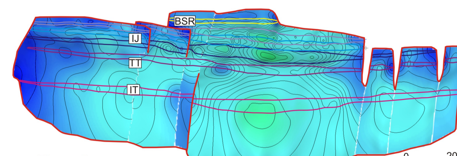
Figure 8. Fault throw (ms)
