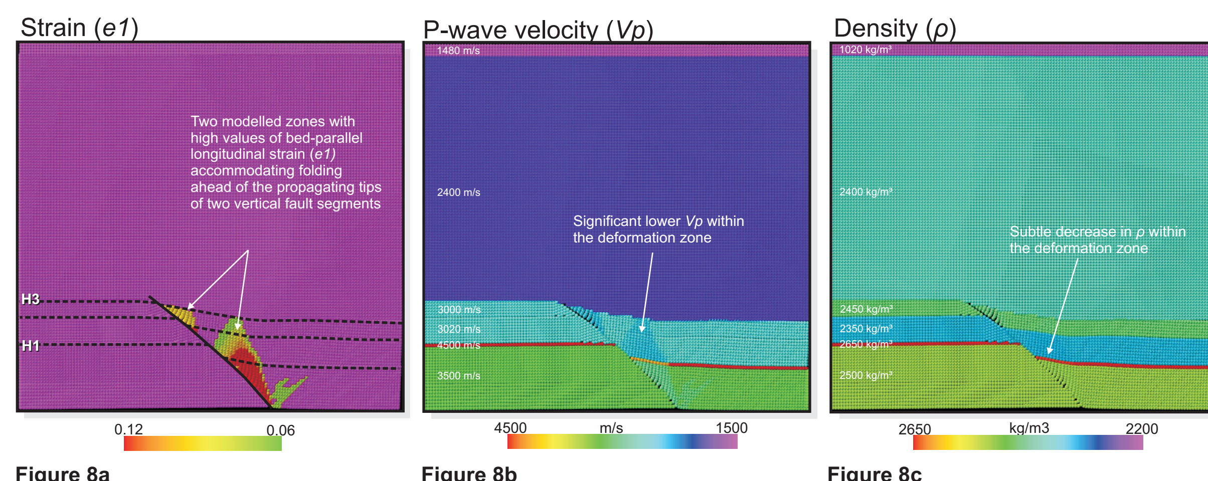
Figure 8a Strain (epsilon_1). Figure 8b P-wave velocity (Vp). Figure 8c Density (rho).
