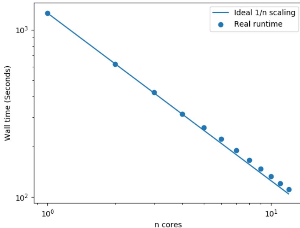
Figure 3.9: Wall time of the code as a function of the number of cores used. The dots show the measured results and the line shows the ideal 1/n scaling extrapolated from the run with a single core. It can be seen the code scales closely to the ideal case.
