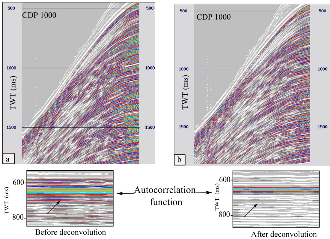
Figure 3.16. CDP gather from Line-19. (a) Before applying deconvolution. (b) After applying deconvolution. Note that this filter has improved the resolution of the seismic data by compressing the seismic wavelet and attenuating the low frequencies.
