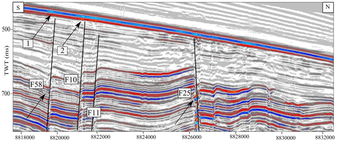
Figure 3.17. Result of the deconvolution with filter length of 8ms and gap length of 100ms along Line 3328. Note how the filter has improved or promoted the appearance of the amplitude anomalies at the seabed as shown by arrows 1 and 2 compared to the final stack with radon filter in Figure 3.14a.
