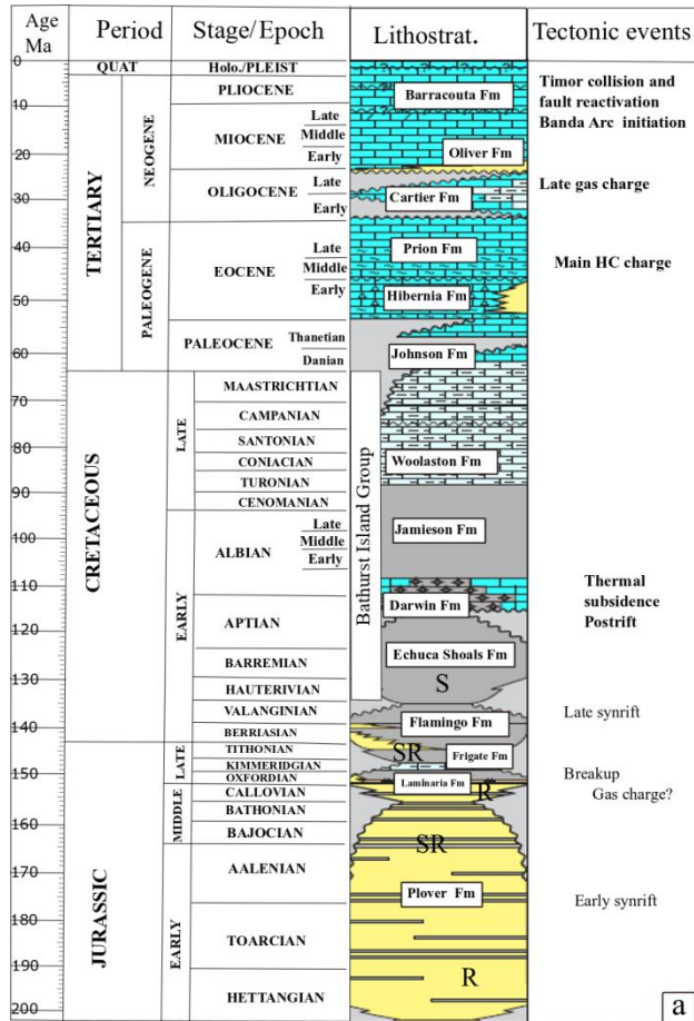
Figure 1.3. a. Generalized stratigraphic column for the Laminaria High (modified from De Ruig et al. 2000); b. Seismic section showing the interpreted horizons and their age used for the seismic and structural interpretation in Chapter 2.
