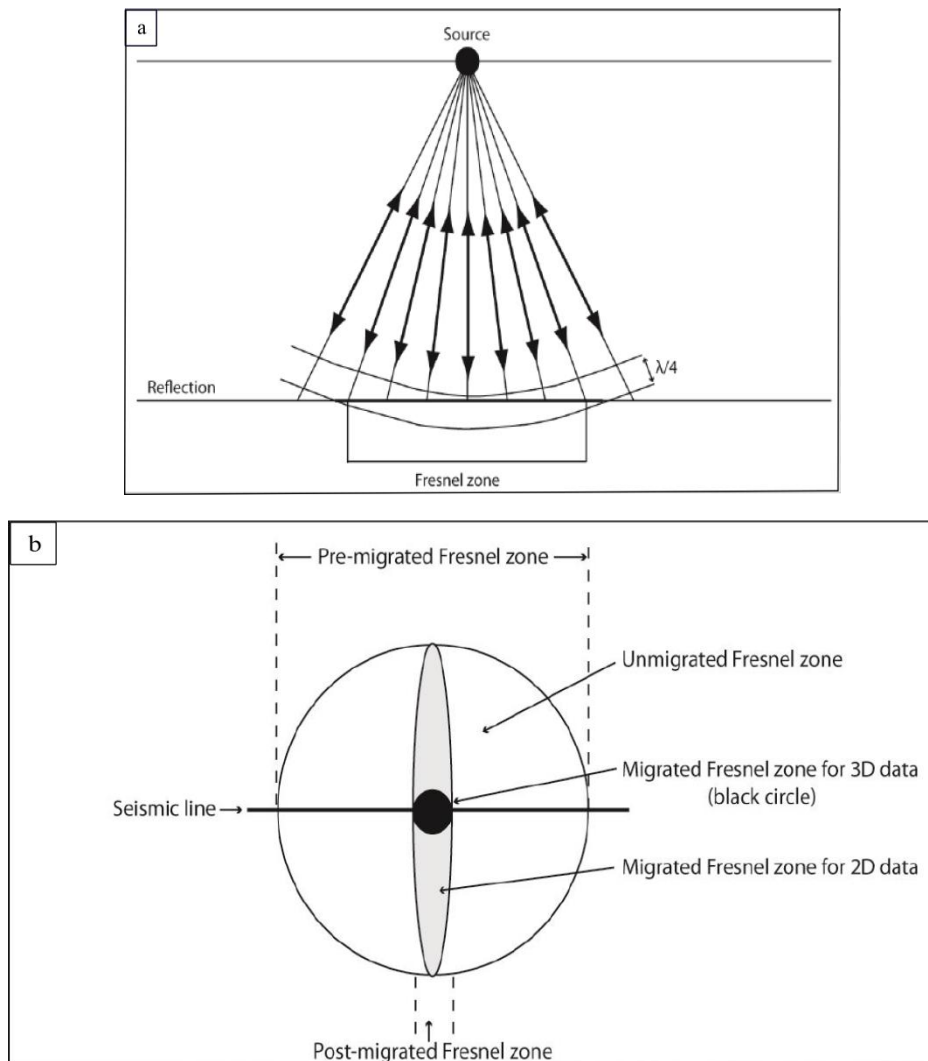
Figure 1.10. (a) Seismic wavelets that are returned to a detector within half a wavelength of the initial reflected arrival forms the Fresnel zone (from Kearey et al., 2002). (b) The Fresnel zone before and after migration (from Brown, 2011).
