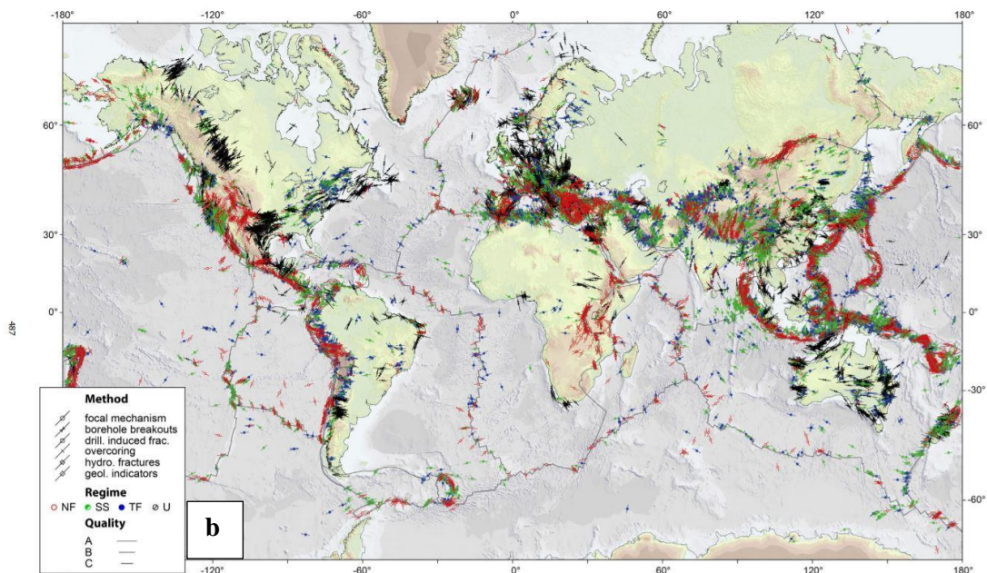
Figure 5.4. a. Earthquakes record along the Australian-Indonesian collision zone from 1979 to 1997. Crosses are earthquakes with M > 4.5 and diamonds are earthquakes with M > 6.5 (from Castillo et al., 1998). Note that the Laminaria High is located within this active area. b. world stress map based on the WSM database released in 2008. Lines show the maximum horizontal stress S_H ; red is for normal faults, green for strike-slip faults, black for unknown fault regime (from Heidbach et al, 2010).
