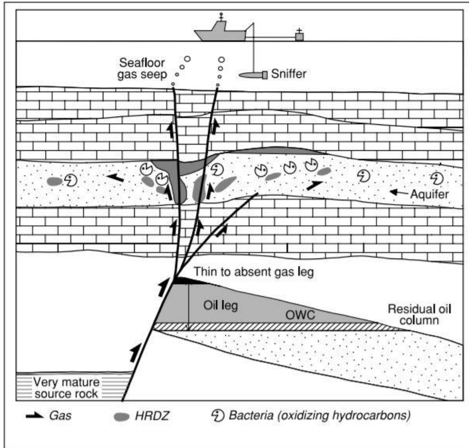
Figure 1.5. Schematic, showing the formation process of the authigenic carbonate in the Vulcan sub-basin. Hydrocarbons migrating up the faults and are oxidized by bacteria releasing CO 2 that is combined with carbonate cementation along the fault zone (from O’Brein et al., 2002). HRDZ= hydrocarbon related diagenetic zones.
