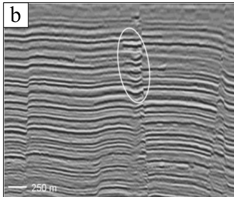
Figure 1.4. 2D seismic sections showing examples of bright spots. (a) Bright spot above a fold at the edge of the Makran continental margin of Pakistan and Iran in the Gulf of Oman (from White, 1977). (b) Bright spots due to hydrocarbon leakage along fault at the Mediterranean Sea (from Ligtenberg, 2005).
