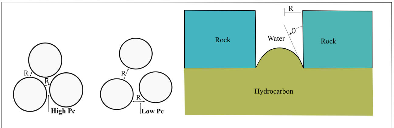
Figure 4.4. Parameters controlling the capillary displacement pressure (modified from Downey, 1984), Note the capillary entry pressure increase when the throat radius of the largest connected pores decreases and vice versa.
