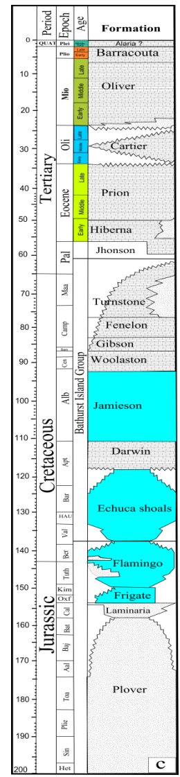
Figure 2.1. (a) Topographic and bathymetric map of the main basins on the Northwest Shelf of Australia. Elevation and depth data provided by Geoscience Australia (2018). (b) Geological setting and Jurassic structure map of northwestern Bonaparte Basin, modified from Long and Imber (2012). (c) Generalized stratigraphic column for the Laminaria High (modified from De Ruig et al. 2000).
