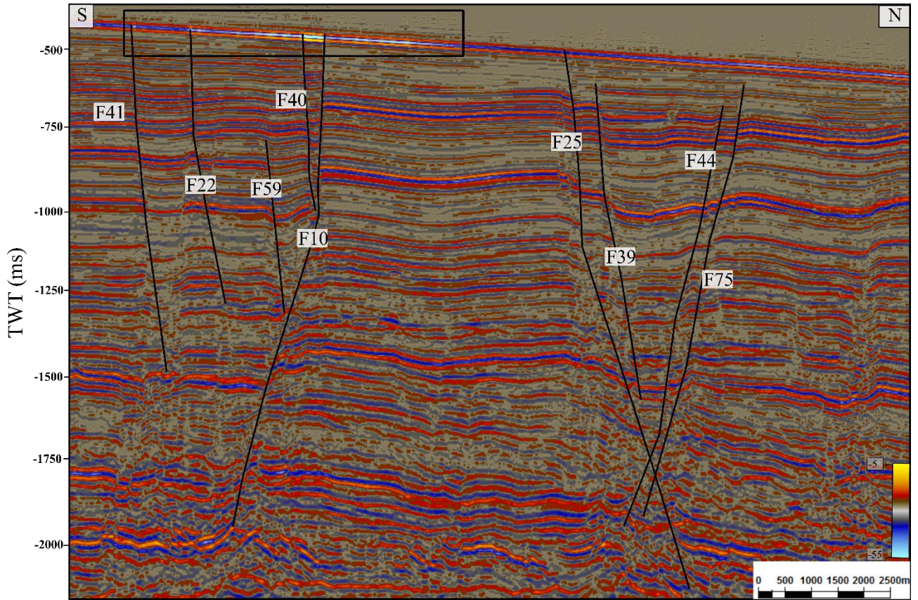
Figure 2.3. Seismic profile (cross line no. 2325) showing the geometry of the main faults in the study area. Note the amplitude anomaly at the seabed associated with fault F10 (box). Location of the seismic profile is shown in Figures 2.2a and 2.4.
