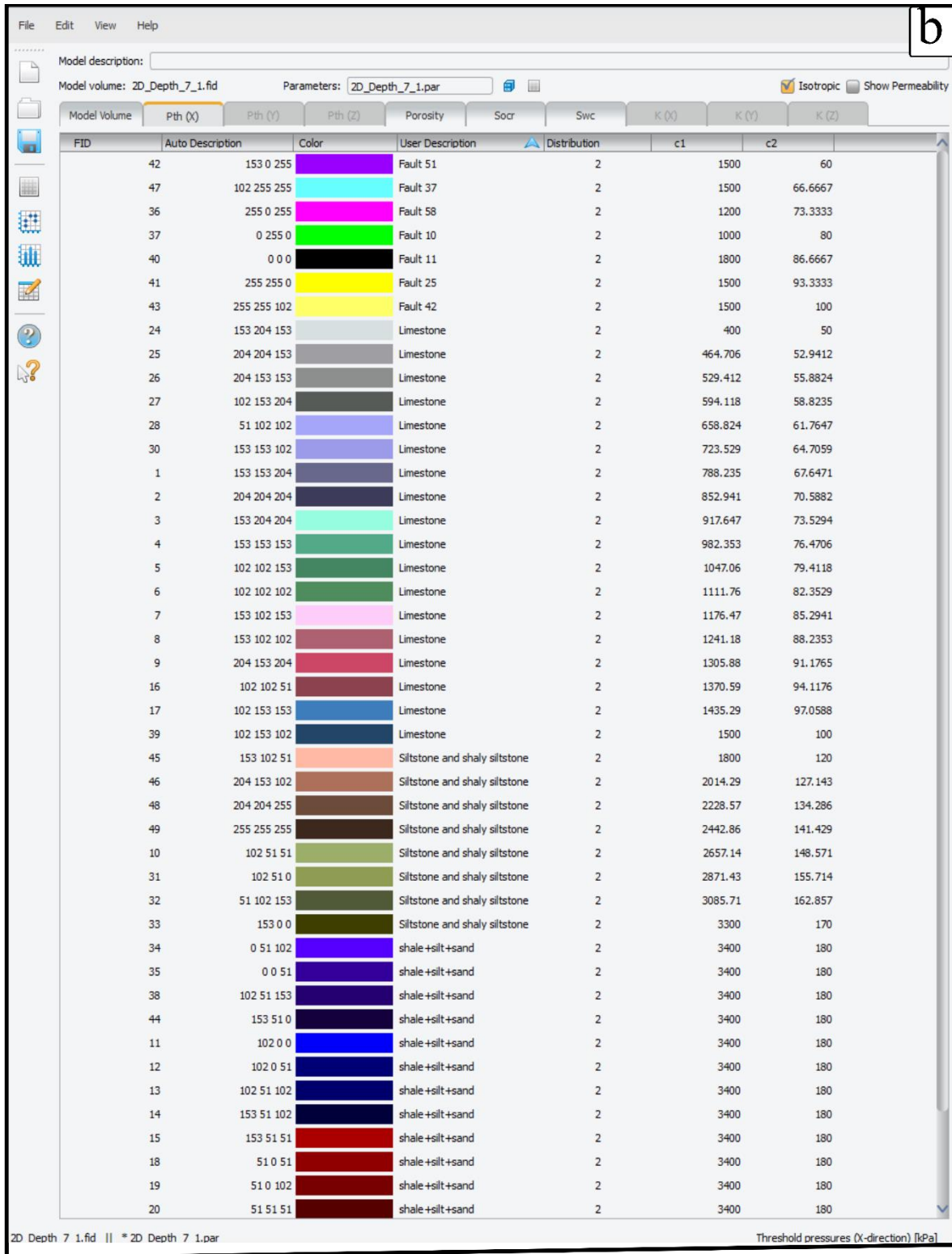
Figure 4.7. a. 2D seismic section (A-A') with a zoom into this section showing a mesh that has a large number of grid cells. Each cell appears as a separate colour representing a flow identification domain (FID); each colour was assigned as a single petrophysical property (CEP) in the volume editor. b. Extract of the volume editor parameter from Permedia showing the input CEP values and distribution assigned to lithologies and colour scales representing assigned lithofacies in normal distribution (see section 4.6.2.2.4 in text) for the first scenario along section A-A' .
