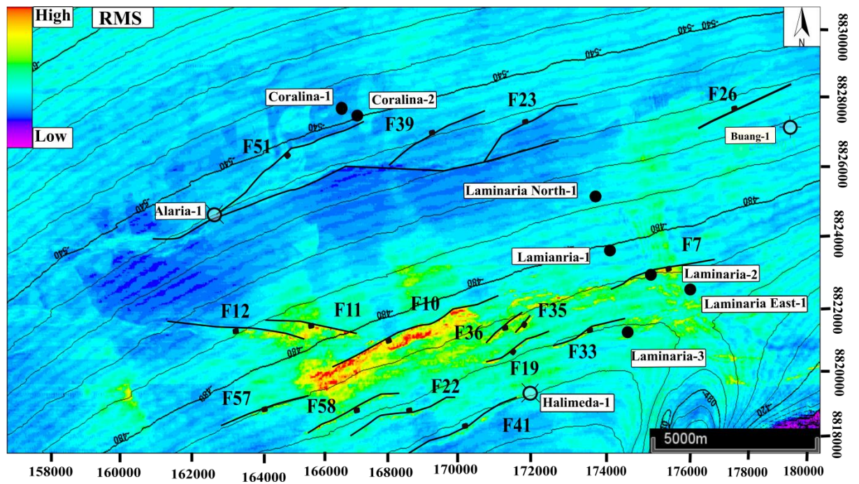
Figure 2.5. RMS amplitude map for the seabed showing a similar distribution of anomalies as shown in Figure 2.4. The two-way time structure contours for this horizon are shown. The principal RMS amplitude anomalies are associated with sets of normal faults F7, F10, F11, F12, F19, F35 and F36 in the southern part of the study area.
