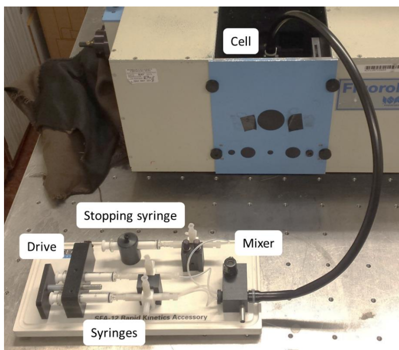
Figure 2.8 SFA-12 Rapid Kinetics Accessory.
