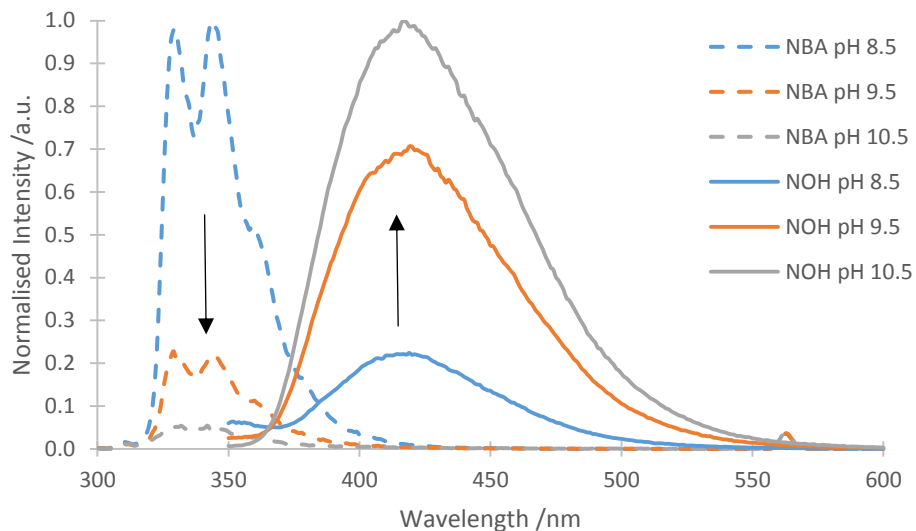
Figure 3.17 Fluorescence of the NBA and NOH as a function of pH, \lambda_{\text{ex}} = 280 \text{ nm} , [\text{NBA}] = 25 \mu\text{M} , [\text{NOH}] = 25 \mu\text{M} .
