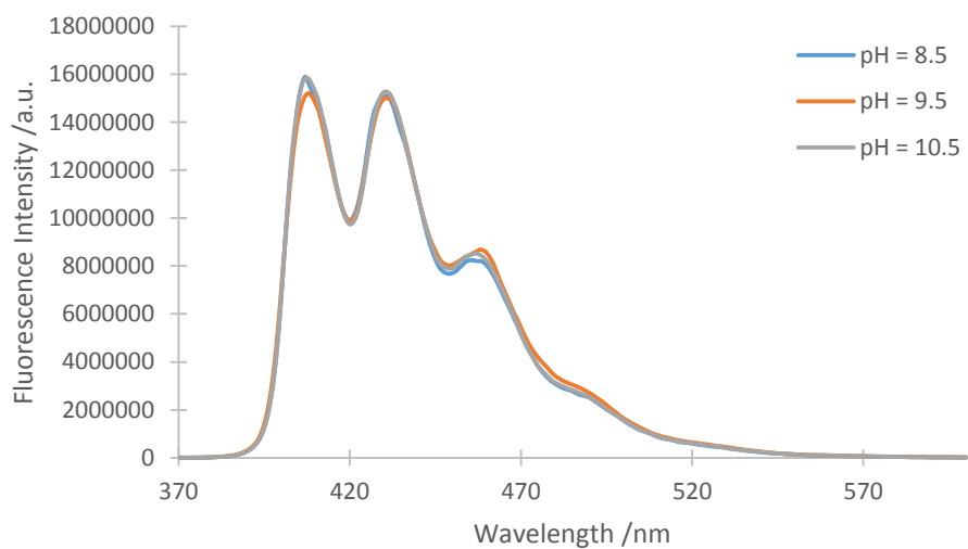
Appendix 4 Fluorescence of the ADMA as a function of pH, [ADMA] = 25 μM, λ ex = 360 nm.
