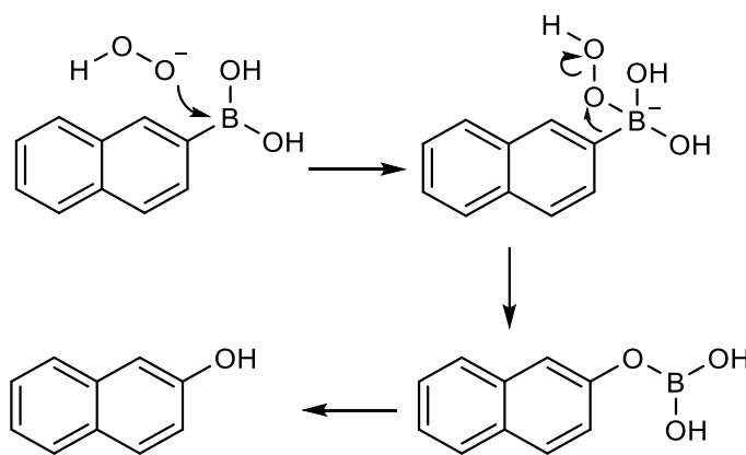
Figure 1.27 Mechanism of naphthol generation from arylboronic acid.
