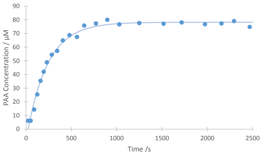
Figure 4.6 The formation of PAA during perhydrolysis reaction of TAED and SPC (1:3 ratio, pH 10.5), determined by the fluorometric titration with NBA, [TAED] = 25 \mu\text{M} , [SPC] = 75 \mu\text{M} , [NBA] = 250 \mu\text{M} , \lambda_{\text{ex}} = 340 nm, \lambda_{\text{em}} = 420 nm.
