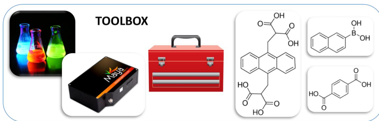
Figure 3.31 Toolbox of molecular probes for ROS detection in laundry applications.
