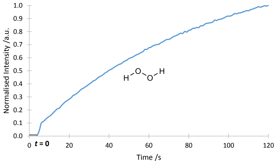
Figure 3.26 NOH fluorescence as a function of time in the presence of hydrogen peroxide, pH 10.5. \text{H}_2\text{O}_2 was added to the mixture in the 4 th second of measurement, pH 10.5, [NBA] = 250 \mu M, [ \text{H}_2\text{O}_2 ] = 50 \mu M, \lambda_{\text{ex}} = 340 nm, \lambda_{\text{em}} = 420 nm. Blue colour indicates the hydrogen peroxide.
