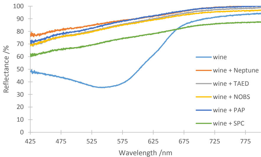
Figure 6.9 Reflectance spectra of the red wine stains before and after 45 min treatment with Neptune, TAED, NOBS, PAP and SPC, [Neptune] = 5000 mg/L, [TAED + SPC] = 1000 \mu M + 3000 \mu M, [NOBS + SPC] = 1000 \mu M + 3000 \mu M, [PAP] = 1000 \mu M, [SPC] = 1000 \mu M.
