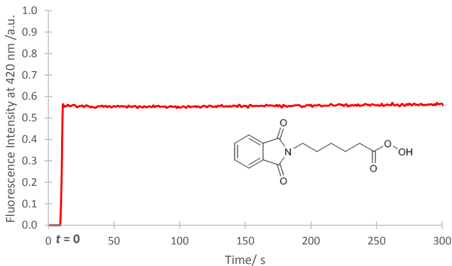
Figure 4.3 Fluorescence of NOH obtained after mixing PAP and NBA, recorder at 420 nm as a function of time ( \lambda_{\text{ex}} = 340 \text{ nm} ) in pH 10.5, [\text{PAP}] = 50 \mu\text{M} , [\text{NBA}] = 250 \mu\text{M} , \lambda_{\text{ex}} = 340 \text{ nm} , \lambda_{\text{em}} = 420 \text{ nm} .
