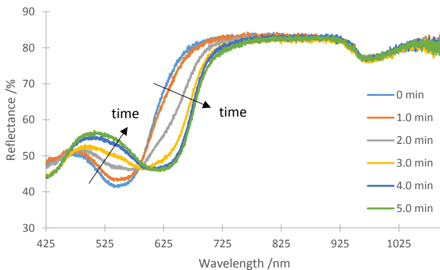
Figure 6.12 Reflectance spectra of red wine stain during treatment with Neptune over 5 min.
