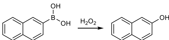
Figure 3.16 Reaction of 2-naphthylboronic acid with hydrogen peroxide which results in the generation of fluorescent 2-naphthol.
