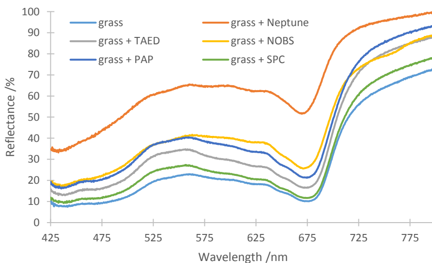
Figure 6.10 Reflectance spectra of the grass stains before and after 45 min treatment with Neptune, TAED, NOBS, PAP and SPC, [Neptune] = 5000 mg/L, [TAED + SPC] = 1000 \mu M + 3000 \mu M, [NOBS + SPC] = 1000 \mu M + 3000 \mu M, [PAP] = 1000 \mu M, [SPC] = 1000 \mu M.
