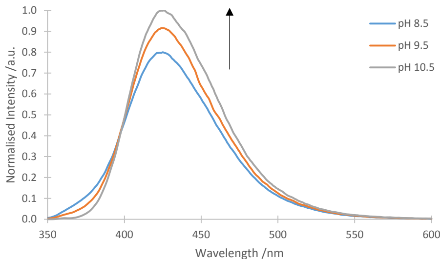
Figure 3.5 HTA fluorescence as a function of pH, \lambda_{\text{ex}} = 340 \text{ nm}
