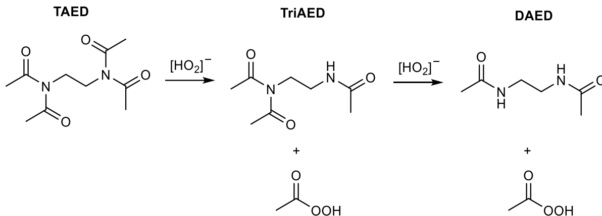
Figure 1.11 Perhydrolysis reaction of TAED.
