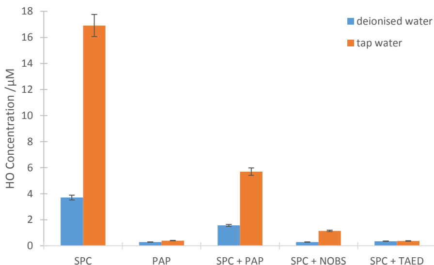
Figure 4.13 Hydroxyl radicals generated from bleach sources at 60 °C within 45 min.
