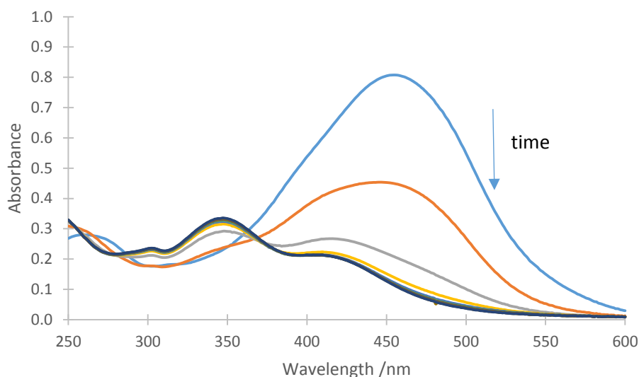
Figure 5.13 Bleaching of CUR with PAA at pH 10.5. [CUR] = 10 \mu M, [PAA] = 100 \mu M, in sodium bicarbonate buffer (0.1 M), total time = 10 min, measurement taken every 1 min.
