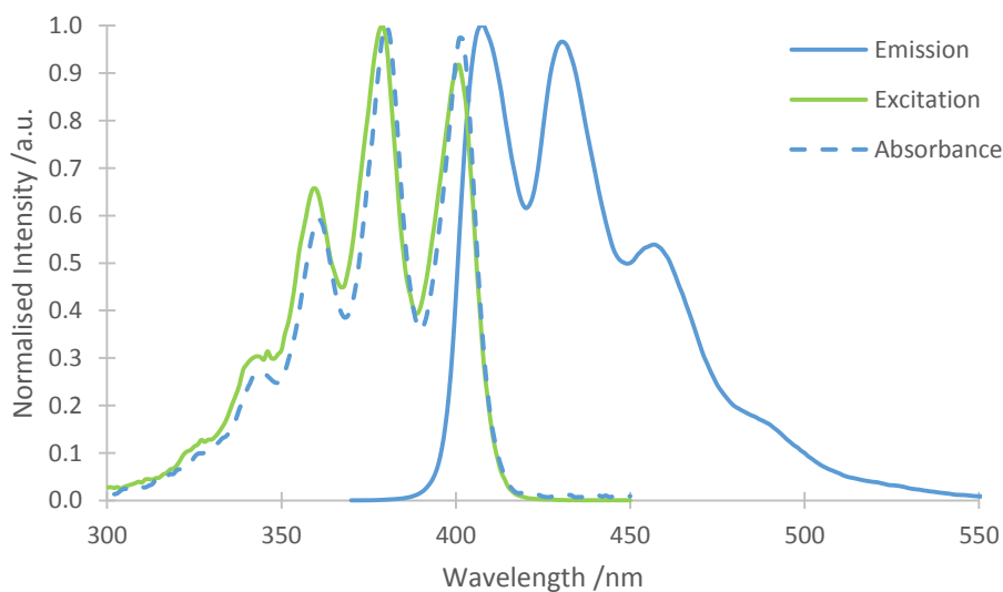
Figure 3.13 Spectral characteristics of the ADMA probe at pH = 10.5, [ADMA] = 25 \mu\text{M} , \lambda_{\text{ex}} = 360 nm, \lambda_{\text{em}} = 420 nm.
