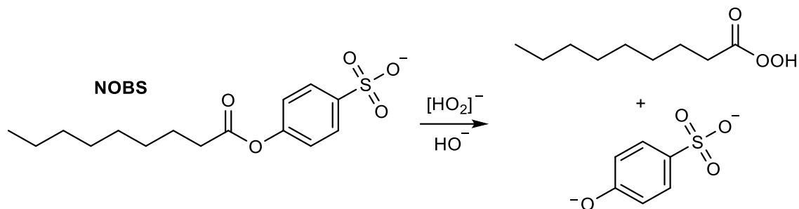
Figure 1.12 Perhydrolysis reaction of NOBS in pH 10.5.
