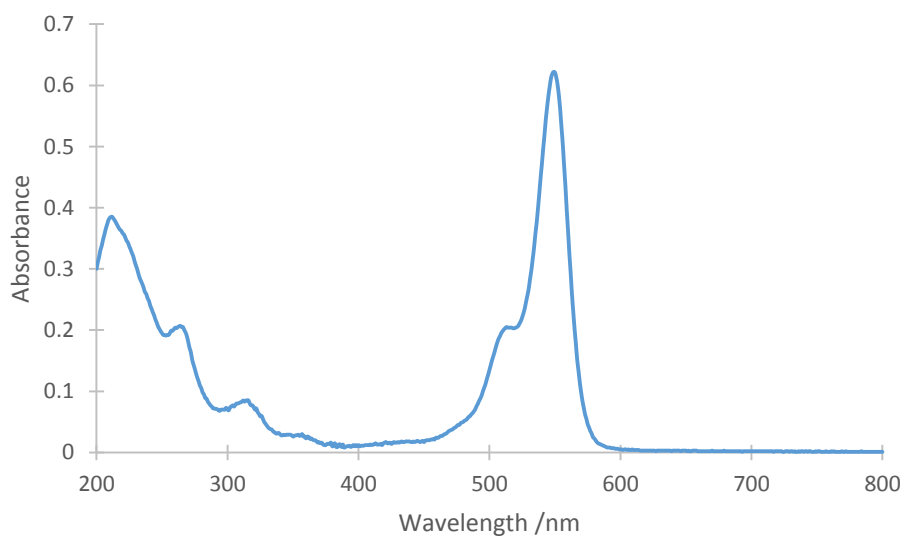
Figure 3.9 Absorbance of the RB in pH = 10.5, [RB] = 50 \mu M.
