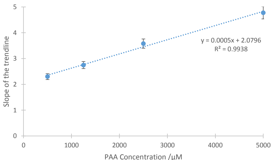
Figure 4.11 Determination of the order of the decomposition reaction. [\text{ADMA}] = 100 \mu\text{M} , \lambda_{\text{ex}} = 360 \text{ nm} , \lambda_{\text{em}} = 410 \text{ nm} .
