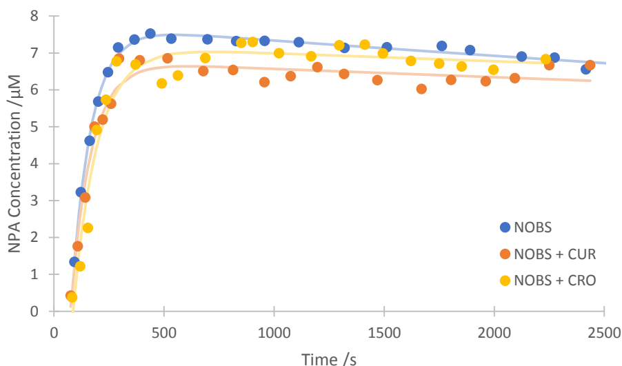
Figure 5.24 Time-concentration profiles of NPA generated from NOBS in presence of CUR and CRO in pH 10.5, over 45 min, [\text{NOBS}] = 10 \mu\text{M} , [\text{SPC}] = 30 \mu\text{M} , [\text{CUR}, \text{CRO}] = 2 \mu\text{M} , [\text{NBA}] = 250 \mu\text{M} , \lambda_{\text{ex}} = 365 \text{ nm} , \lambda_{\text{em}} = 420 \text{ nm} .
