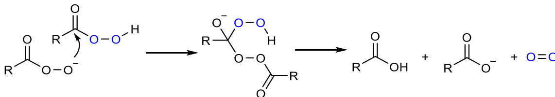
Figure 1.16 Decomposition of peroxydicarboxylic acid.
