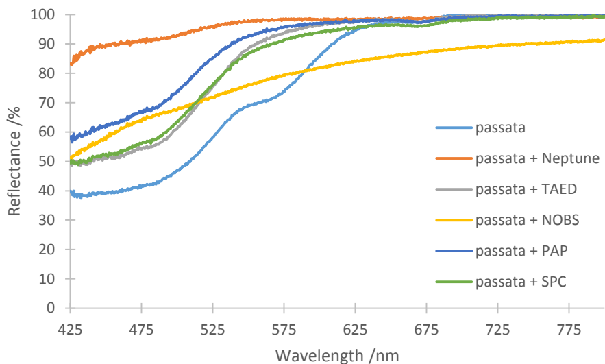
Figure 6.11 Reflectance spectra of the tomato stains before and after 45 min treatment with Neptune, TAED, NOBS, PAP and SPC, [Neptune] = 5000 mg/L, [TAED + SPC] = 1000 \mu M + 3000 \mu M, [NOBS + SPC] = 1000 \mu M + 3000 \mu M, [PAP] = 1000 \mu M, [SPC] = 1000 \mu M.
