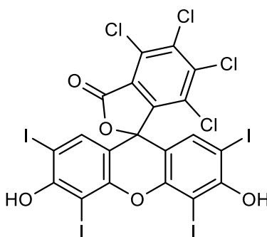
Figure 3.7 Structure of Rose Bengal.
