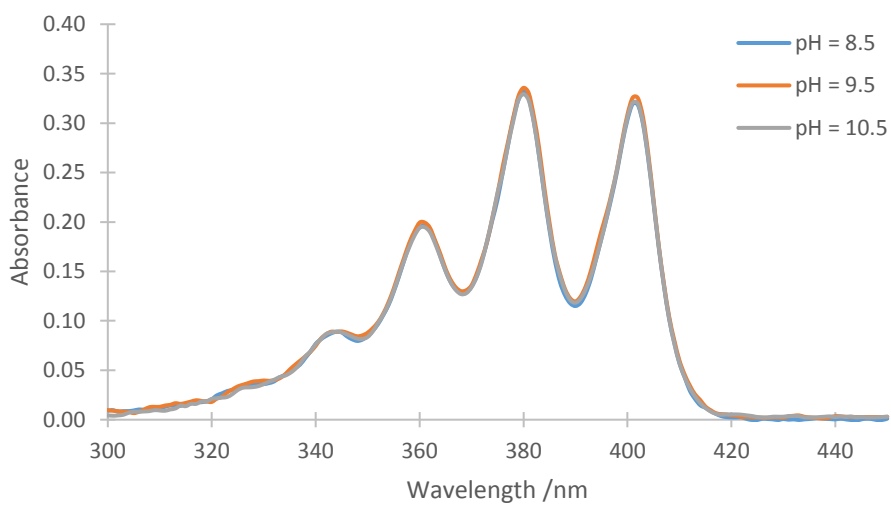
Appendix 6 Absorbance of the ADMA as a function of pH, [ADMA] = 25 \mu M.
