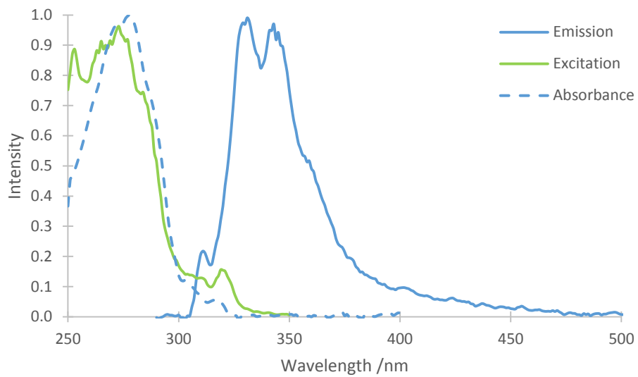
Appendix 7 Spectral characteristic of the NBA in pH = 8.5, [NBA] = 10 \mu M, \lambda_{\text{ex}} = 280 nm, \lambda_{\text{em}} = 340 nm.
