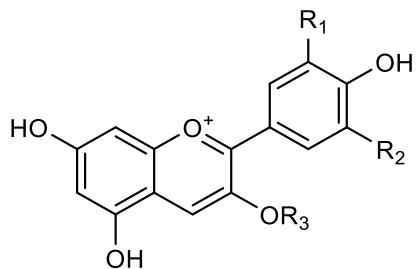
Figure 6.3 The basic chemical structure of anthocyanins - glycosides of anthocyanidins.
