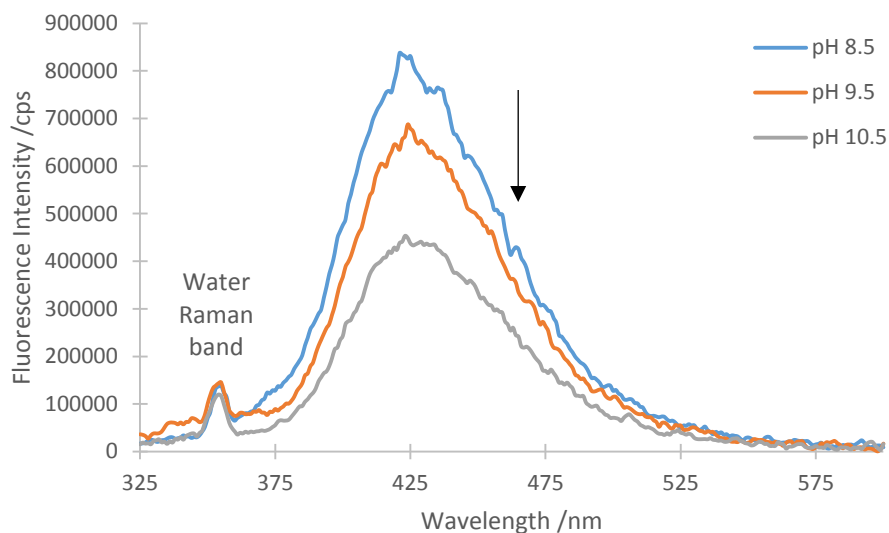
Figure 3.15 HTA fluorescence after 30 min in CuO assay of H 2 O 2 detection. [CuO] = 50 μM, [H 2 O 2 ] = 100 μM, [TA] = 250 μM, λ ex = 315 nm.
