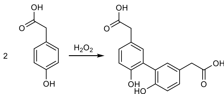
Figure 1.22 Reaction of PHPAA with hydrogen peroxide.
