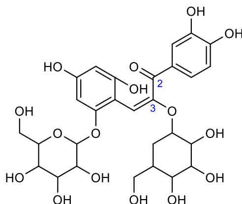
Figure 5.18 Structure of chalcone form of cyanin (pH > 7).
