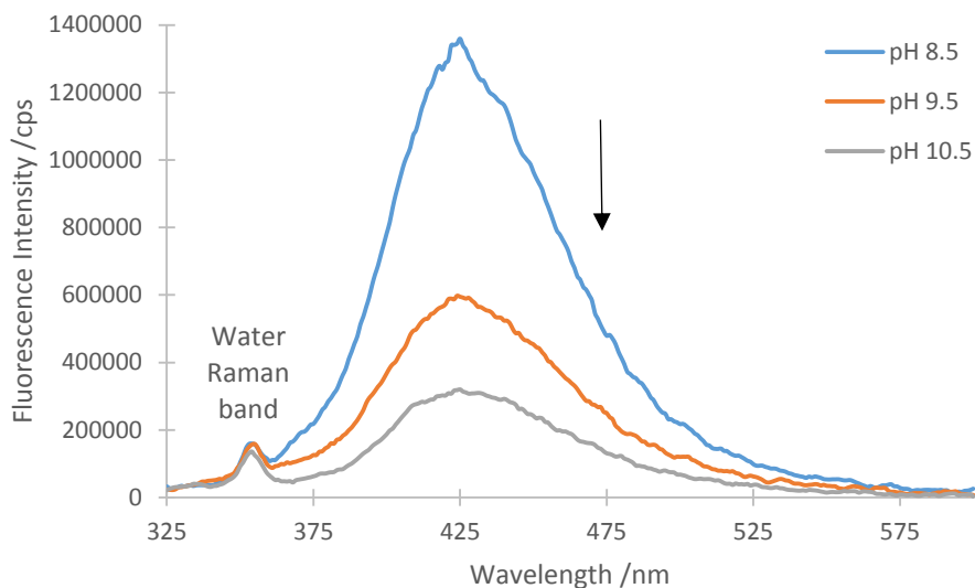
Figure 3.1 Generation of hydroxyl radicals by the Fenton reaction with TA detection in alkaline pH.
