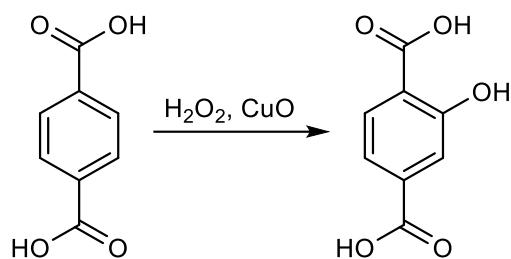
Figure 1.25 Generation of HTA after catalytic decomposition of hydrogen peroxide by CuO nanoparticles.
