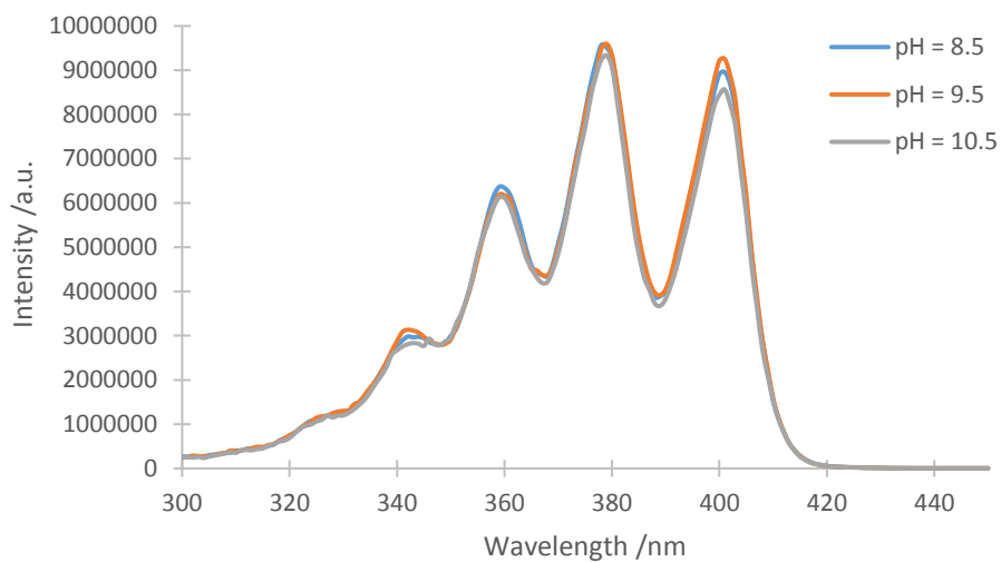
Appendix 5 Excitation spectra of the ADMA as a function of pH, [ADMA] = 25 \mu M, \lambda_{em} = 420 nm.
