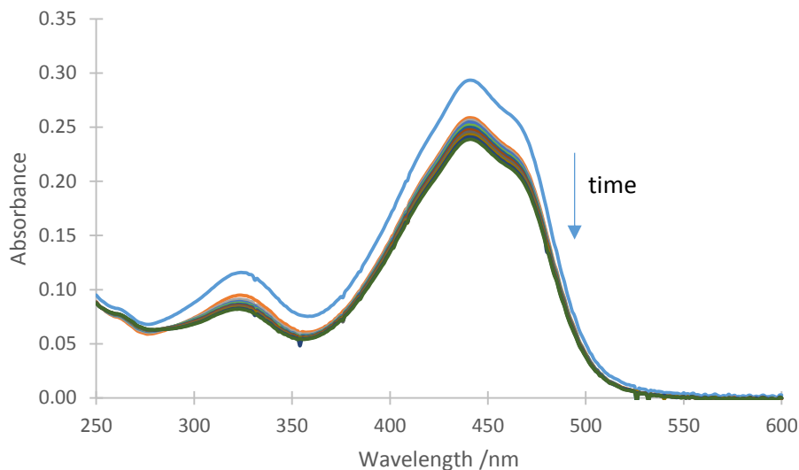
Figure 5.17 Bleaching of CRO with PAP at pH 7.5. [CRO] = 10 \mu M, [PAP] = 100 \mu M, in phosphate buffer (0.1 M), total time = 10 min, measurement taken every 1 min.
