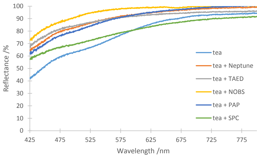
Figure 6.8 Reflectance spectra of the tea stains before and after 45 min treatment with Neptune, TAED, NOBS, PAP and SPC, [Neptune] = 5000 mg/L, [TAED + SPC] = 1000 \mu M + 3000 \mu M, [NOBS + SPC] = 1000 \mu M + 3000 \mu M, [PAP] = 1000 \mu M, [SPC] = 1000 \mu M.
