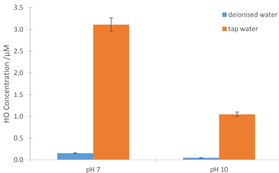
Figure 4.14 Hydroxyl radicals generated by acoustic cavitation, [\text{TA}] = 100 \mu\text{M} , t = 60 \text{ min} , \lambda_{\text{ex}} = 315 \text{ nm} .
