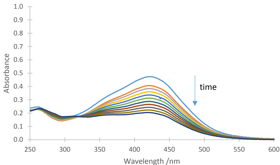
Figure 5.16 Bleaching of CUR with PAA at pH 7.5. [CUR] = 10 \mu M, [PAA] = 100 \mu M, in phosphate buffer (0.1 M), total time = 10 min, measurement taken every 1 min.
