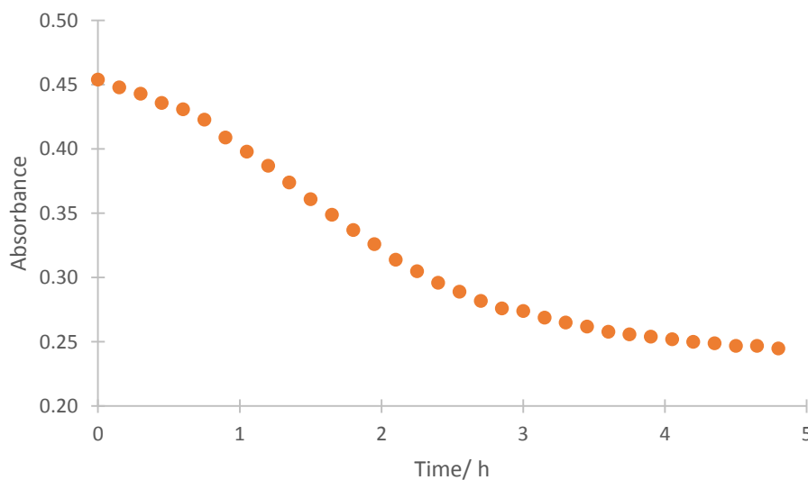
Figure 5.21 Absorbance at 420 nm of CUR while bleaching by PAP over 5 hours in pH 10.5, [CUR] = 25 \mu M, [PAP] = 250 \mu M.
