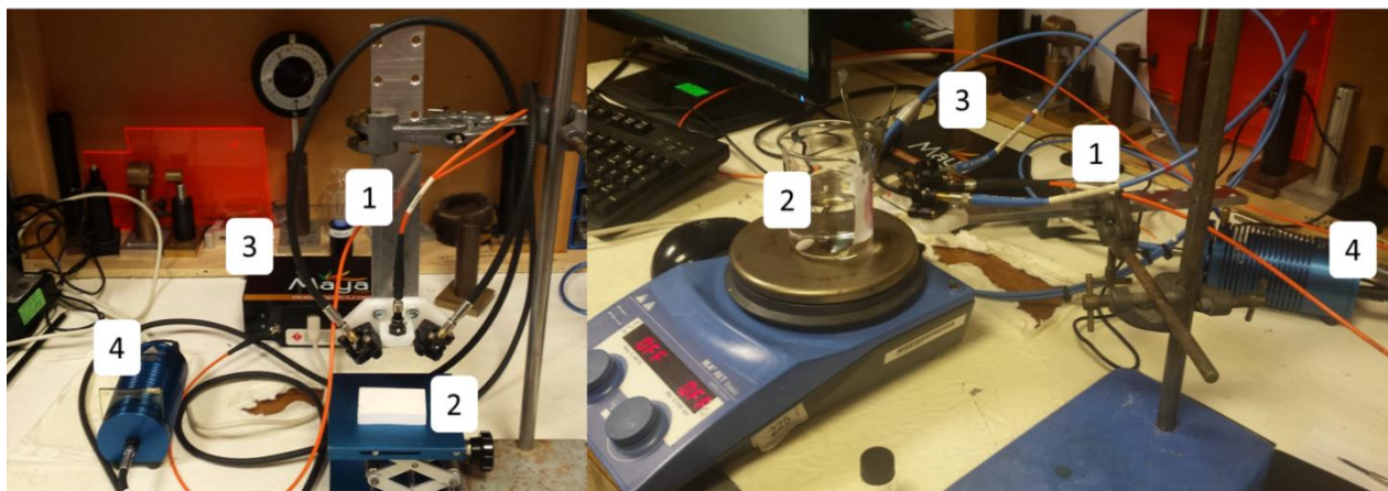
Figure 2.5 Vertical and horizontal configuration of the diffuse reflectance setup, 1 – reflectance head, 2 – sample, 3 – detector (spectrometer) and 4 – source of light + filter.
