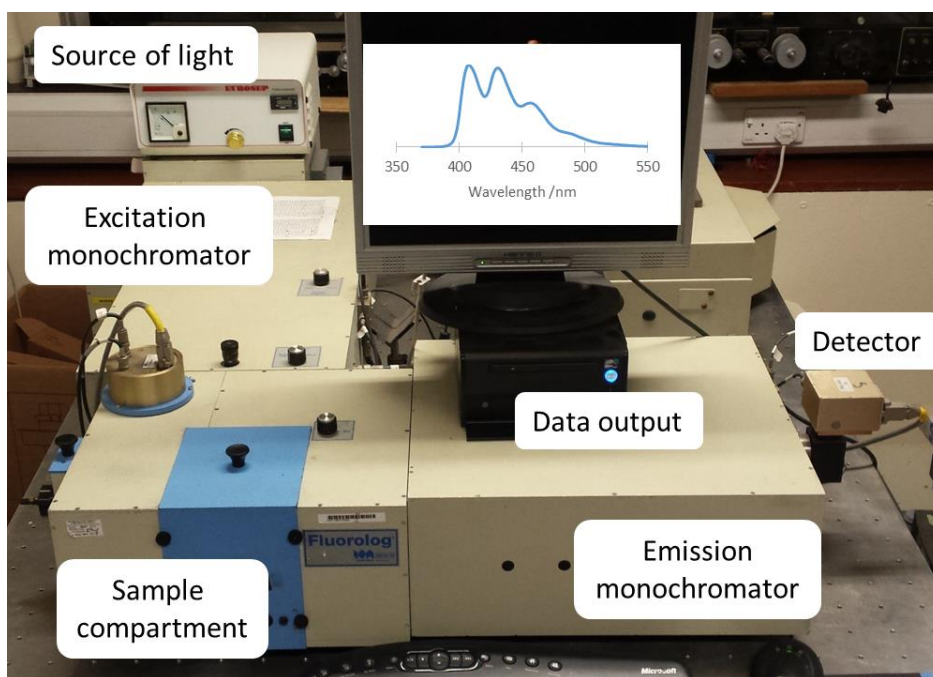
Figure 2.3 Spectrofluorimeter Fluorolog 3-22.
