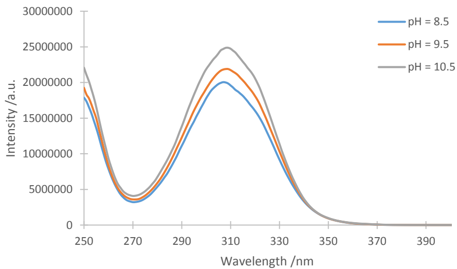
Appendix 2 HTA excitation spectra as a function of pH, [HTA] = 10 \mu M, \lambda_{em} = 320 nm.
