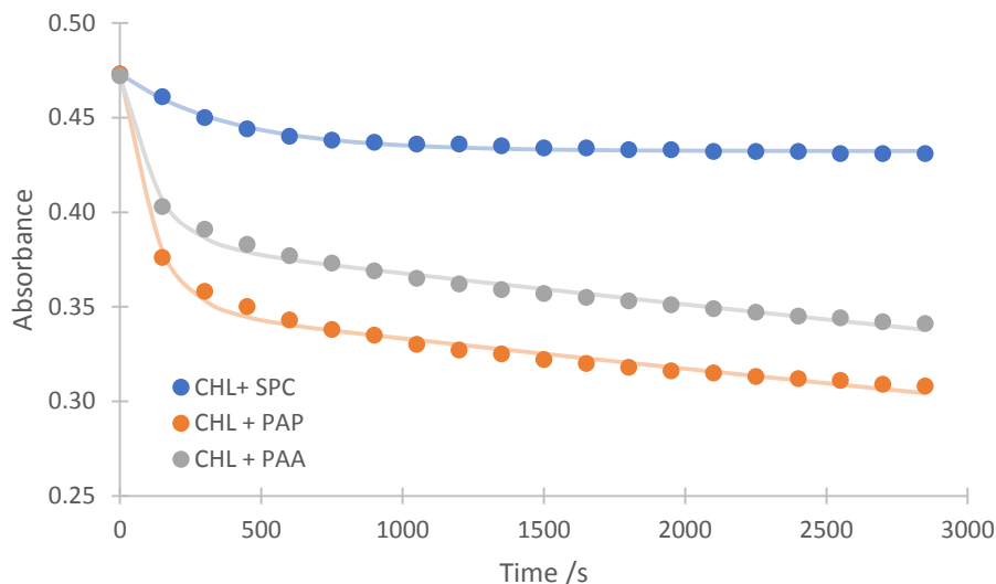
Figure 5.19 Absorbance of the CHL at 630 nm during bleaching by SPC, PAP and PAA over 45 min in pH 10.5, [CHL] = 25 \mu M, [SPC, PAP, PAA] = 250 \mu M.
