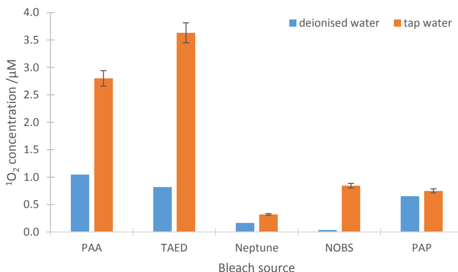
Figure 4.10 Singlet oxygen generated from bleach sources in 45 min in pH 10.5, [\text{ADMA}] = 100 \mu\text{M} , [\text{PAA}, \text{PAP}, \text{TAED}, \text{NOBS}] = 500 \mu\text{M} , [\text{SPC}] = 1500 \mu\text{M} , [\text{Neptune}] = 5000 \text{ mg/L} , \lambda_{\text{ex}} = 360 \text{ nm} , \lambda_{\text{em}} = 410 \text{ nm} .
