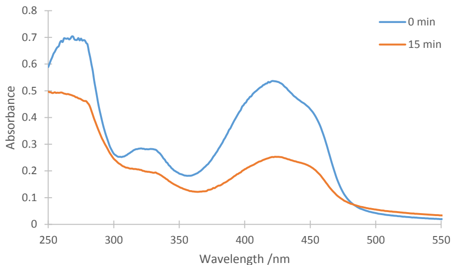
Figure 3.11 Decomposition of the DPBF in pH 10.5 buffered solution when exposed to sunlight, [DPBF] = 60 \mu M.
