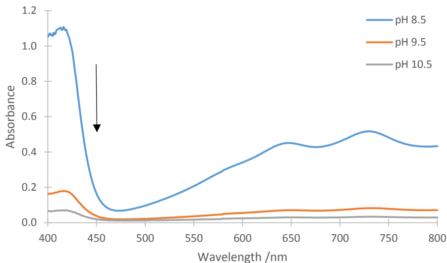
Figure 3.22 Absorbance of the ABTS radical cation as a function of pH, [ABTS] = 50 \mu M, [PAA] = 10 \mu M.
