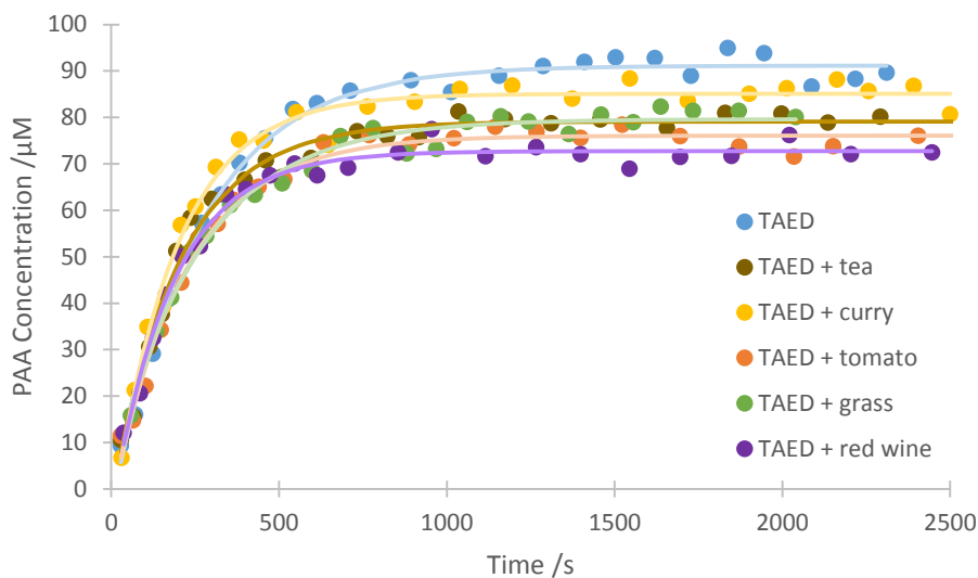
Figure 6.15 Time-concentration profile of PAA, generated from TAED in presence of stains, pH 10.5, [TAED] = 50 \mu\text{M} , [SPC] = 150 \mu\text{M} , two stains of curry, grass, tomato, wine and tea per experiment, [NBA] = 250 \mu\text{M} , \lambda_{\text{ex}} = 365 nm, \lambda_{\text{em}} = 420 nm.
