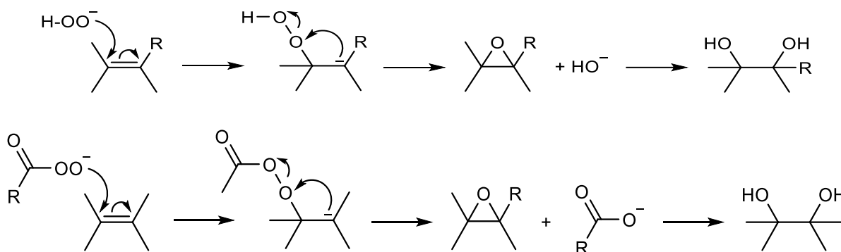
Figure 1.17 Bleaching by perhydroxyl ion and peroxy acid anion through nucleophilic attack on an alkene group. R is an electron-withdrawing group.
