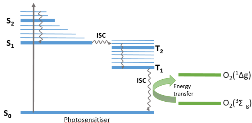
Figure 3.8 Generation of singlet oxygen by photosensitiser.
