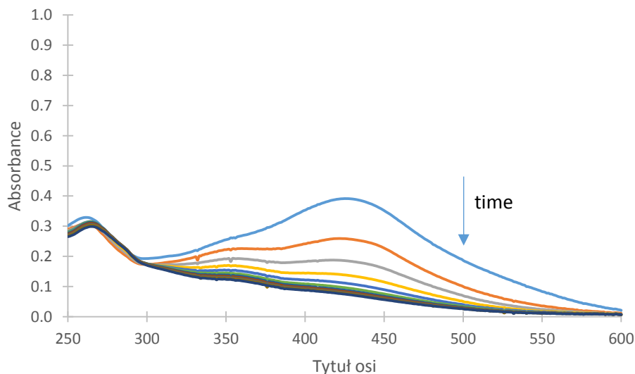
Figure 5.15 Bleaching of CUR with PAA at pH 8.5. [CUR] = 10 \mu M, [PAA] = 100 \mu M, in borax buffer (0.1 M), total time = 10 min, measurement taken every 1 min.
