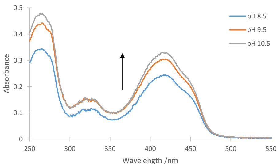
Figure 3.10 DPBF absorbance as a function of pH, [DPBF] = 50 \mu M.
