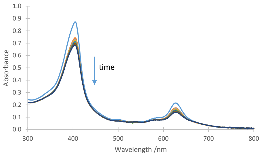
Figure 5.11 Bleaching of CHL with PAA at pH 10.5. [CHL] = 10 \mu M, [PAA] = 100 \mu M, in sodium bicarbonate buffer (0.1 M), total time = 10 min, measurement taken every 1 min.
