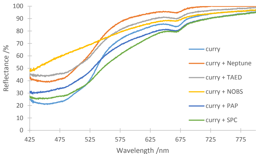
Figure 6.7 Reflectance spectra of curry stains before and after 45 min treatment with Neptune, TAED, NOBS, PAP and SPC, [Neptune] = 5000 mg/L, [TAED + SPC] = 1000 \mu M + 3000 \mu M, [NOBS + SPC] = 1000 \mu M + 3000 \mu M, [PAP] = 1000 \mu M, [SPC] = 1000 \mu M.
