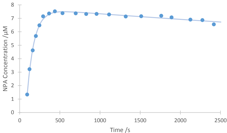
Figure 4.8 The formation of NPA during the perhydrolysis reaction of NOBS and SPC (1:3 ratio, pH 10.5), determined by the fluorometric titration with NBA, [NOBS] = 25 \mu\text{M} , [SPC] = 75 \mu\text{M} , [NBA] = 250 \mu\text{M} , \lambda_{\text{ex}} = 340 nm, \lambda_{\text{em}} = 420 nm.
