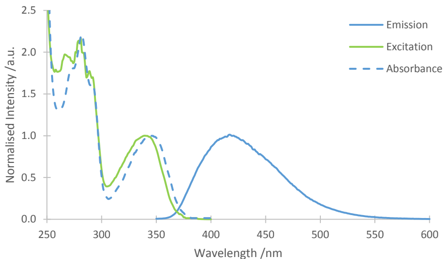
Figure 3.18 Spectral characteristic of the NOH in pH = 10.5, \lambda_{\text{ex}} = 340 \text{ nm} , \lambda_{\text{em}} = 420 \text{ nm} , [\text{NOH}] = 25 \mu\text{M} .
