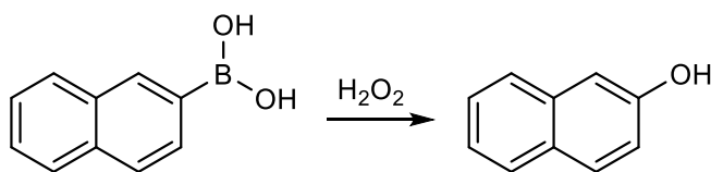
Figure 1.26 Reaction of 2-naphthylboronic acid with hydrogen peroxide.
