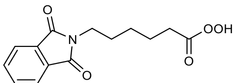
Figure 1.15 Structure of PAP.
