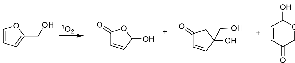
Figure 1.30 Reaction of FFA with singlet oxygen.
