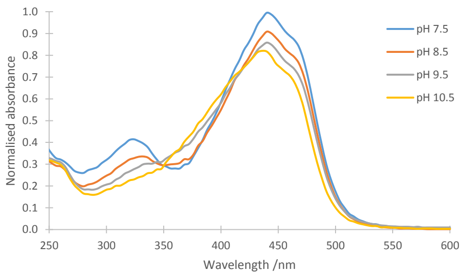
Figure 5.6 Absorbance of the CRO as a function of pH. [CRO] = 25 \mu M in buffer solutions (0.1 M).
