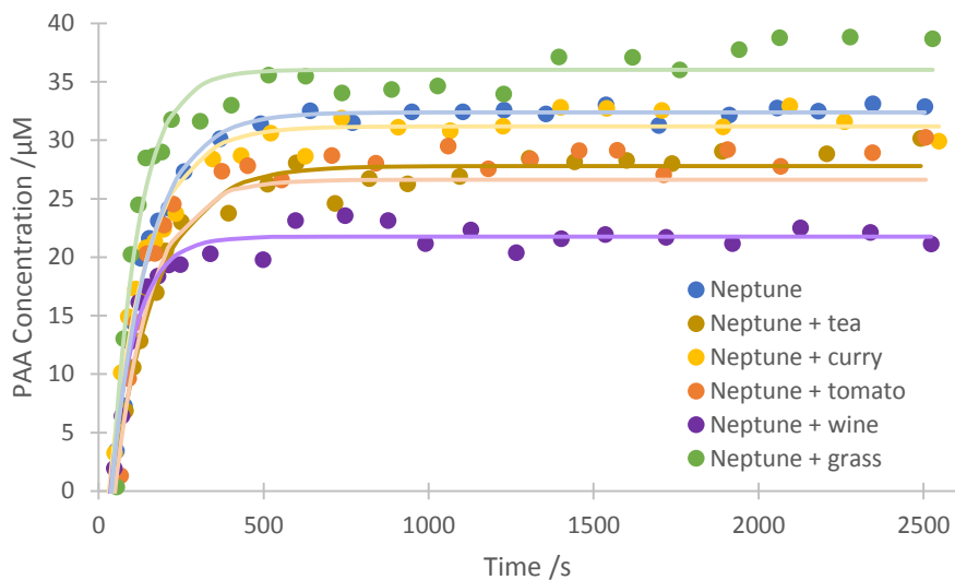
Figure 6.17 Time-concentration profile of PAA, generated from Neptune in presence of stains, pH 10.5, [Neptune] = 5000 mg/L, [NBA] = two stains of tea, curry, tomato, wine and grass per experiment, [NBA] = 250 \mu M, \lambda_{\text{ex}} = 365 nm, \lambda_{\text{em}} = 420 nm.
