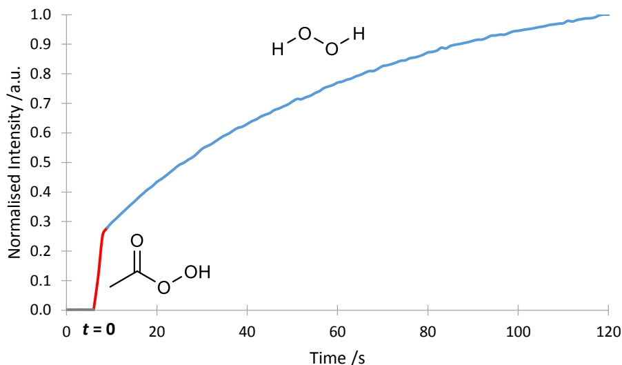
Figure 3.27 NBA fluorescence as a function of time in the presence of peroxyacid and hydrogen peroxide. PAA and \text{H}_2\text{O}_2 were added to the mixture in the 6 th second of measurement, pH 10.5, [\text{NBA}] = 250 \mu\text{M} , [\text{PAA}] = 25 \mu\text{M} , [\text{H}_2\text{O}_2] = 25 \mu\text{M} , \lambda_{\text{ex}} = 340 \text{ nm} , \lambda_{\text{em}} = 420 \text{ nm} . Red colour indicates the peroxy acid and blue the hydrogen peroxide.
