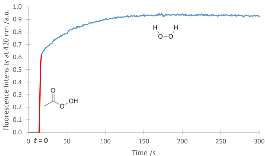
Figure 4.5 Fluorescence of NOH obtained after mixing TAED, SPC and NBA, recorded at 420 nm as a function of time ( \lambda_{\text{ex}} = 340 \text{ nm} , \lambda_{\text{em}} = 420 \text{ nm} ) in pH 10.5. The rapid rise (red) is attributed to the presence of formed PAA, and slow rise (blue) to the presence of hydrogen peroxide. [\text{TAED}] = 25 \mu\text{M} , [\text{SPC}] = 75 \mu\text{M} , [\text{NBA}] = 250 \mu\text{M} .
