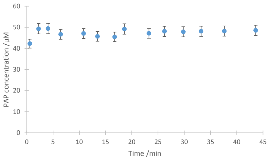
Figure 4.4 Stability of the PAP (50 \mu\text{M} ) in pH 10.5 confirmed with NBA (250 \mu\text{M} ) fluorescent assay, \lambda_{\text{ex}} = 340 \text{ nm} , \lambda_{\text{em}} = 420 \text{ nm} .
