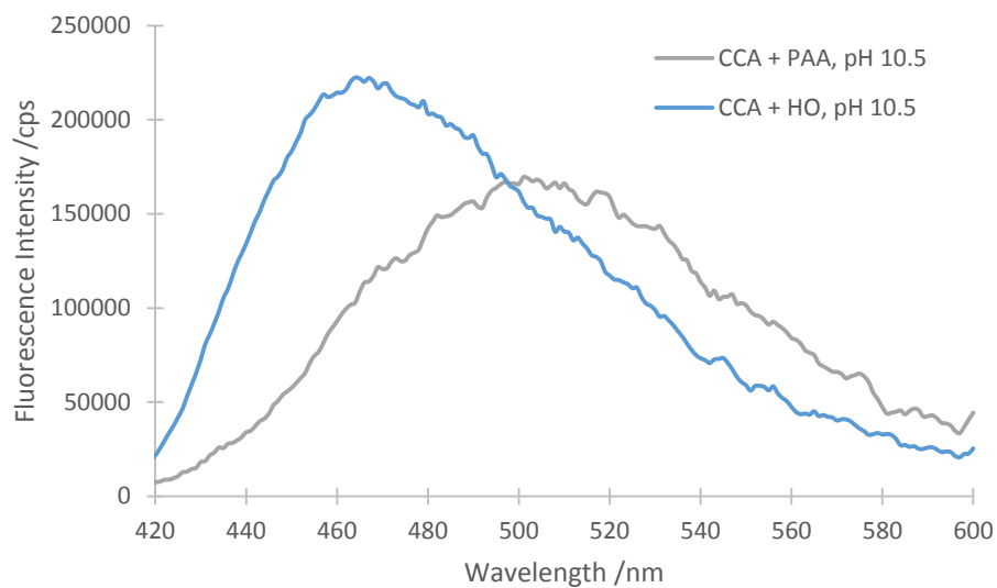
Appendix 3 Fluorescence of HO-CCA, after reaction of CCA with PAA and HO • , in pH 10.5, [CCA] = 10 μM, [PAA] = 50 μM, [KNO 3 ] = 250 μM, λ ex = 410 nm.
