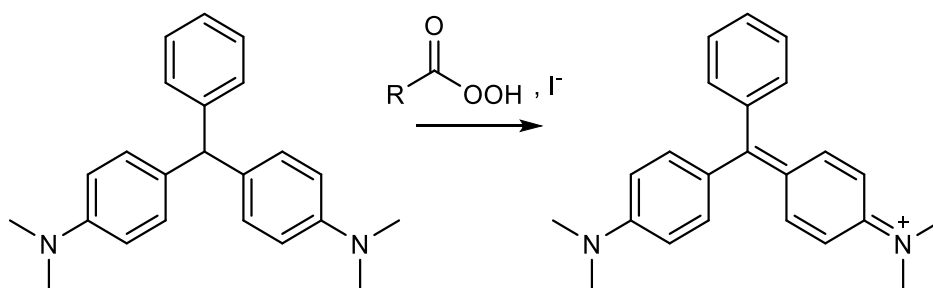
Figure 1.28 Reaction of leucomalachite green with peroxy acid.
