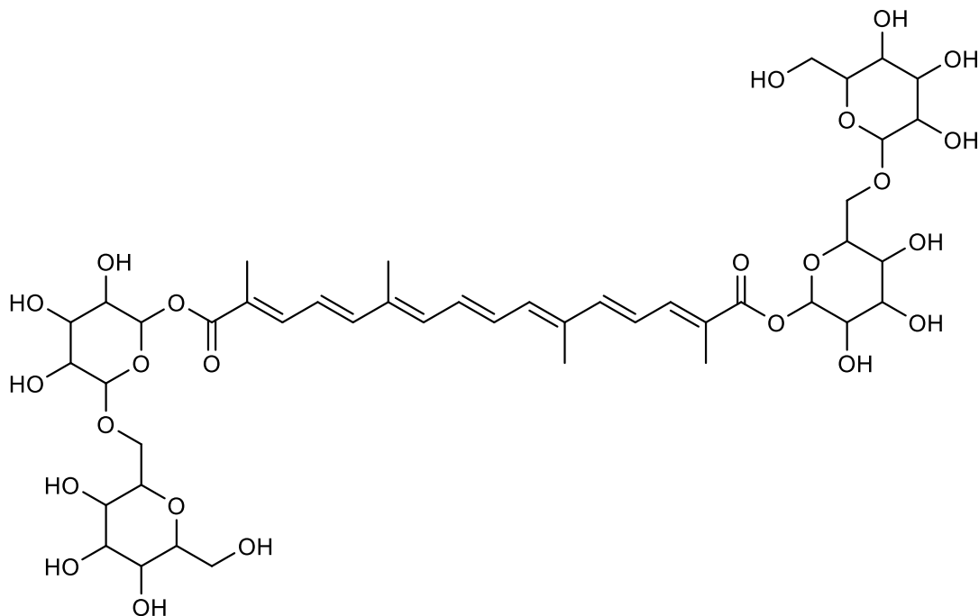
Figure 5.5 Structure of crocin.
