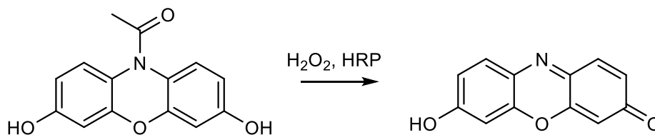
Figure 1.24 Reaction of Amplex Red with hydrogen peroxide to yield resourfin.
