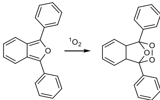
Figure 1.31 Reaction of DPBF with singlet oxygen.
