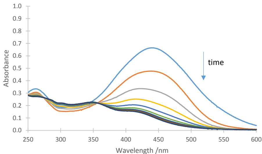
Figure 5.14 Bleaching of CUR with PAA at pH 9.5. [CUR] = 10 \mu M, [PAA] = 100 \mu M, in borax buffer (0.1 M), total time = 10 min, measurement taken every 1 min.
