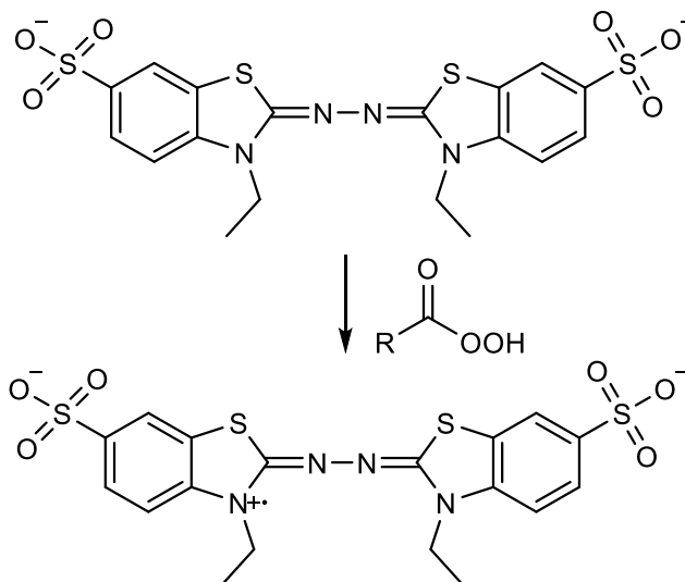
Figure 1.29 Reaction of ABTS with peroxy acid.
