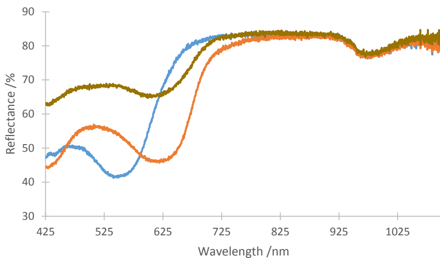
Figure 6.13 Reflectance spectra of red wine stain during treatment with Neptune over 45 min, [Neptune] = 5000 mg/L. Blue line: t < 0 min (without Neptune), orange line: t = 0 min (with Neptune), brown line: t = 45 min (bleaching).
