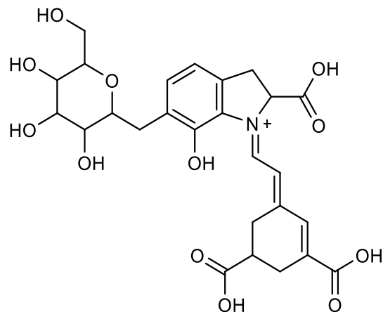
Figure 5.9 Structure of betanin.
