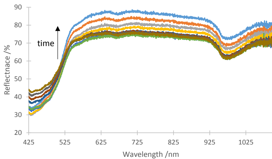
Figure 6.14 Reflectance spectra of tomato stain during treatment with Neptune over 45 min. Measurement taken every 5 min, [Neptune] = 5000 mg/L.
