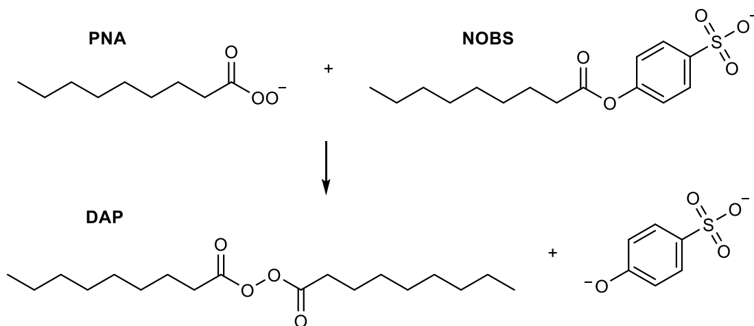
Figure 1.13 The formation of DAP.
