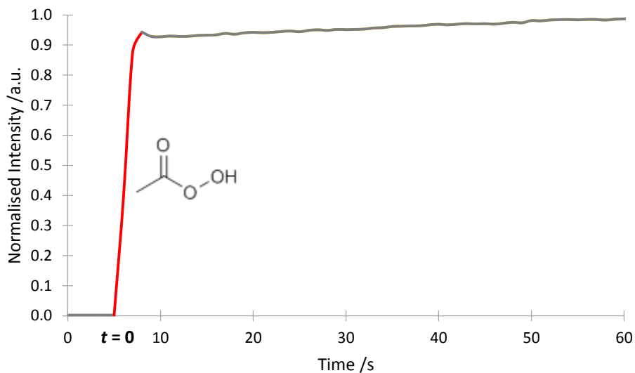
Figure 3.25 NOH fluorescence as a function of time, after the reaction between NBA and PAA, pH 10.5. PAA was added to the mixture in the 5 th second of measurement, pH 10.5, [NBA] = 250 \mu M, [PAA] = 50 \mu M, \lambda_{\text{ex}} = 340 nm, \lambda_{\text{em}} = 420 nm. Red colour indicates the peroxy acid.
