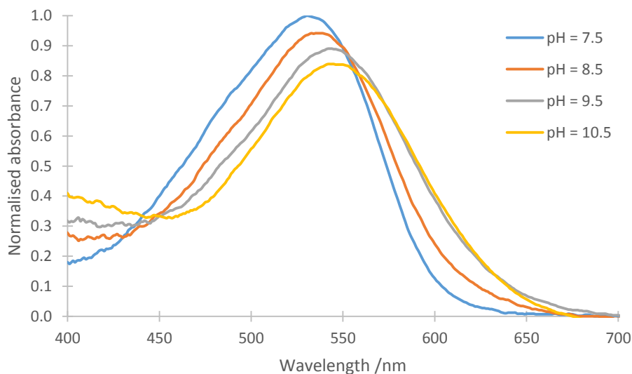
Figure 5.10 Absorbance of BET as a function of pH. [\text{BET}] = 200 \mu\text{M} in buffer solutions (0.1 M). Savitzky-Golay filter was used to smooth the spectra ( n=5 ).
