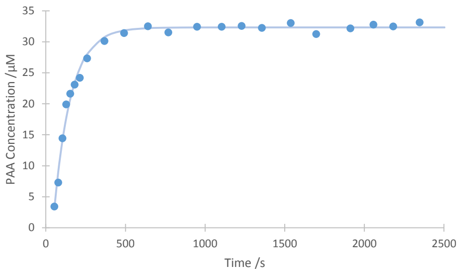
Figure 4.9 Time-concentration profile of PAA in Neptune sample, pH 10.5, [Neptune] = 5000 mg/L, [NBA] = 250 \mu M, \lambda_{\text{ex}} = 340 nm, \lambda_{\text{em}} = 420 nm.
