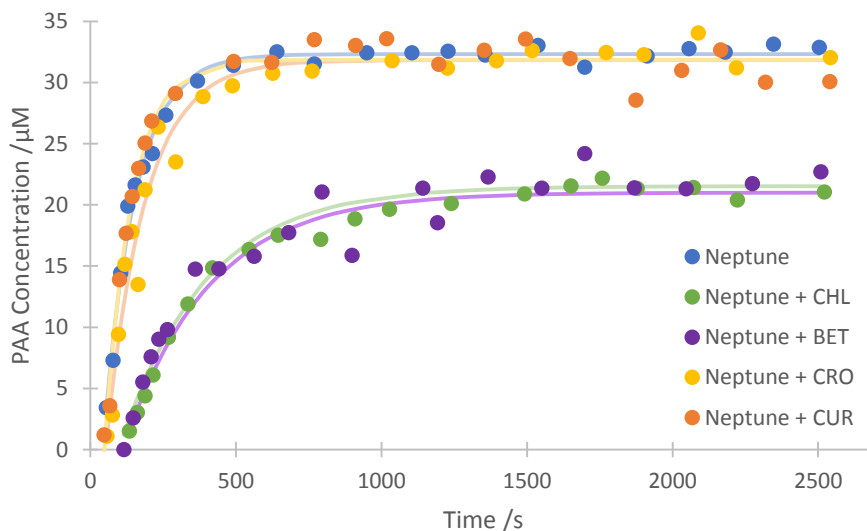
Figure 5.26 Time-concentration profiles of PAA generated from Neptune in presence of dyes in pH 10.5, over 45 min, [Neptune] = 5000 mg/L, [CHL, BET, CRO, CUR] = 4 µM, [NBA] = 250 µM, \lambda_{\text{ex}} = 365 \text{ nm} , \lambda_{\text{em}} = 420 \text{ nm} .
