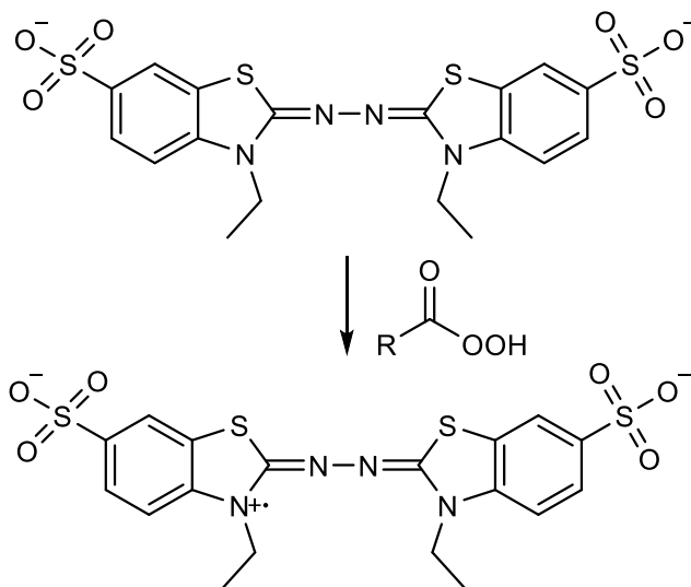
Figure 3.21 Reaction of ABTS with PAA results in ABTS radical cation.
