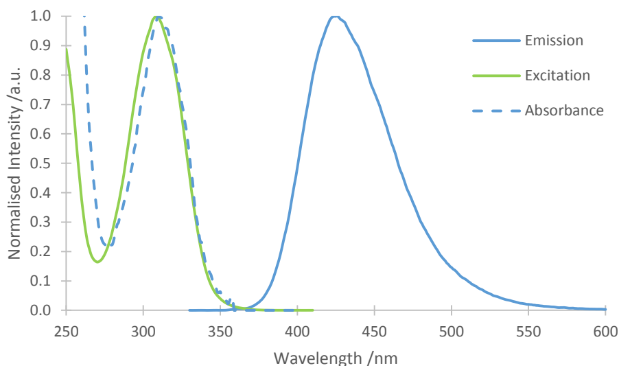
Figure 3.4 Spectral characteristic of HTA at pH = 10.5, \lambda_{\text{ex}} = 320 \text{ nm} , \lambda_{\text{em}} = 420 \text{ nm} .
