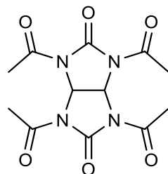
Figure 1.4 Structure of TAGU.
