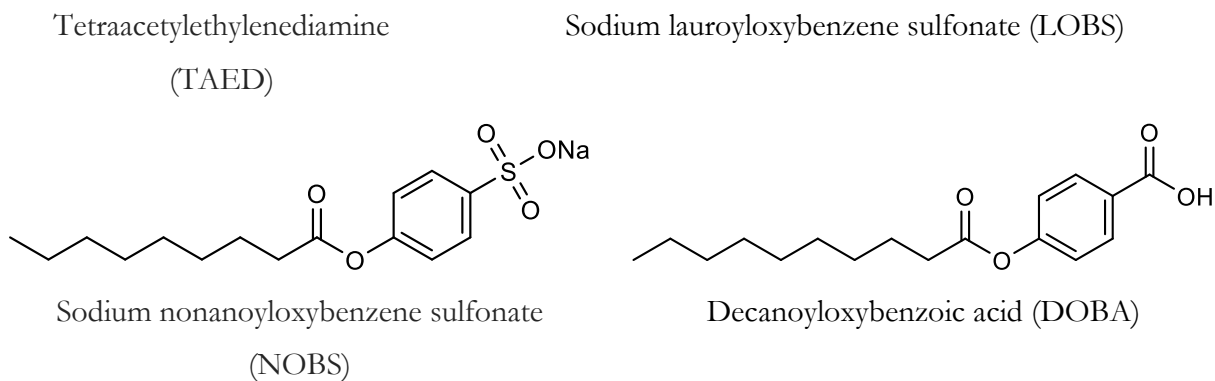
Figure 1.5 Currently used bleach activators.
