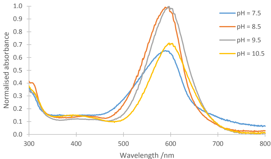
Figure 5.8 Absorbance of the CYN as a function of pH. [CYN] = 25 \mu M in buffer solutions (0.1 M).
