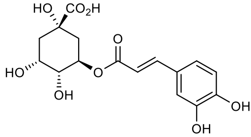
Figure 6.1 Structure of the chlorogenic acid.
