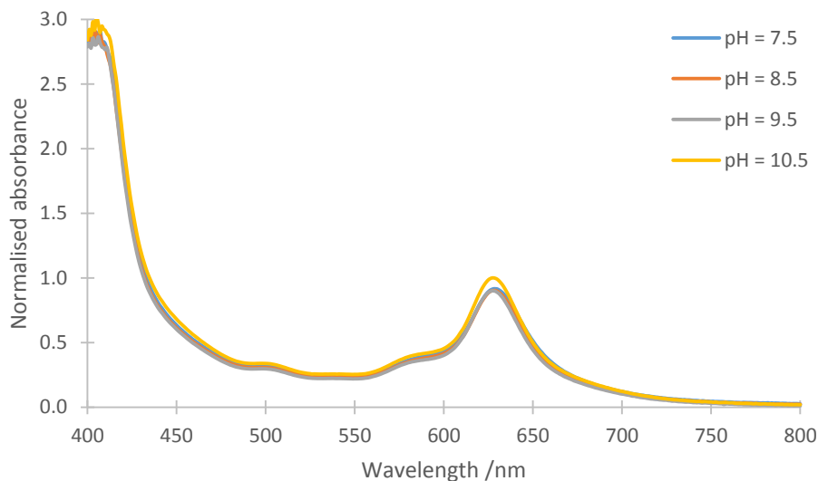
Figure 5.2 Absorbance of the CHL as a function of pH in visible region, [CHL] = 25 \mu M, in a buffer solutions (0.1 M).
