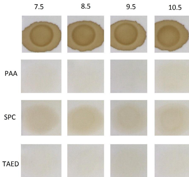
Figure 6.4 Pictures of coffee stains bleached by PAA, SPC and TAED over 45 min in alkaline pH range, [PAA] = 0.01 M, [SPC] = 0.01 M, [TAED + SPC] = 0.01 M + 0.03 M.
