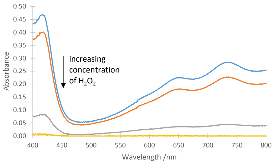
Figure 3.23 Absorbance of the mixtures of ADMA and H 2 O 2 with constant PAA concentration at pH = 8.5, [ABTS] = 100 \mu M, [PAA] = 20 \mu M, [H 2 O 2 ] = 5, 10, 20, 50 \mu M.
