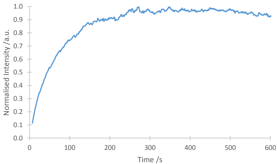
Figure 3.29 Fluorescence at 420 nm recorded using stopped flow during the reaction of NBA and \text{H}_2\text{O}_2 , pH 10.5, [NBA] = 50 \mu M, [ \text{H}_2\text{O}_2 ] = 20 \mu M, \lambda_{\text{ex}} = 340 nm, \lambda_{\text{em}} = 420 nm.
