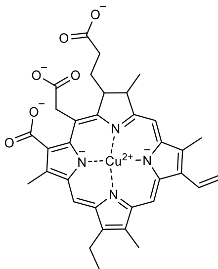
Figure 5.1 Structure of chlorophyllin.
