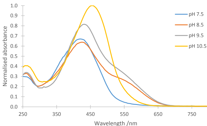
Figure 5.4 Absorbance of CUR as a function of pH, [CUR] = 25 \mu M in a buffer solutions (0.1 M) containing 0.3% of ethanol.
