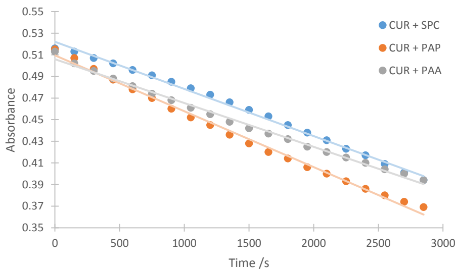
Figure 5.20 Absorbance of the CUR at 420 nm during bleaching by SPC, PAP and PAA over 45 min in pH 10.5, [\text{CUR}] = 25 \mu\text{M} , [\text{SPC}, \text{PAP}, \text{PAA}] = 250 \mu\text{M} .
