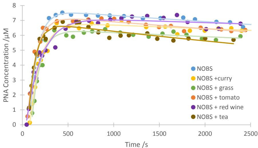
Figure 6.16 Time-concentration profiles of PNA, generated from NOBS in presence of stains, pH 10.5, [NOBS] = 10 \mu\text{M} , [SPC] = 30 \mu\text{M} , two stains of curry, grass, tomato, wine and tea per experiment, [NBA] = 250 \mu\text{M} , \lambda_{\text{ex}} = 365 nm, \lambda_{\text{em}} = 420 nm.
