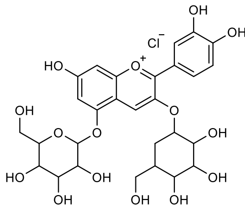
Figure 5.7 Structure of cyanin chloride (flavylium cation) at pH 1.
