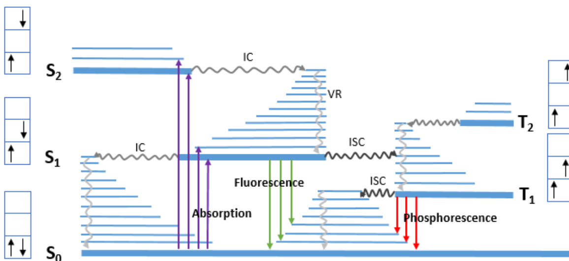
Figure 2.1 Jabłoński diagram
