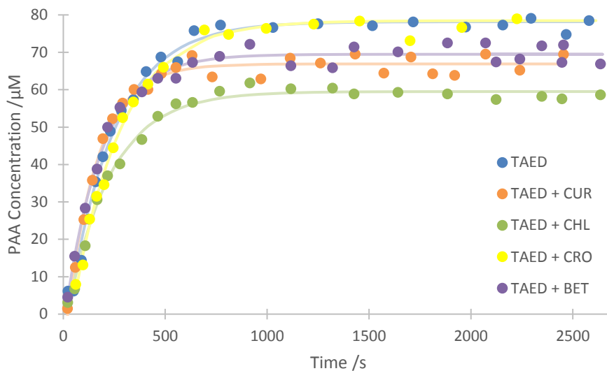
Figure 5.23 Time-concentration profiles of PAA generated from TAED in presence of dyes in pH 10.5, over 45 min, [TAED] = 50 \mu\text{M} , [SPC] = 150 \mu\text{M} , [CUR, CHL, CRO, BET] = 10 \mu\text{M} , [NBA] = 250 \mu\text{M} , \lambda_{\text{ex}} = 365 nm, \lambda_{\text{em}} = 420 nm.
