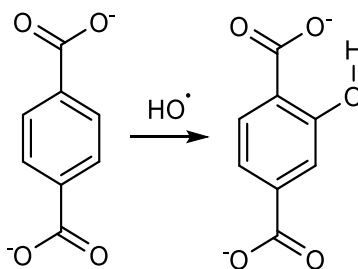
Figure 3.3 Reaction of terephthalic acid (TA) and hydroxyl radical which yields to 2-hydroxy-terephthalic acid (HTA).
