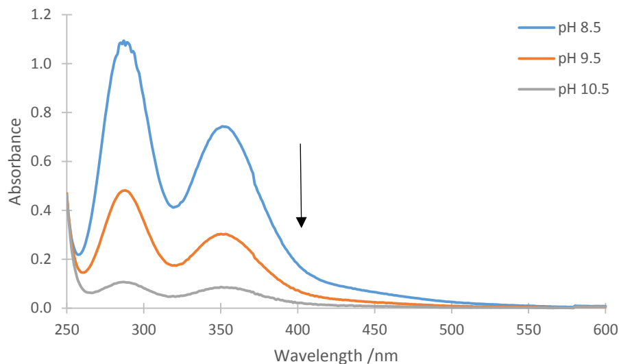
Figure 3.19 I_3^- absorbance as a function of pH, [PAA] = 25 \mu\text{M} , [KI] = 100 \mu\text{M} .
