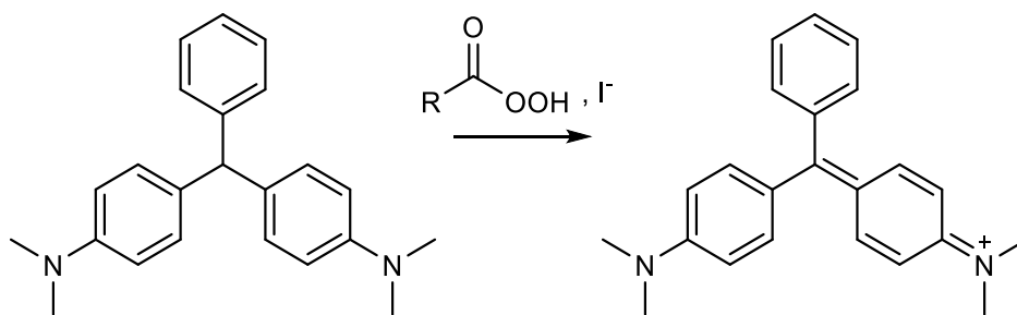
Figure 3.20 Reaction of LMG and PAA in presence of I^- results in generation of malachite green.
