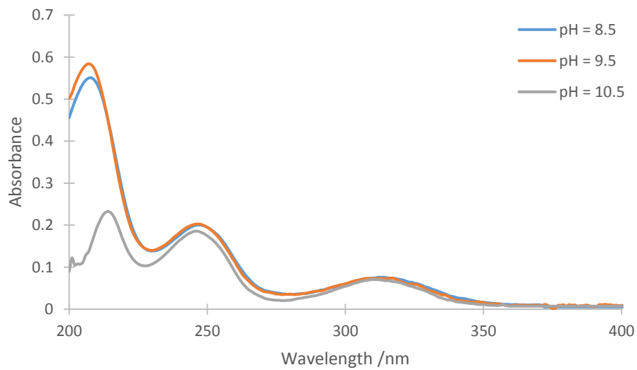
Appendix 1 HTA absorbance as a function of pH, [HTA] = 25 \mu M.
