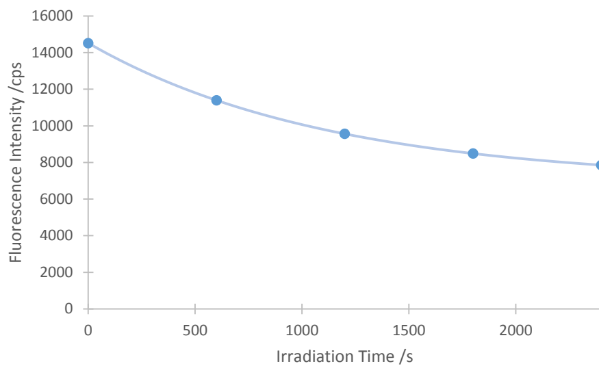
Figure 3.14 ADMA bleaching by singlet oxygen kinetic plot in pH 10.5, [ADMA] = 25 \mu M, [RB] = 50 \mu M, \lambda_{\text{ex}} = 340 nm, \lambda_{\text{em}} = 430 nm.
