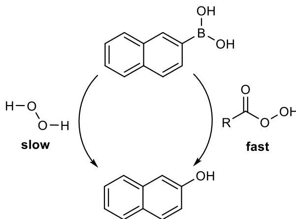
Figure 3.24 Concept behind assay for peroxides detection.
