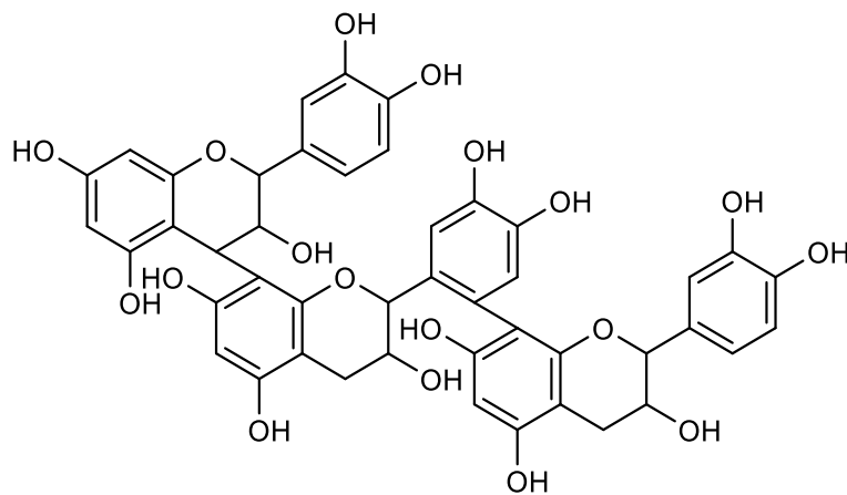
Figure 6.2 Example of polymerised catechin.
