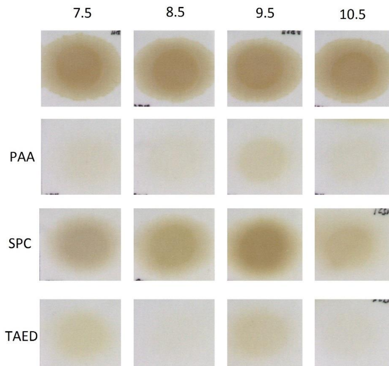
Figure 6.5 2 SRI, WN and ST parameters obtained for tea stains after bleaching PAA, SPC, TAED oxidants and in alkaline pH range over 45 min, [PAA] = 0.01 M, [SPC] = 0.01 M, [TAED + SPC] = 0.01 M + 0.03 M.
