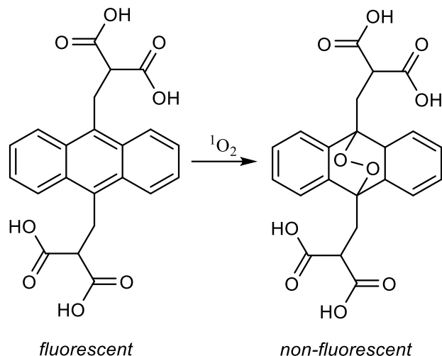
Figure 3.12 Reaction of ADMA and singlet oxygen results in a non-fluorescent endoperoxide.
