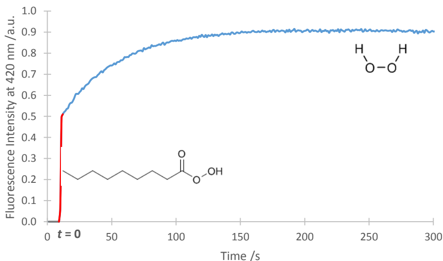
Figure 4.7 Fluorescence of NOH obtained after mixing NOBS, SPC and NBA, recorder at 420 nm as a function of time ( \lambda_{\text{ex}} = 340 \text{ nm} , \lambda_{\text{em}} = 420 \text{ nm} ) in pH 10.5. The rapid rise (red) is attributed to the presence of formed NPA, and slow rise (blue) to the presence of hydrogen peroxide.
