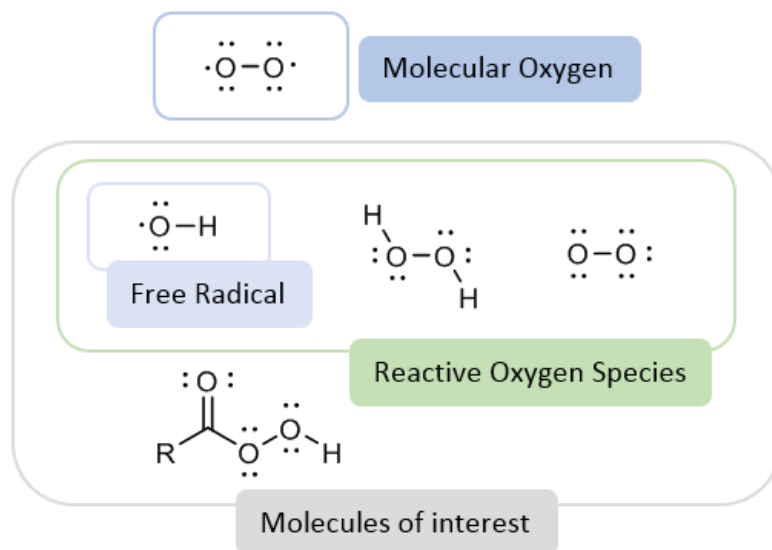
Figure 1.18 Lewis structures of ROS.
