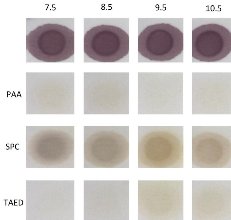
Figure 6.6 SRI, WN and ST parameters obtained for red wine stains after bleaching with PAA, SPC and TAED in alkaline pH range over 45 min, [PAA] = 0.01 \text{ M} , [SPC] = 0.01 \text{ M} , [TAED + SPC] = 0.01 \text{ M} + 0.03 \text{ M} .
