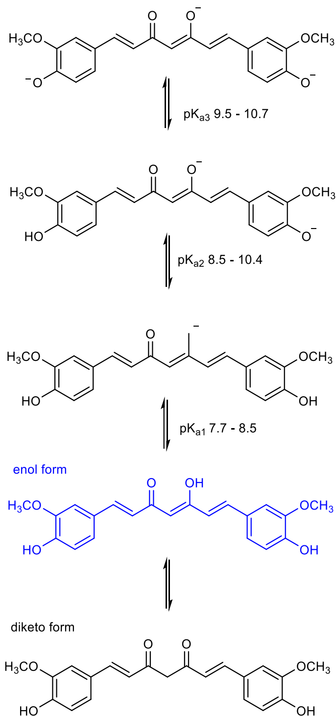
Figure 5.3 Keto-enol tautomerism and prototropic equilibria of curcumin; \text{pK}_{a1} 7.7 to 8.5, \text{pK}_{a2} 8.5 to 10.4, \text{pK}_{a3} 9.5 to 10.7. 7
