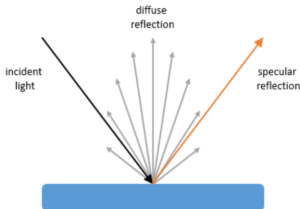
Figure 2.4 Diffuse and specular reflection from a glossy surface.
