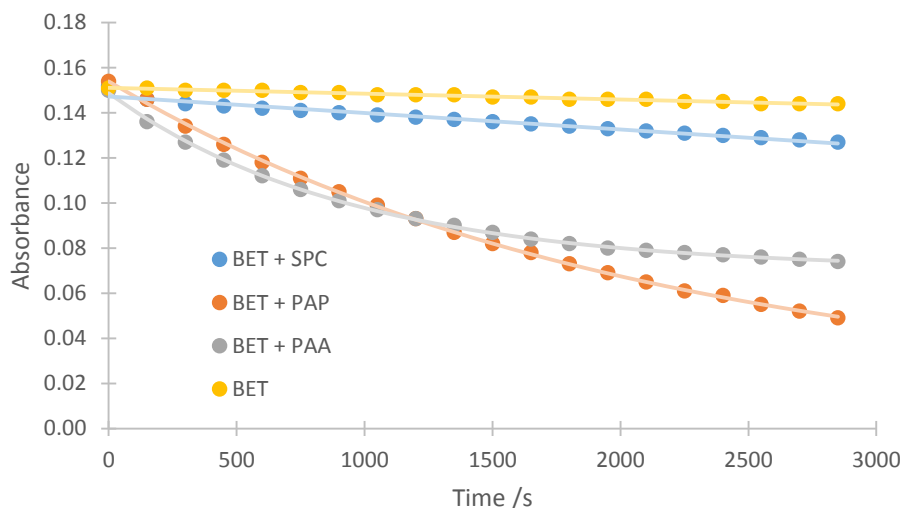
Figure 5.22 Absorbance of the BET at 550 nm and also in presence of agents, PAP and PAA over 45 min in pH 10.5, [BET] = 25 \mu M, [SPC, PAP, PAA] = 250 \mu M.
