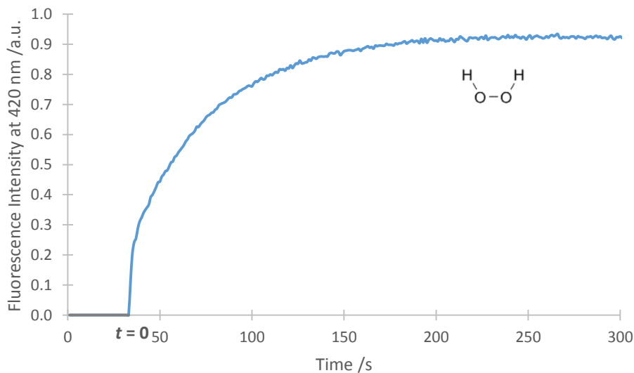
Figure 4.1 Fluorescence of NOH obtained after mixing SPC and NBA at 420 nm as a function of time ( \lambda_{\text{ex}} = 340 \text{ nm} ) at pH 10.5, [SPC] = 50 \mu\text{M} , [NBA] = 250 \mu\text{M} , \lambda_{\text{ex}} = 340 \text{ nm} , \lambda_{\text{em}} = 420 \text{ nm} .
