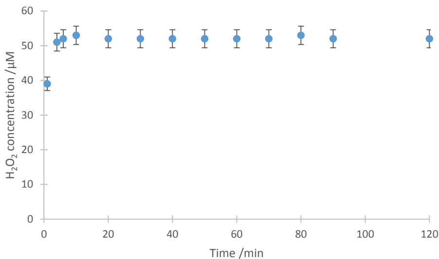
Figure 4.2 Iodometric titration of a 50 µM SPC sample over 2 hours. H 2 O 2 is rapidly released from SPC and then stable in alkaline environment (pH 10.5).
