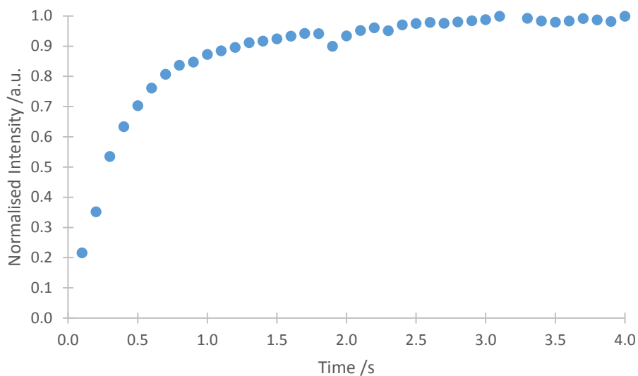
Figure 3.28 Fluorescence at 420 nm recorded using stopped flow during the reaction of NBA and PAA, pH 10.5, [NBA] = 50 \mu M, [PAA] = 20 \mu M, \lambda_{\text{ex}} = 340 nm, \lambda_{\text{em}} = 420 nm.
