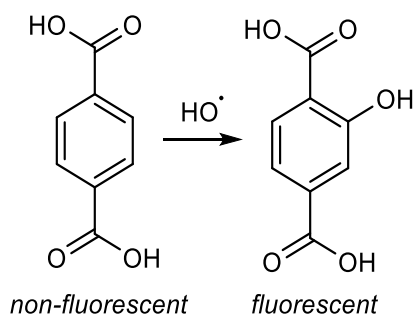
Figure 1.20 Reaction of TA and hydroxyl radical.
