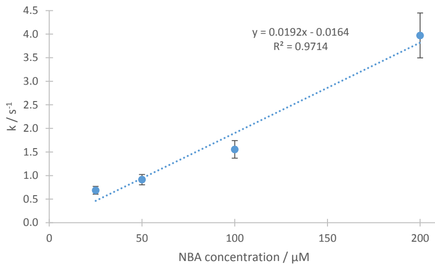
Figure 3.30 Linear plot of rate constant as a function of NBA concentration , while [\text{PAA}] = 50 \mu\text{M} , pH 10.5.
