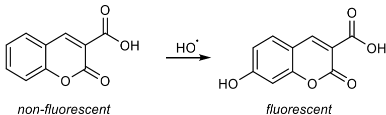
Figure 1.21 Reaction of CCA with hydroxyl radical.
