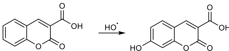
Figure 3.6 Reaction of coumarin-3-carboxylic acid (CCA) and hydroxyl radical which yields to 7-hydroxy-coumarin-3-carboxylic acid (7-OH-CCA).
