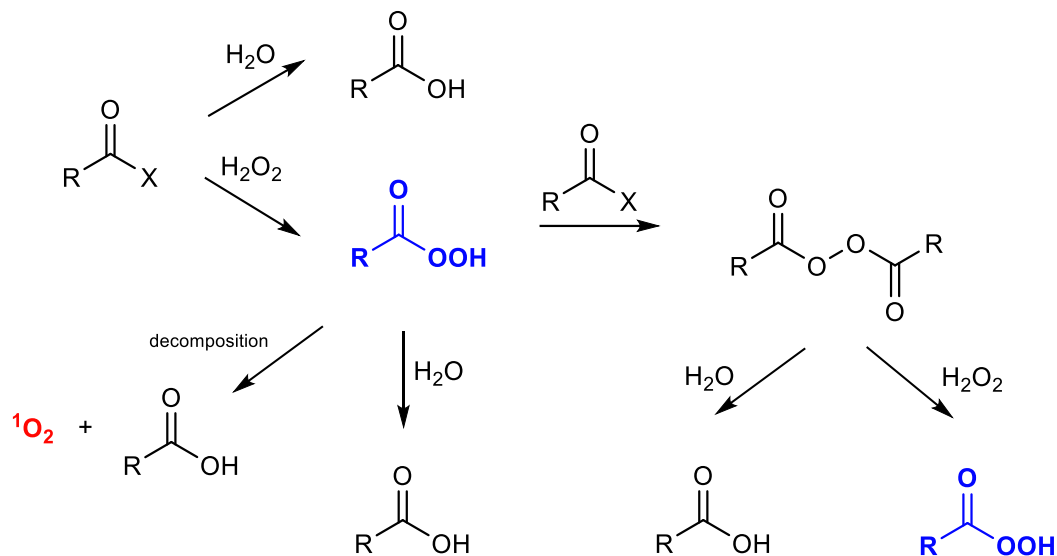
Figure 1.9 Routes of peroxyacid decompositions.
