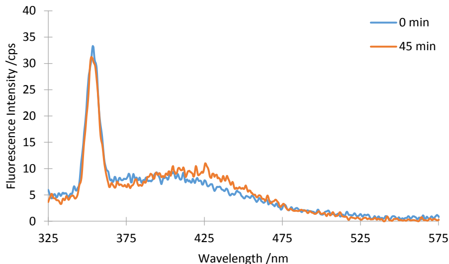
Figure 4.12 Raman scattering of water peak, obtained from mixture of PAA and TA in pH 10.5, [TA] = 100 \mu M, [PAA] = 500 \mu M, \lambda_{\text{ex}} = 315 nm.
