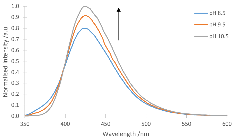
Figure 3.2 Generation of hydroxyl radicals with irradiation of \text{KNO}_3 as a function of pH. [\text{KNO}_3] = 1 \text{ mM} , [\text{TA}] = 250 \mu\text{M} , \lambda_{\text{ex}} = 340 \text{ nm} .
