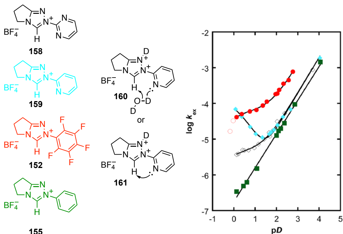
Figure 4: pD – \log k_{\text{ex}} profile for N-pyridinyl and N-pyrimidinyl substituents, with the profile for N-Ph and N-C 6 F 5 shown for comparison. 58,59 (Reproduced with permission of Wiley publications. Copyright © 2014 John Wiley & Sons, Ltd)
