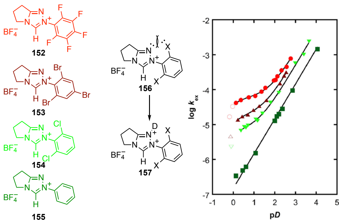
Figure 3: pD - \log k_{ex} profile for a range of ortho -halogenated N-aryl substituents, with the profile for N-Ph shown for comparison. 58,59 (Reproduced with permission of Wiley publications. Copyright © 2014 John Wiley & Sons, Ltd)
