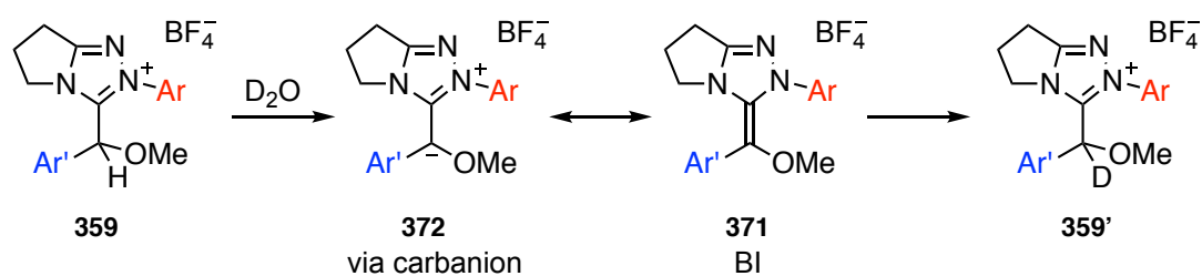
Scheme 64: C(α)-H/D is evidence of carbanion formation at C(α), which may delocalise to form the O-methylated BI 371.
