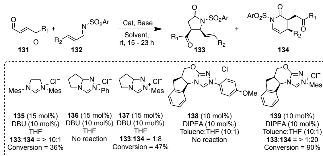
Scheme 23: Triazolylidene-catalysed azadiene Diels-Alder reaction which, goes via enolate intermediate. 46
