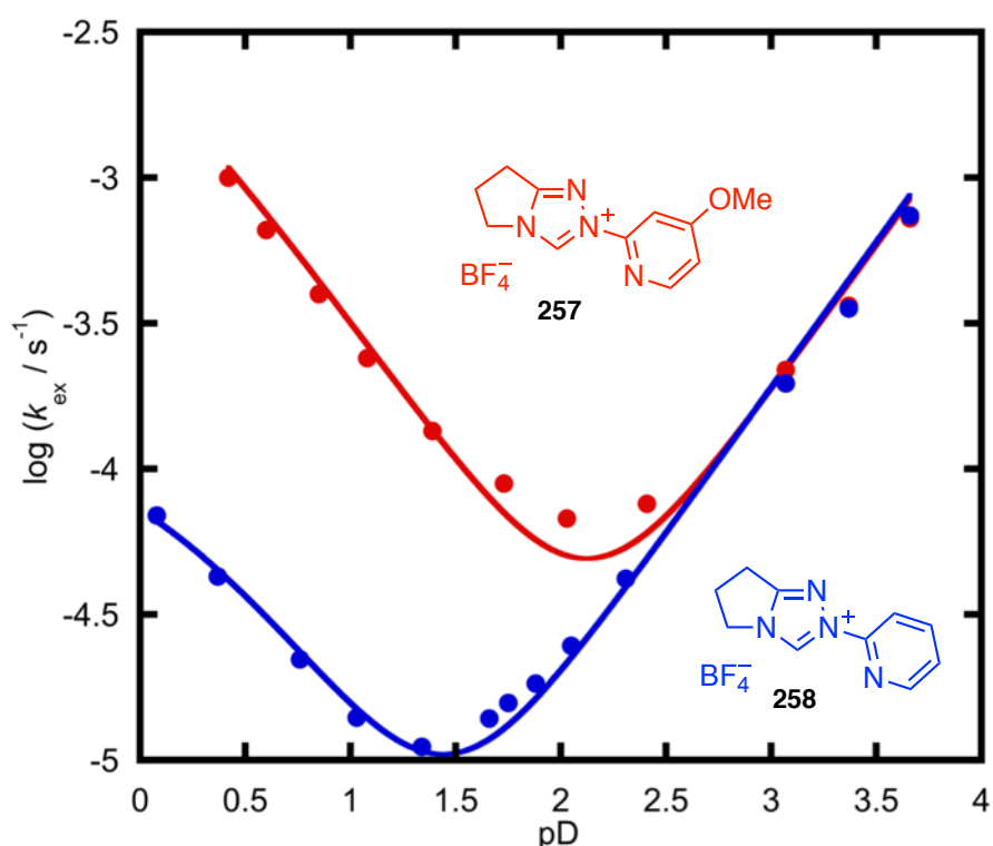
Figure 18: pD – \log k_{ex} profile for C(3)-H/D exchange for N-5-methoxypyrid-2-yl 257 (●) and N-pyrid-2-yl 258 (●) triazolium salts, which includes a substrate ionisation term ( K_a^{N1} , leading to the onset of a downward bend at pD ~ 0) but excludes a pD-independent term (in between the slopes of -1 and +1). The points are experimental, the solid curve calculated using Eqn. (4).
